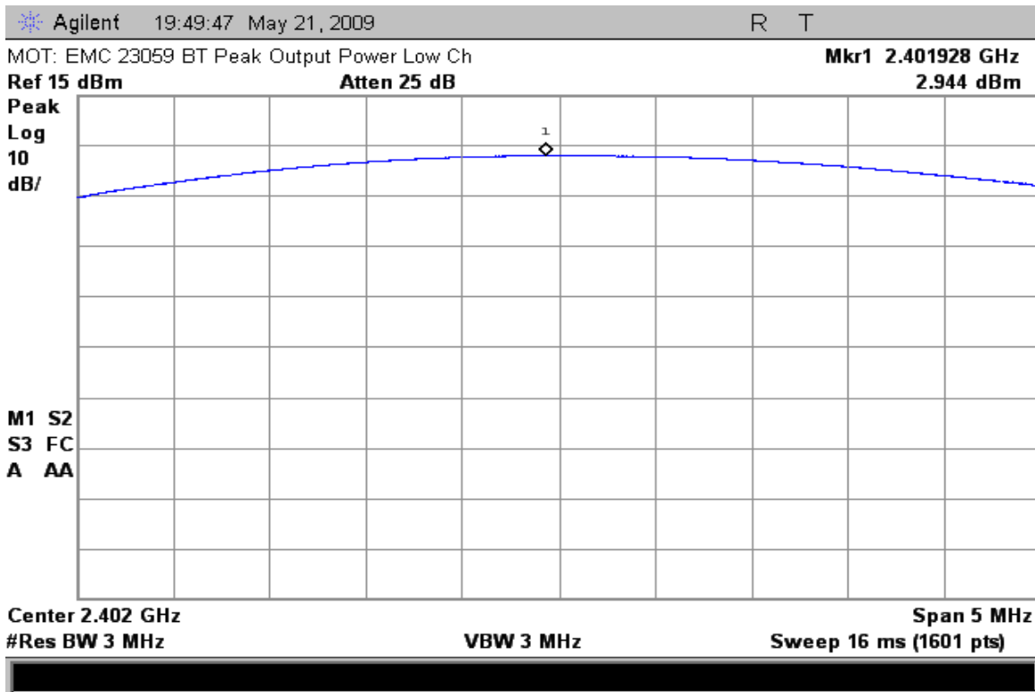
Low Channel Peak Output Power with EDR Disabled
