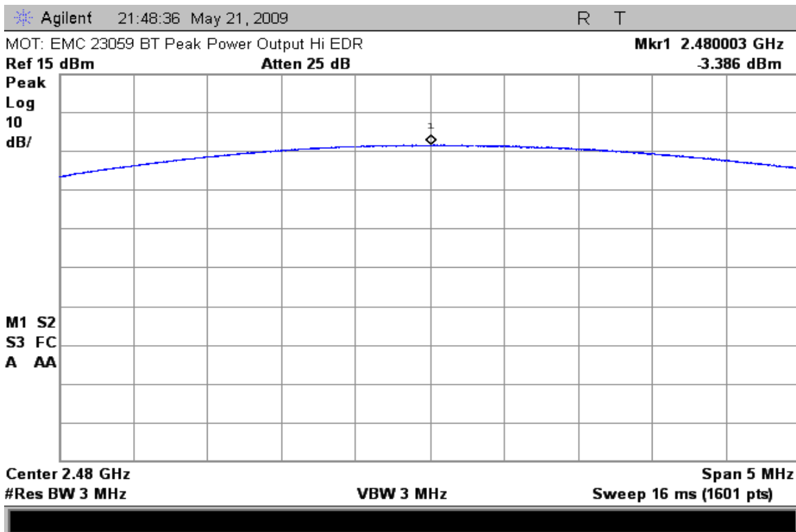
High Channel Peak Output Power with EDR Enabled
