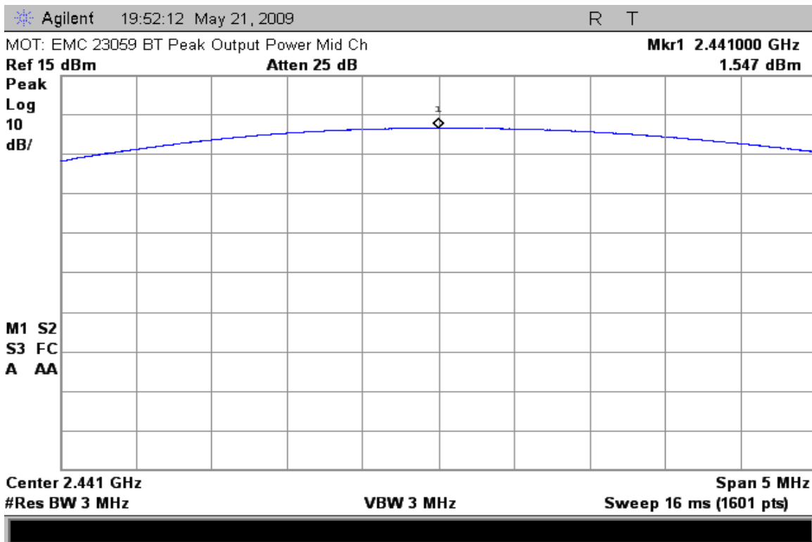
Mid Channel Peak Output Power with EDR Disabled
