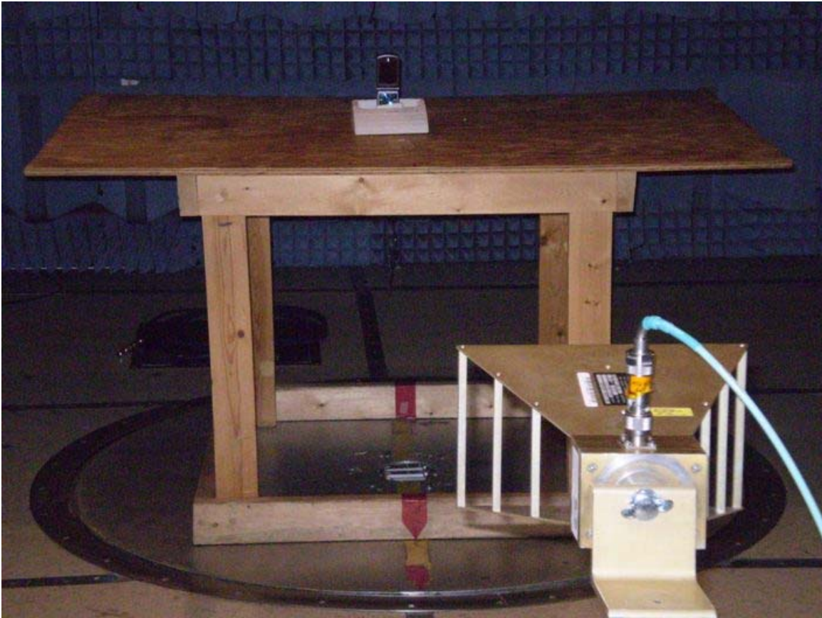
EMC Report #23059 Tx Radiated
