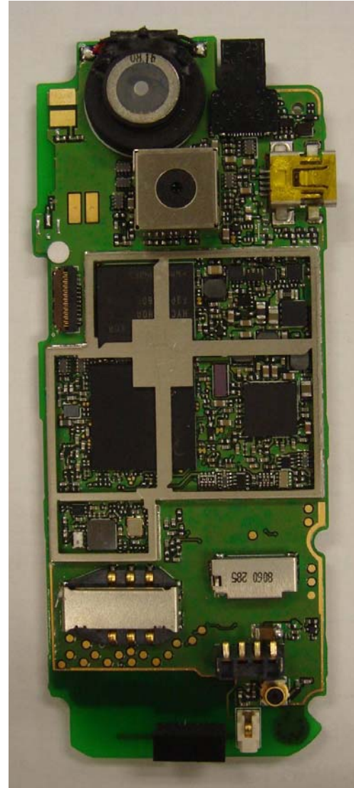
Rear View (Shields Removed)
