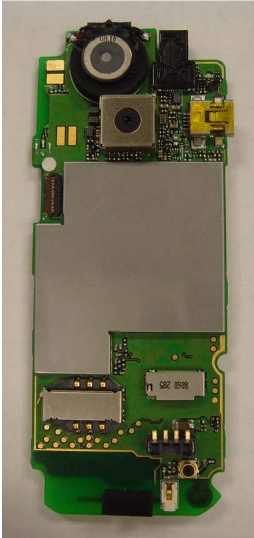
Rear View with Shields
