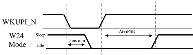
Figure 2-10: WKUPI_N Signal Operation
