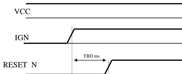
Figure 2-5: IGN Power On Timing
