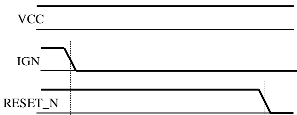
Figure 2-7: IGN Power Off Timing
