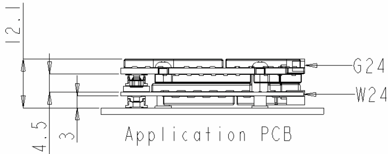
figure A-A
