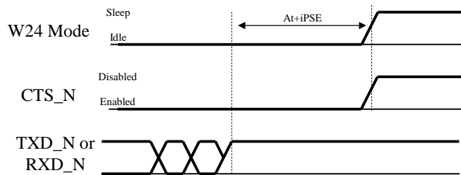
Figure 2-11: Serial Interface Data
