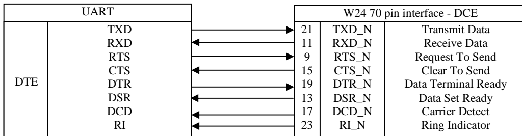
Figure 2-12:UART1 Interface Signals
