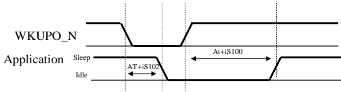
Figure 2-11: WKUPO_N Signal Operation
