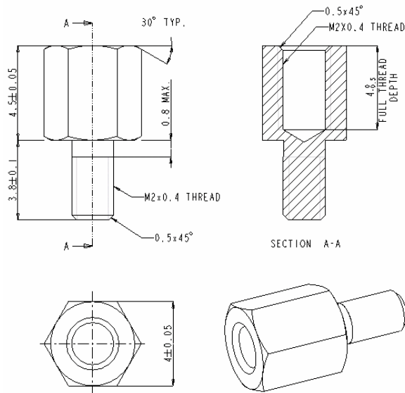
figure B-B
