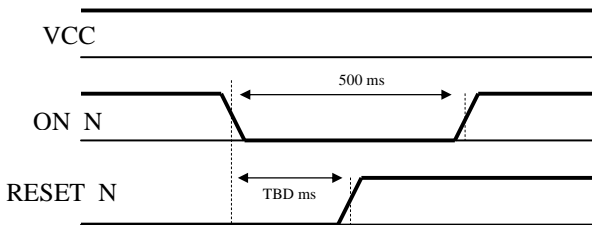
Figure 2-4: ON_N Power On Timing
