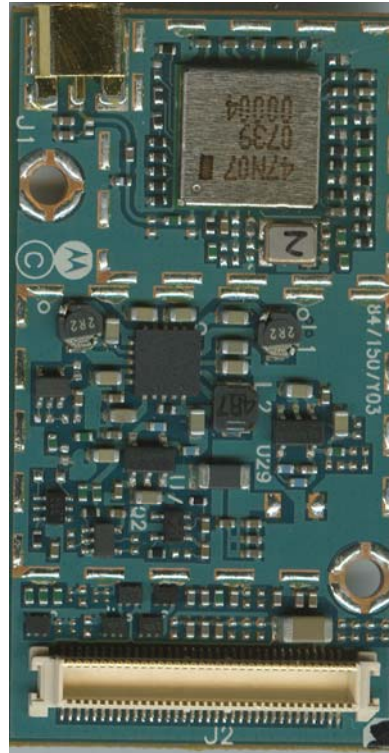
Rear View (Shields Removed)
