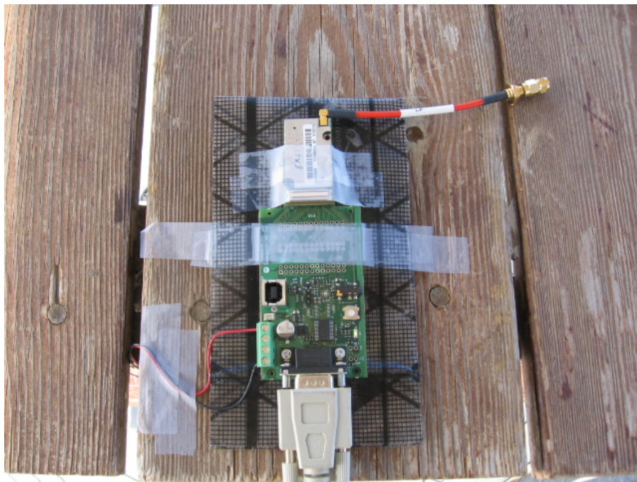
Figure 4. Radiated Emission Test Close-up
