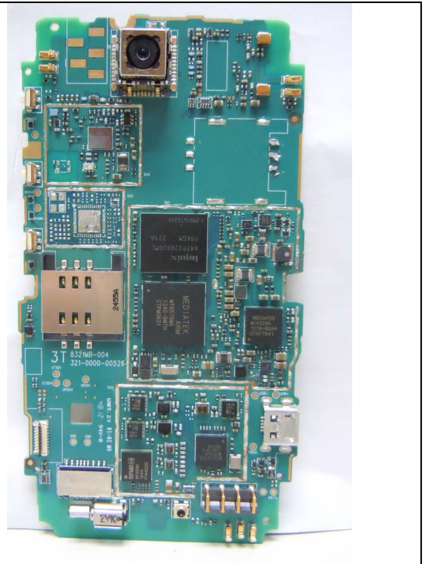
Photograph 9-2: Single SIM Variant PC Board.
