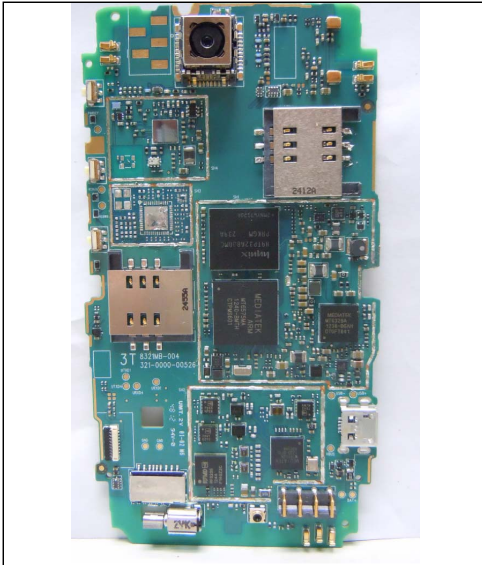
Photograph 9-1: Dual SIM Variant PC Board.
