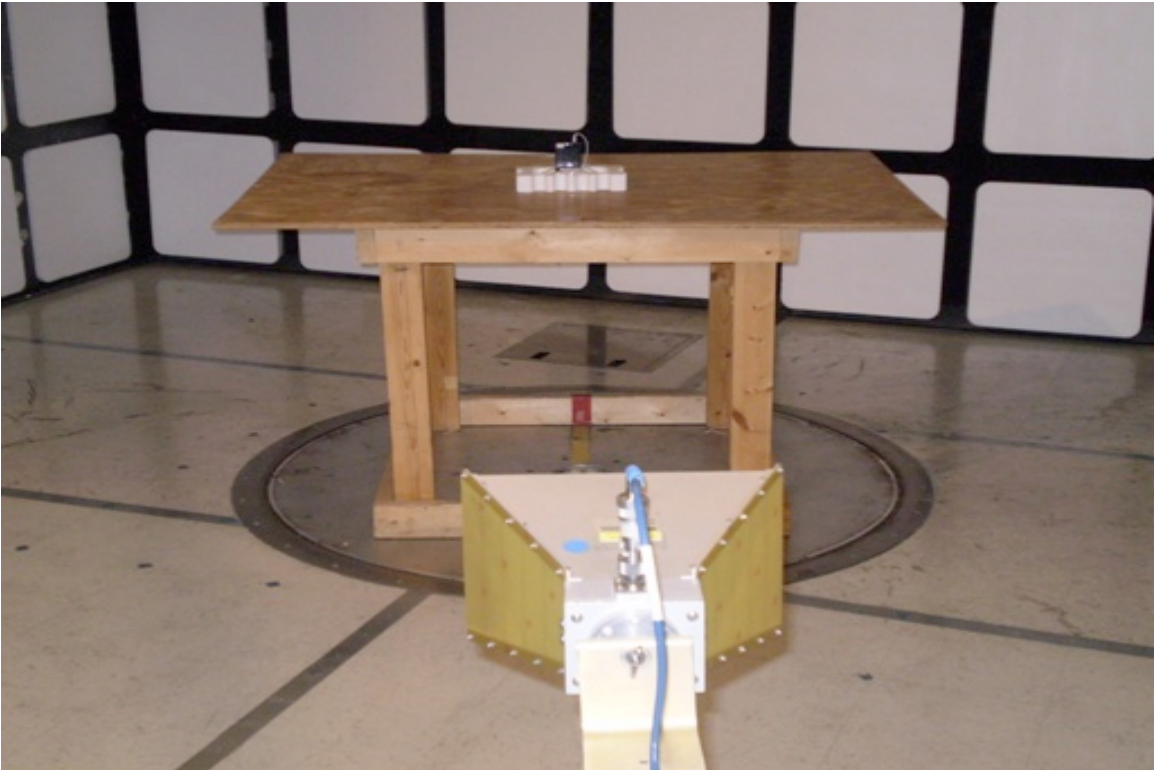
Tx Radiated
