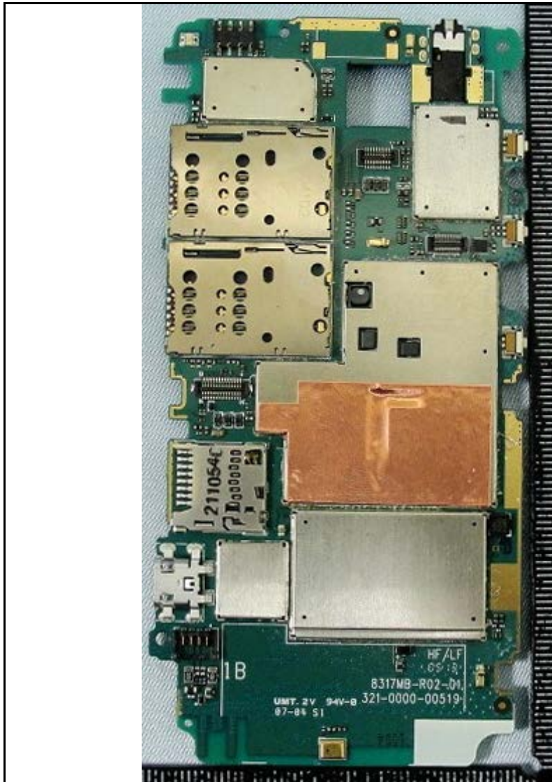
Photograph 9-1: Dual SIM Variant PC Board.
