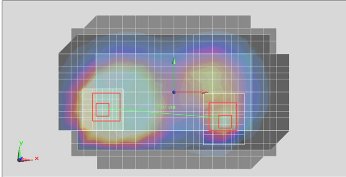
WCDMA 1900 Back of Phone 10mm from Phantom SAR overlaid with Wi-Fi 2.4 GHz Back of Phone 10mm from Phantom SAR
