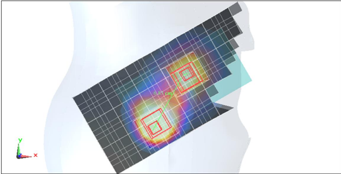
WCDMA 850 Right Head Cheek SAR overlaid with Wi-Fi 2.4 GHz Right Head Cheek SAR
