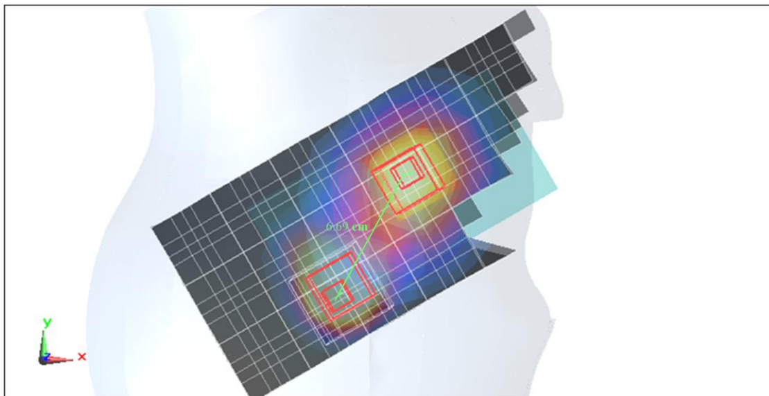
GSM 850 Right Head Cheek SAR overlaid with Wi-Fi 2.4 GHz Right Head Cheek SAR
