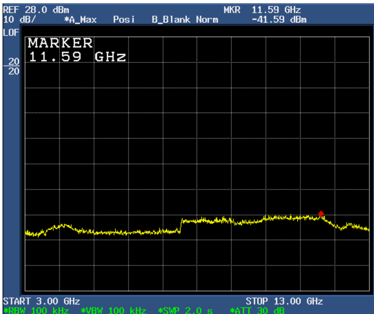
Figure 6d.8-8: Plot of spurious conducted emissions 3 GHz – 13 GHz (High Channel Enabled).
