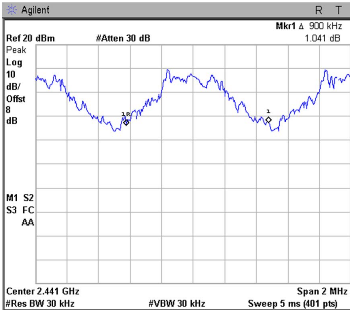
Figure 6d.2-1: Plot of 20 dB bandwidth (GFSK Modulation)
