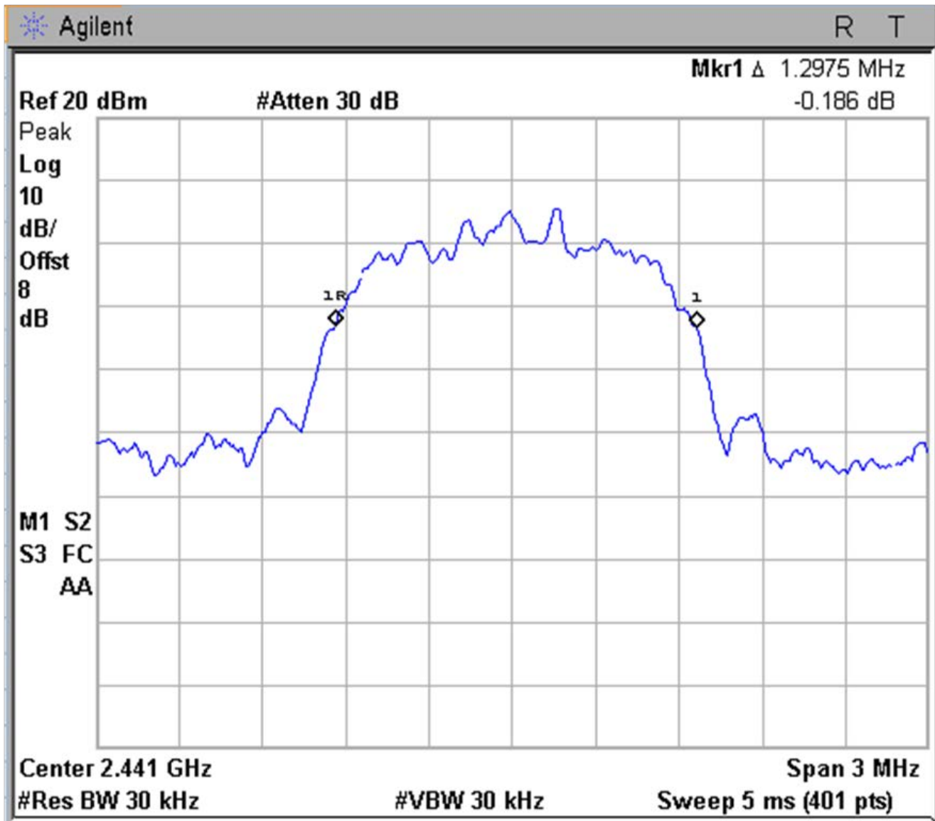
Figure 6d.2-2: Plot of 20 dB bandwidth (P/4 DPSK Modulation)
