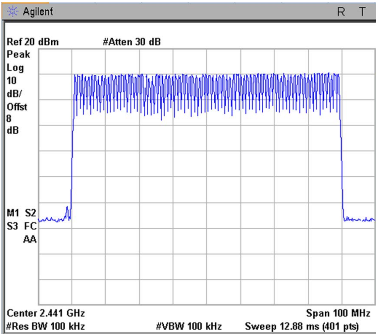
Figure 6d.3-1: Plot of number of Bluetooth hopping frequencies
