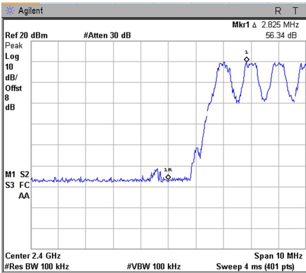
Figure 6d.6-3: Plot of lower band-edge conducted emissions with hopping enabled (GFSK Modulation).
