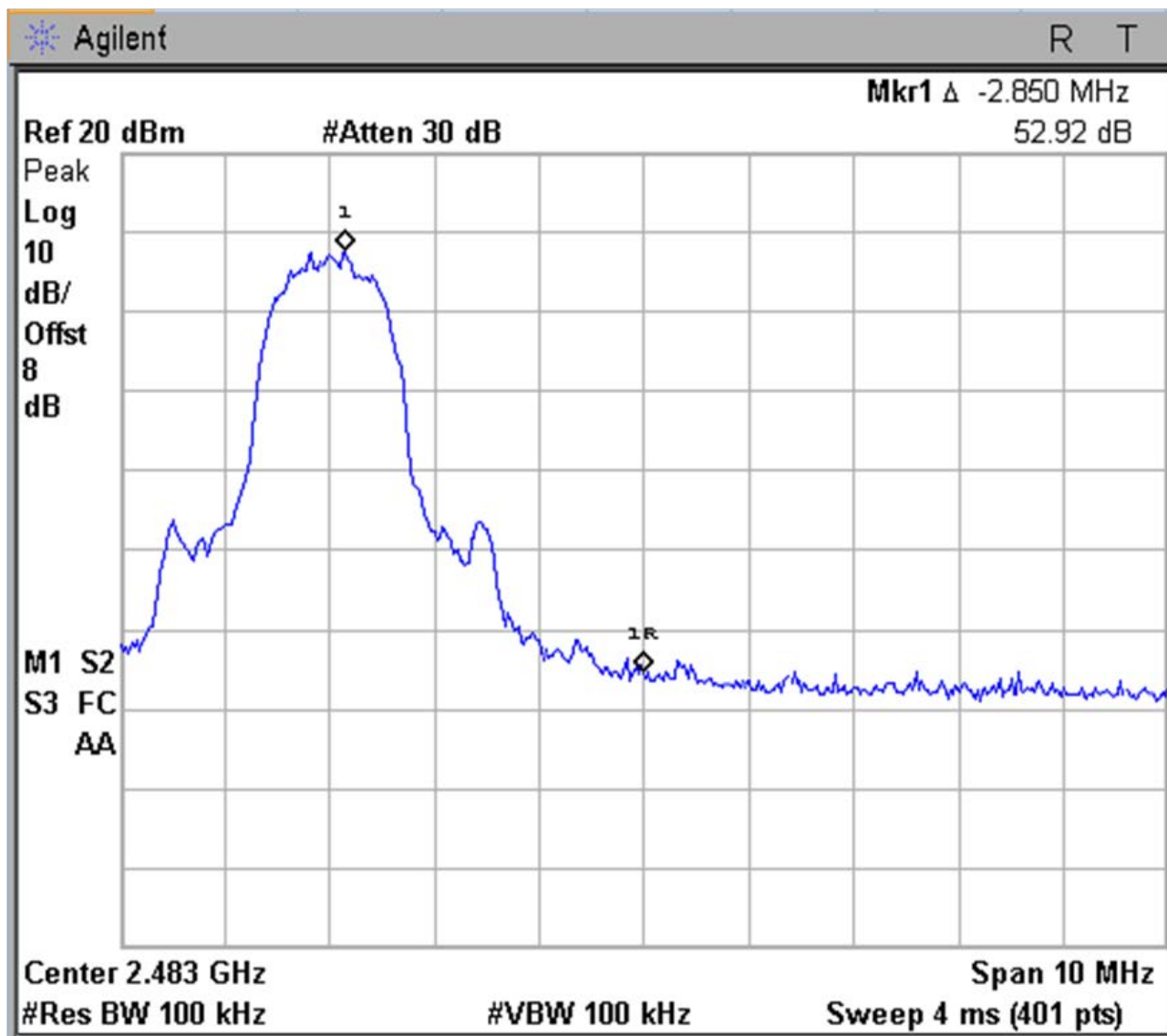
Figure 6d.6-10: Plot of upper band-edge conducted emissions with hopping disabled (8 DPSK Modulation).
