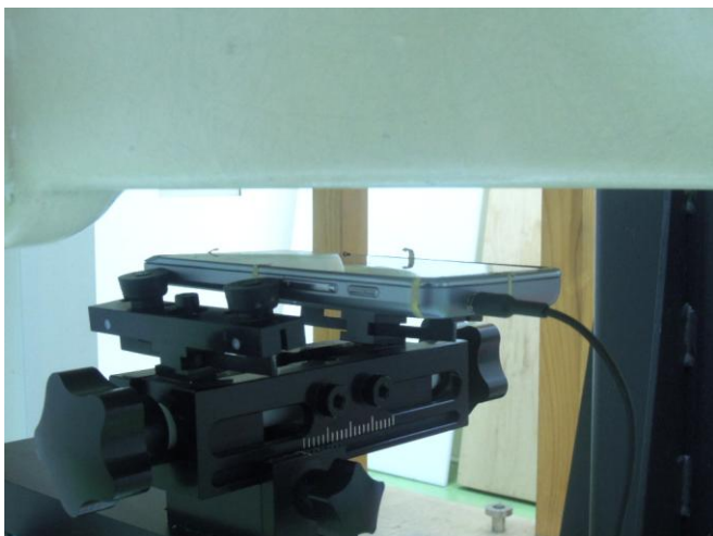
Front Face of EUT with 2.5 cm Gap (Body-Worn Mode)
