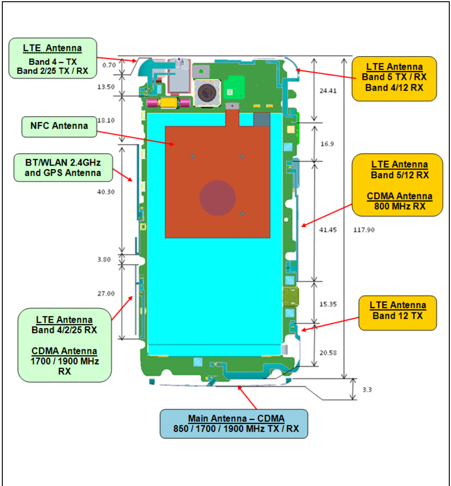
Photograph 9-8: Antenna Dimensions and Spacing (Back Side View).
