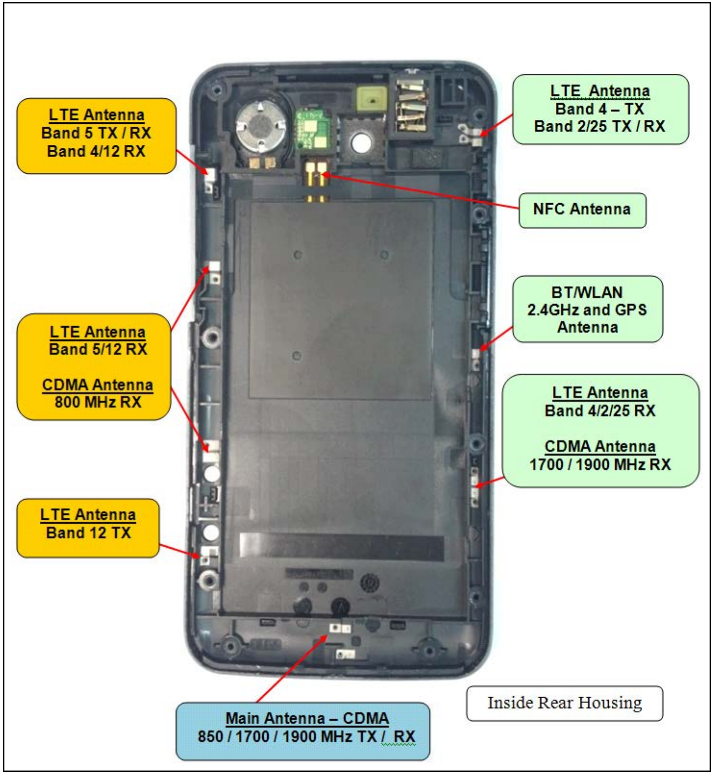
Photograph 9-6: Antenna Locations inside Rear Housing (Front Side View).
