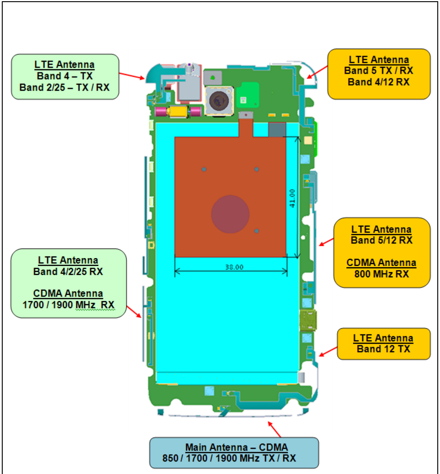
Photograph 9-7: Antenna Representations, Licensed Services Only (Back Side View)
