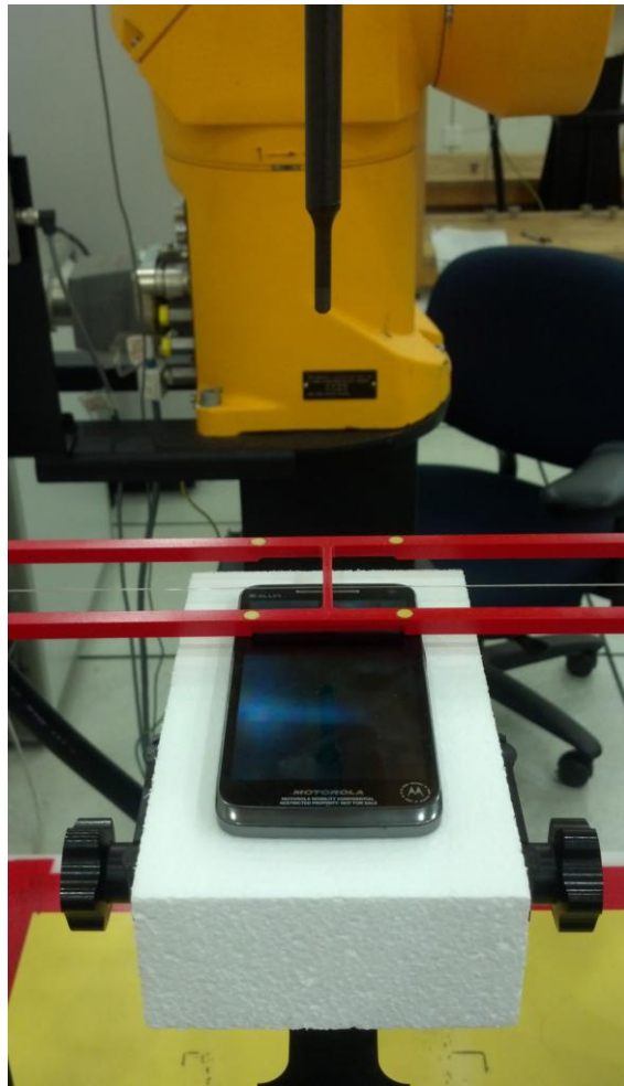
Figure 4. Positioning and Measurement for RF Emissions
