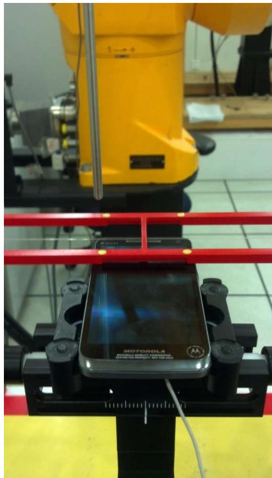
Figure 7. Positioning and Measurement for T-coil
