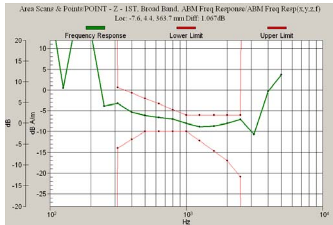
Figure 9-1-4: 900 MHz Measured Frequency Response (1:6).
