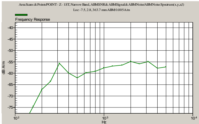
Figure 9-4-1: 900 MHz Undesired Signal (2:6).
