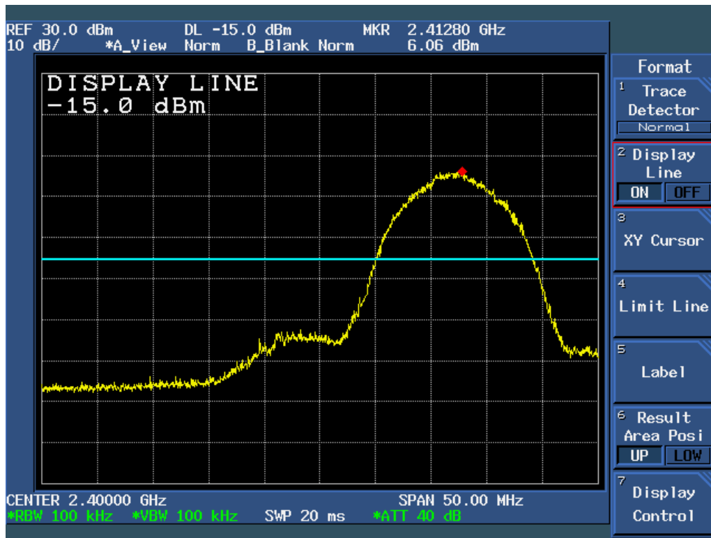
Figure 6c.6-1: Plot of Lower Band Edge Spurious Emission (11 Mbps data rate).
