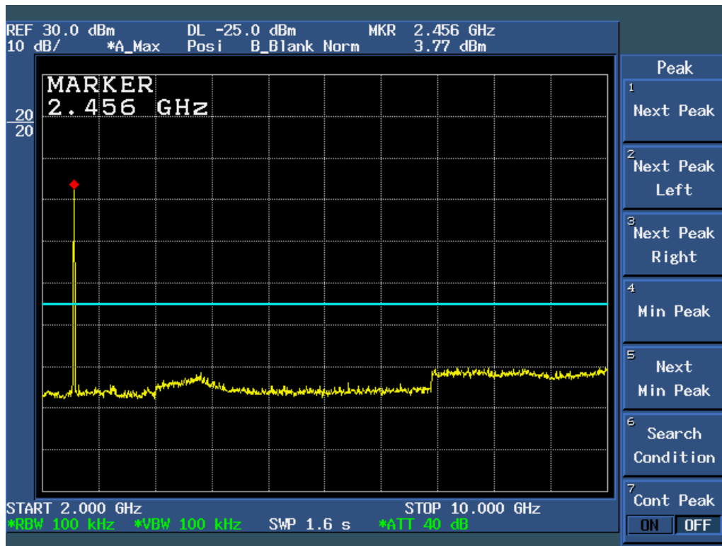
Figure 6c.5-10: Plot of Conducted Spurious Emissions, 2 – 10 GHz (11 Mbps data rate, Ch 11).
