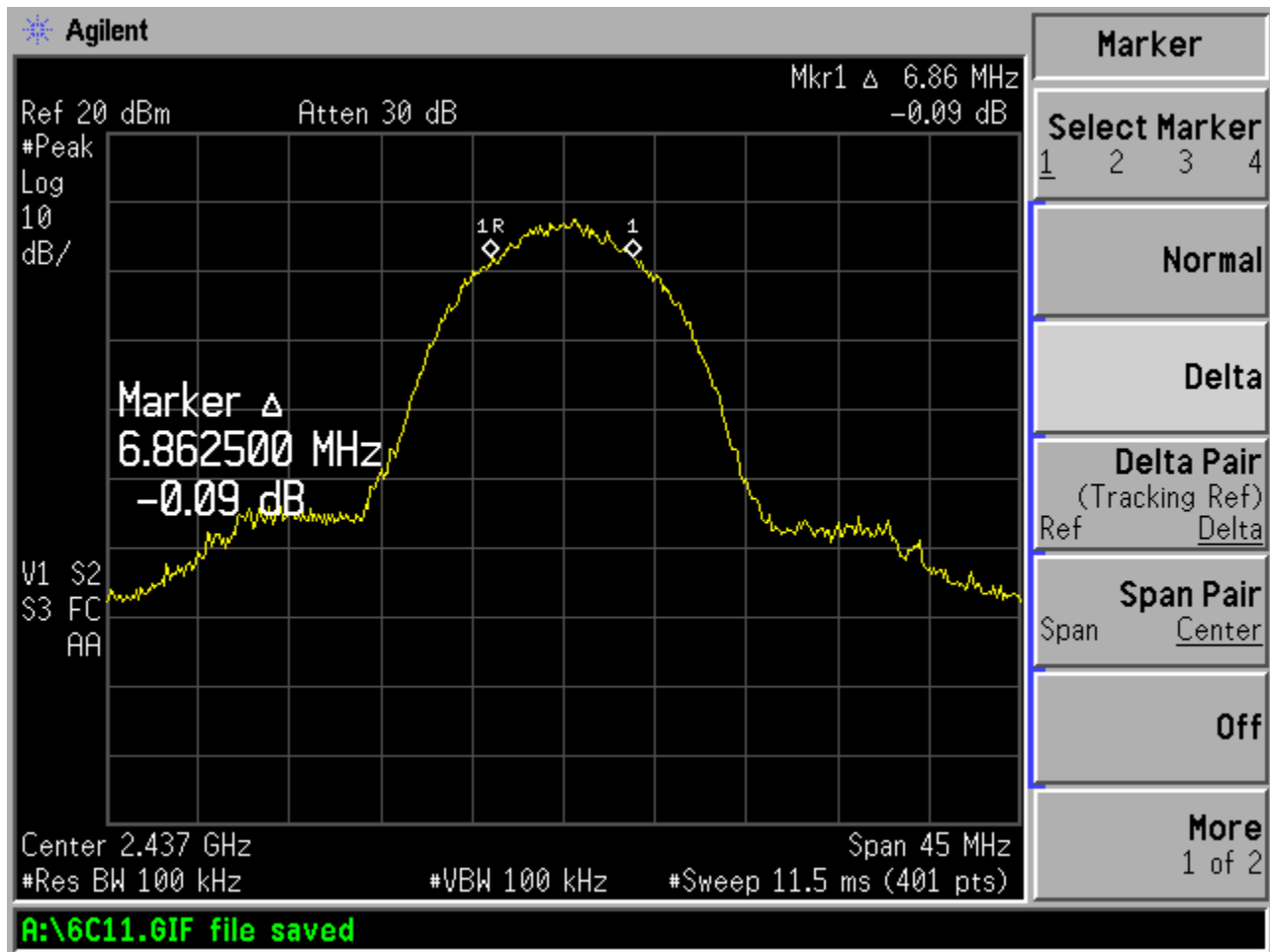
Figure 6c.1-2: Plot of 6 dB bandwidth (Channel 6, 11 Mbps data rate)
