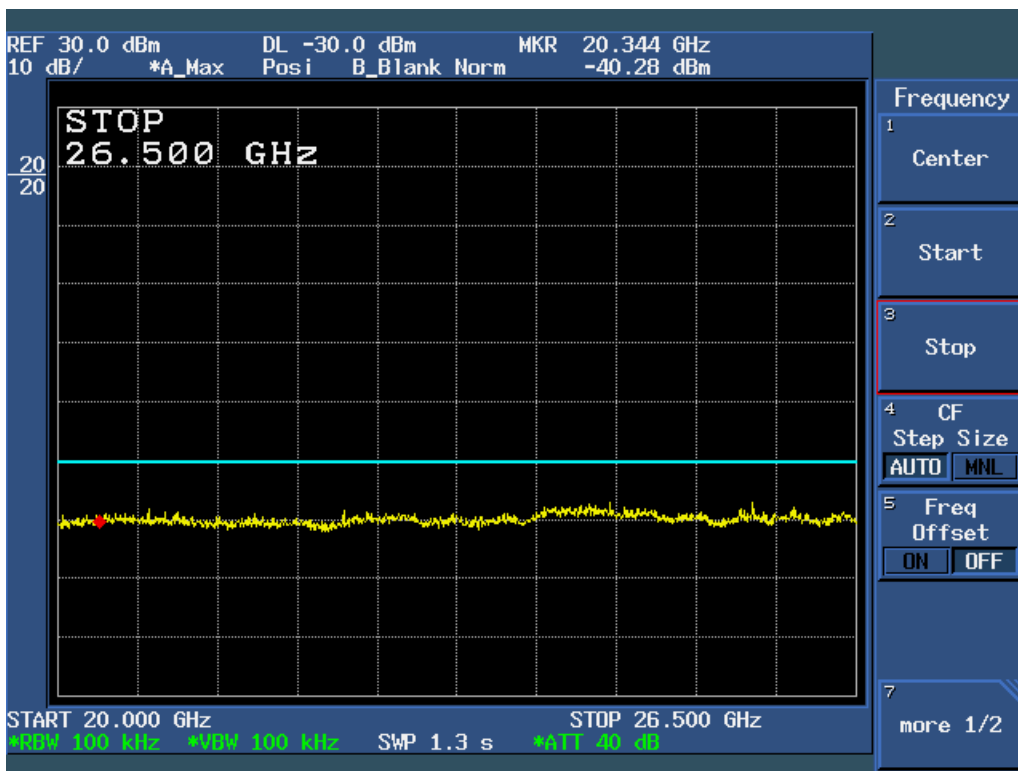
Figure 6c.5-20: Plot of Conducted Spurious Emissions, 20 – 26.5 GHz (54 Mbps data rate, Ch 6).
