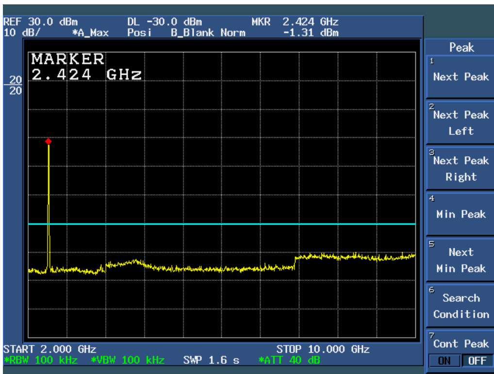
Figure 6c.5-18: Plot of Conducted Spurious Emissions, 2 – 10 GHz (54 Mbps data rate, Ch 6).
