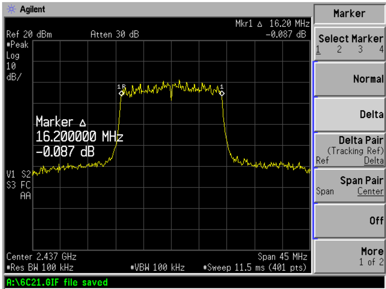
Figure 6c.2-2: Plot of 6 dB bandwidth (Channel 6, 54 Mbps data rate)
