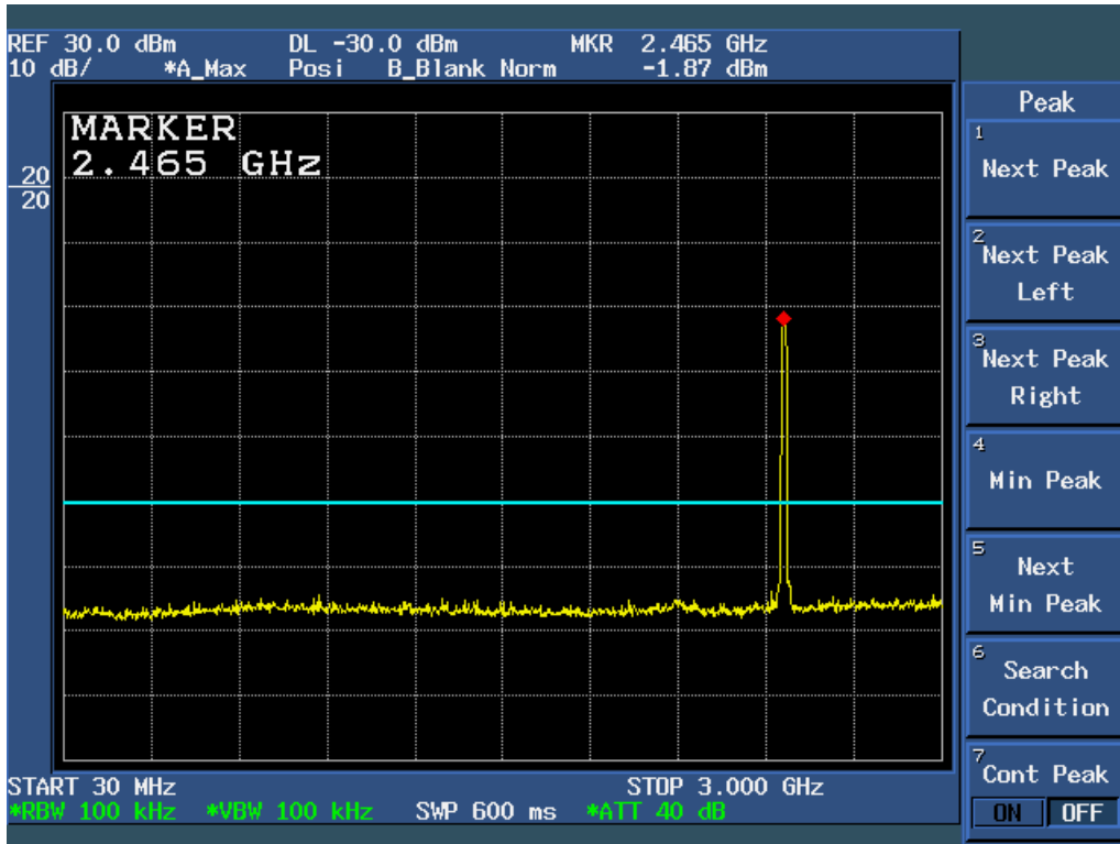
Figure 6c.5-21: Plot of Conducted Spurious Emissions, 30 – 3000 MHz (54 Mbps data rate, Ch 11).
