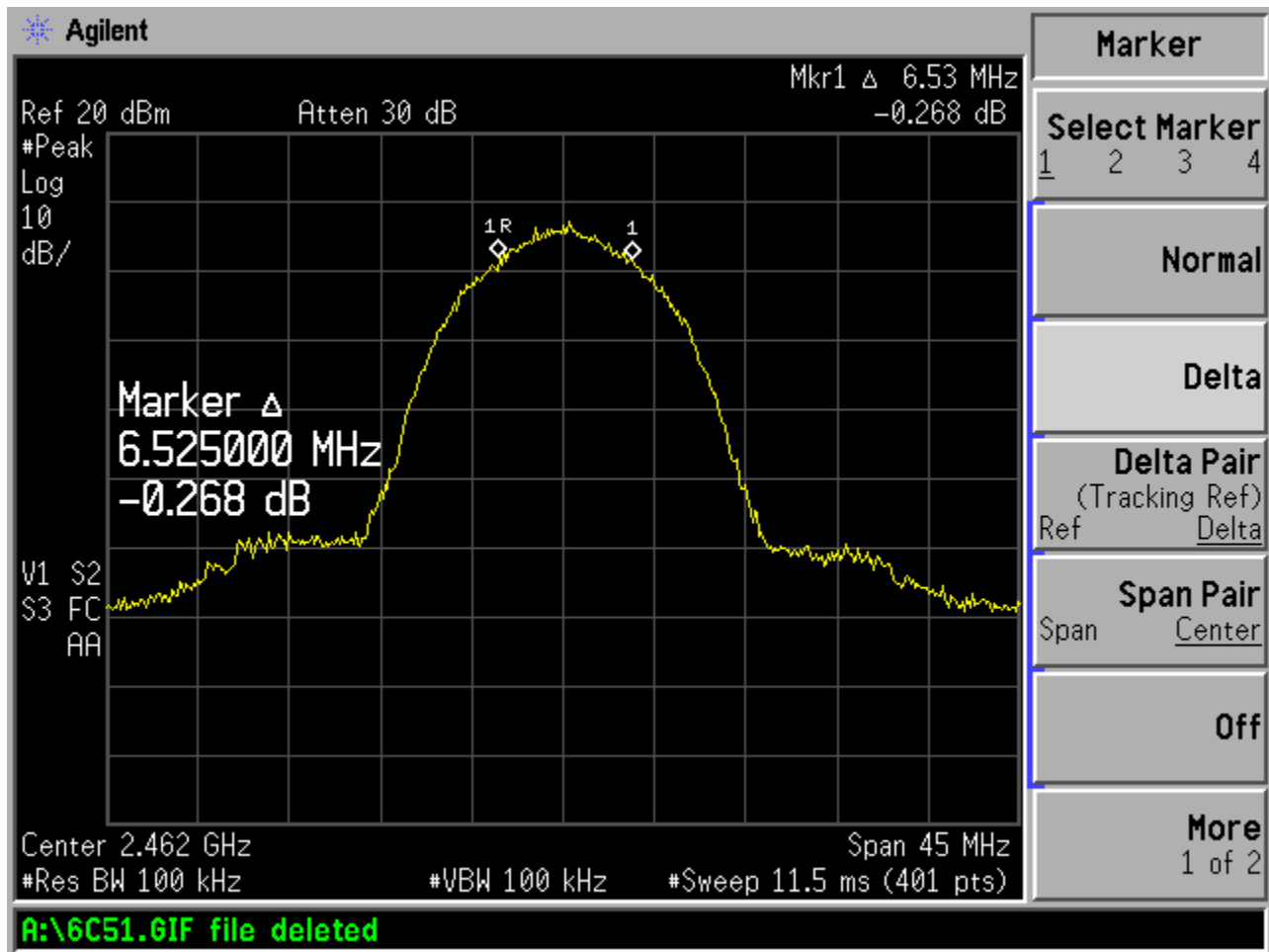
Figure 6c.1-3: Plot of 6 dB bandwidth (Channel 11, 11 Mbps data rate)
