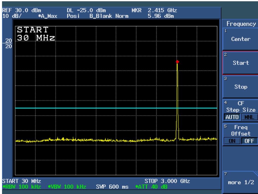
Figure 6c.5-1: Plot of Conducted Spurious Emissions, 30 – 3000 MHz (11 Mbps data rate, Ch 1).
