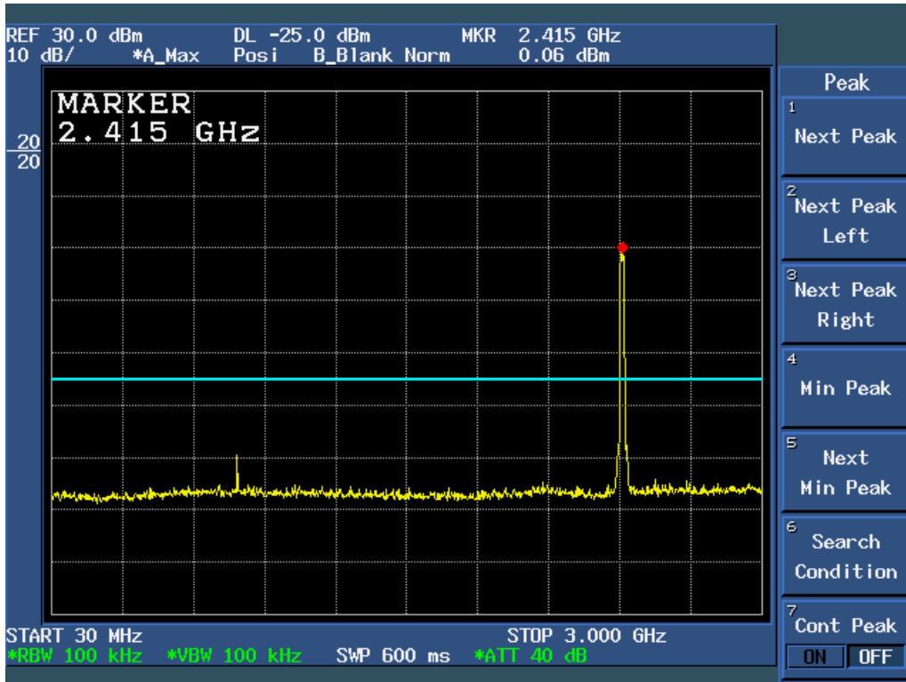
Figure 6c.5-13: Plot of Conducted Spurious Emissions, 30 – 3000 MHz (54 Mbps data rate, Ch 1).
