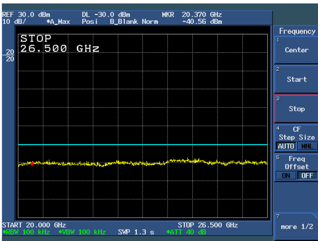
Figure 6c.5-24: Plot of Conducted Spurious Emissions, 20 – 26.5 GHz (54 Mbps data rate, Ch 11).
