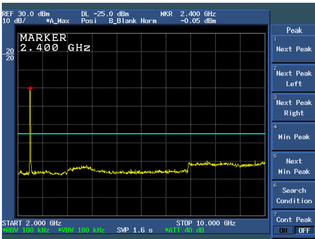
Figure 6c.5-14: Plot of Conducted Spurious Emissions, 2 – 10 GHz (54 Mbps data rate, Ch 1).
