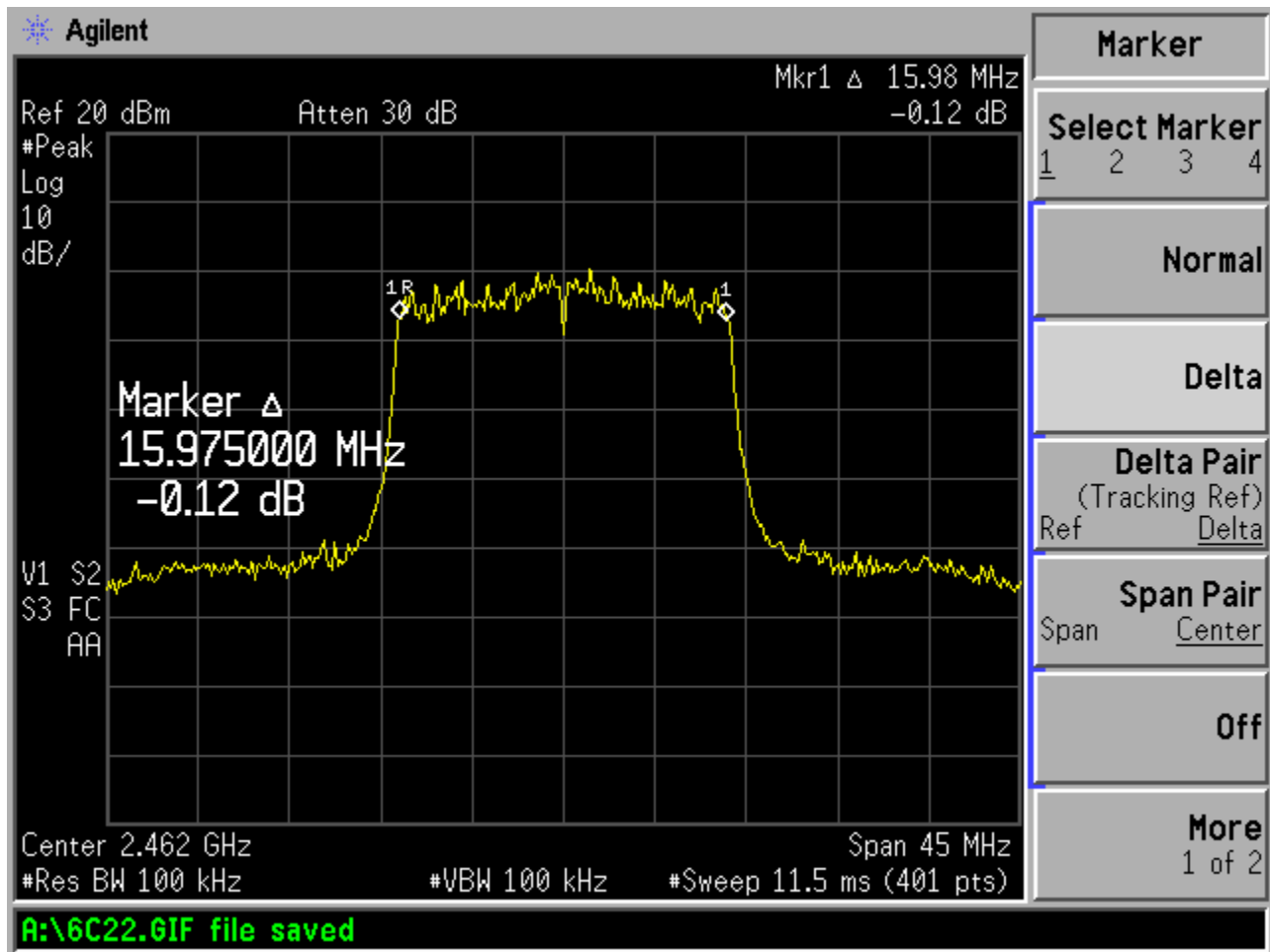
Figure 6c.2-3: Plot of 6 dB bandwidth (Channel 11, 54 Mbps data rate)
