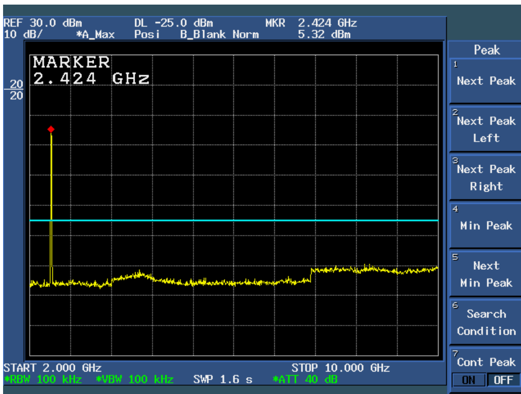
Figure 6c.5-6: Plot of Conducted Spurious Emissions, 2 – 10 GHz (11 Mbps data rate, Ch 6).
