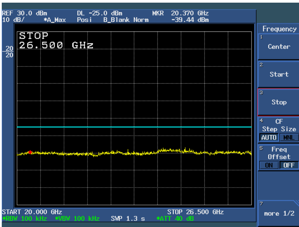
Figure 6c.5-12: Plot of Conducted Spurious Emissions, 20 – 26.5 GHz (5 Mbps data rate, Ch 11).
