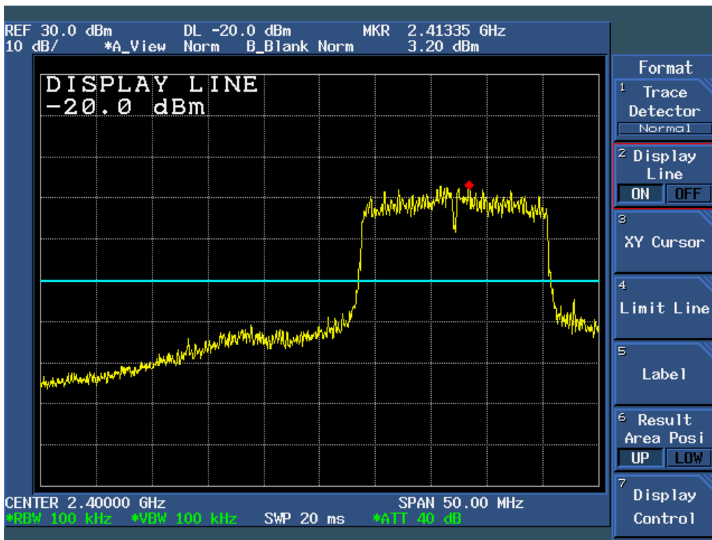
Figure 6c.6-31: Plot of Lower Band Edge Spurious Emission (54 Mbps data rate).
