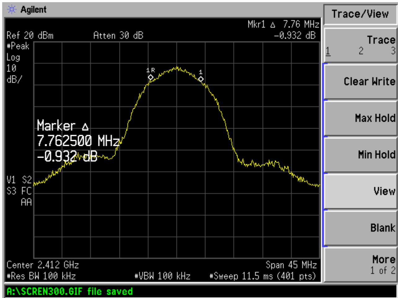
Figure 6c.1-1: Plot of 6 dB bandwidth (Channel 1, 11 Mbps data rate)
