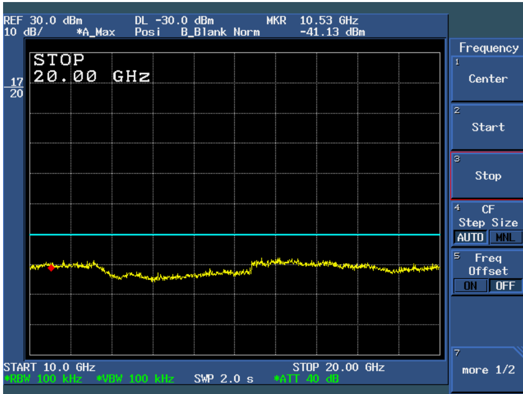
Figure 6c.5-19: Plot of Conducted Spurious Emissions, 10 – 20 GHz (54 Mbps data rate, Ch 6).
