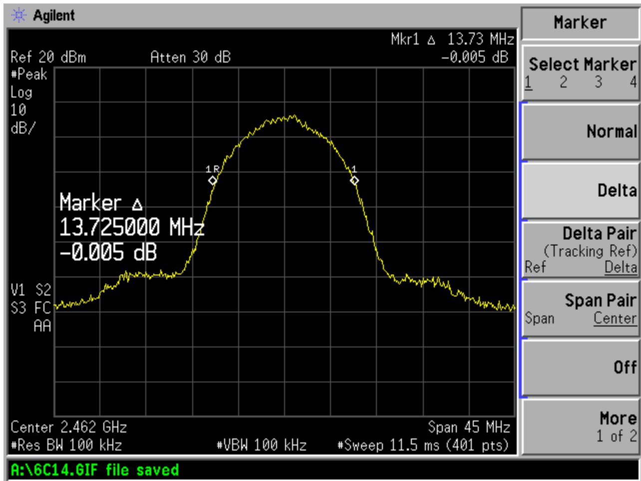
Figure 6c.1-6: Plot of 20 dB bandwidth (Channel 11, 11 Mbps data rate)
