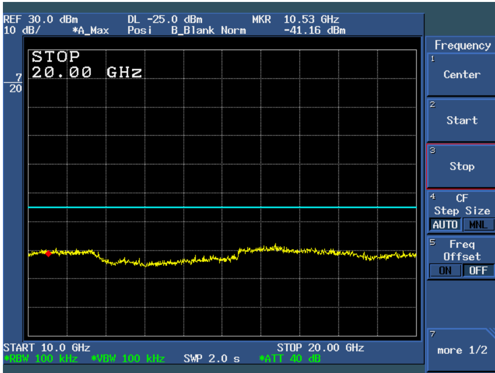
Figure 6c.5-7: Plot of Conducted Spurious Emissions, 10 – 20 GHz (11 Mbps data rate, Ch 6).
