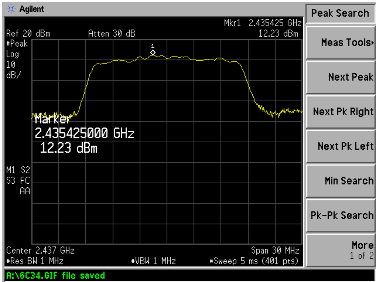
Figure 6c.3-5: Peak Output Power (Channel 6, 54 Mbps data rate)
