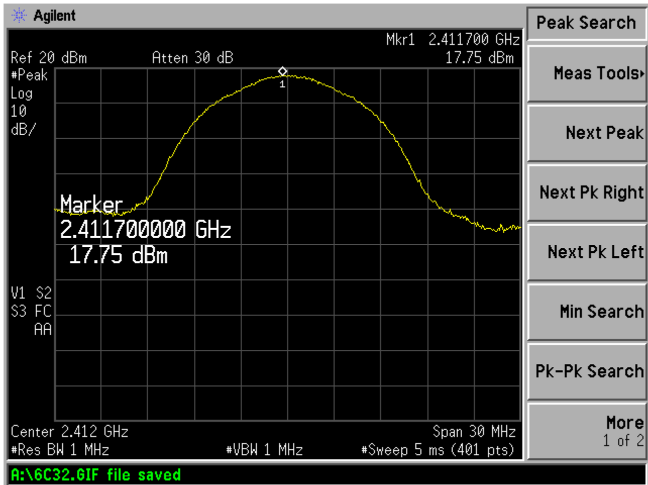
Figure 6c.3-1: Peak Output Power (Channel 1, 11 Mbps data rate)
