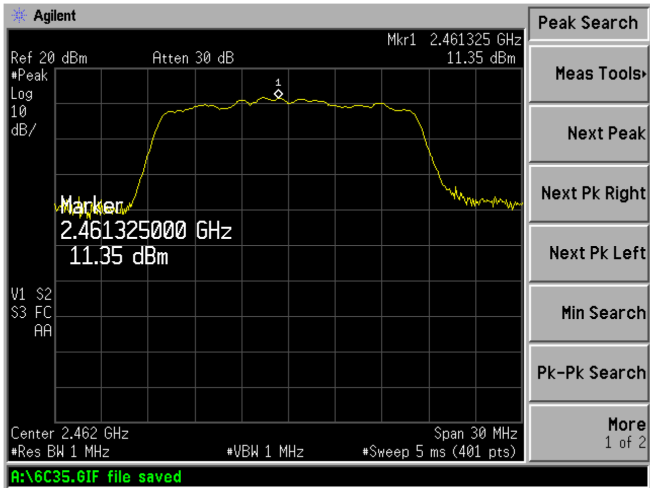
Figure 6c.3-6: Peak Output Power (Channel 11, 54 Mbps data rate)
