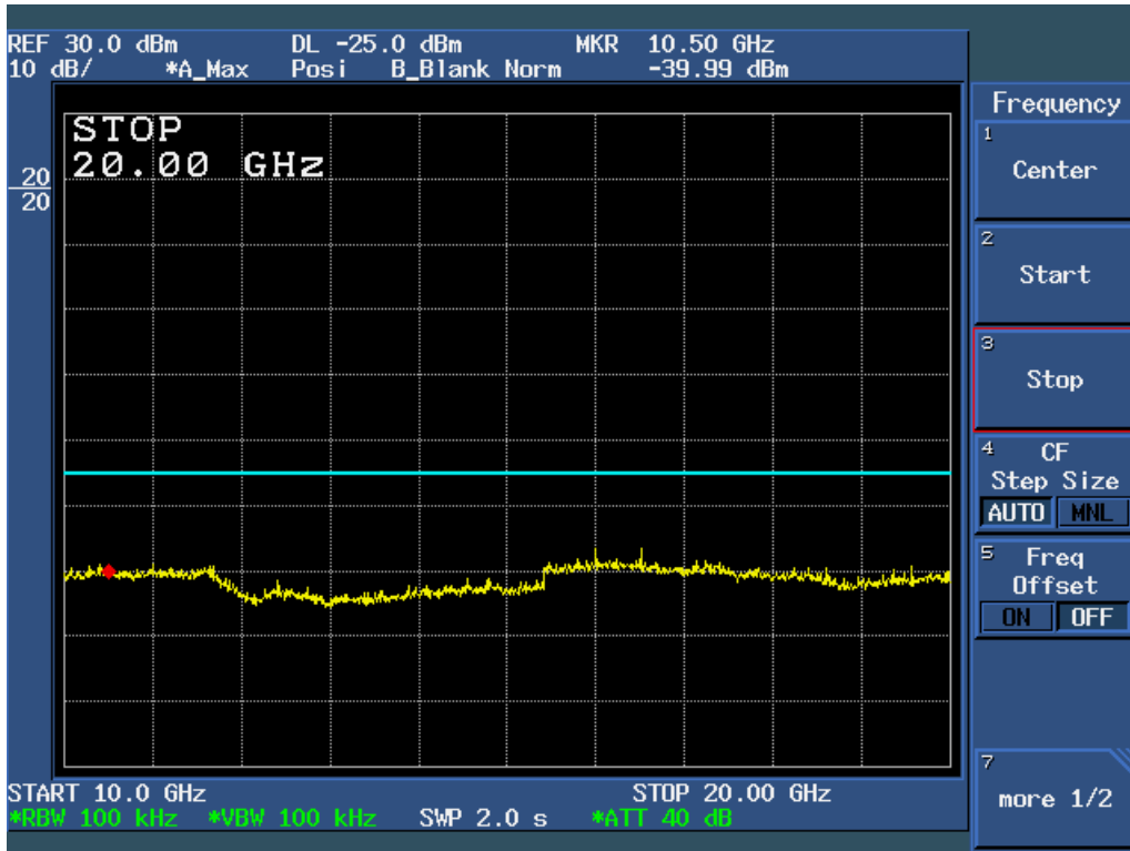
Figure 6c.5-15: Plot of Conducted Spurious Emissions, 10 – 20 GHz (54 Mbps data rate, Ch 1).
