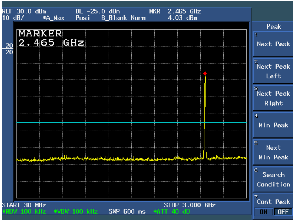
Figure 6c.5-9: Plot of Conducted Spurious Emissions, 30 – 3000 MHz (11 Mbps data rate, Ch 11).
