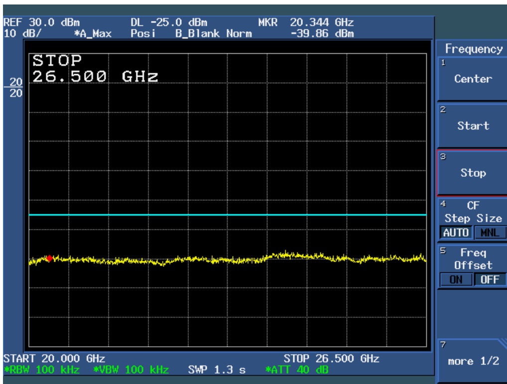
Figure 6c.5-8: Plot of Conducted Spurious Emissions, 20 – 26.5 GHz (11 Mbps data rate, Ch 6).
