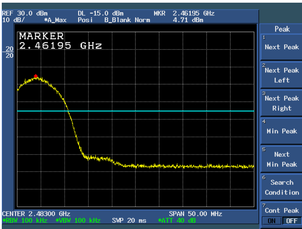
Figure 6c.6-2: Plot of Upper Band Edge Spurious Emission (11 Mbps data rate).
