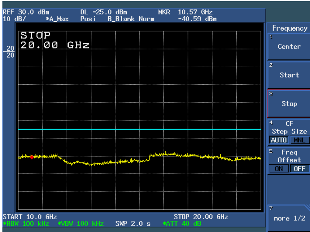
Figure 6c.5-11: Plot of Conducted Spurious Emissions, 10 – 20 GHz (11 Mbps data rate, Ch 11).
