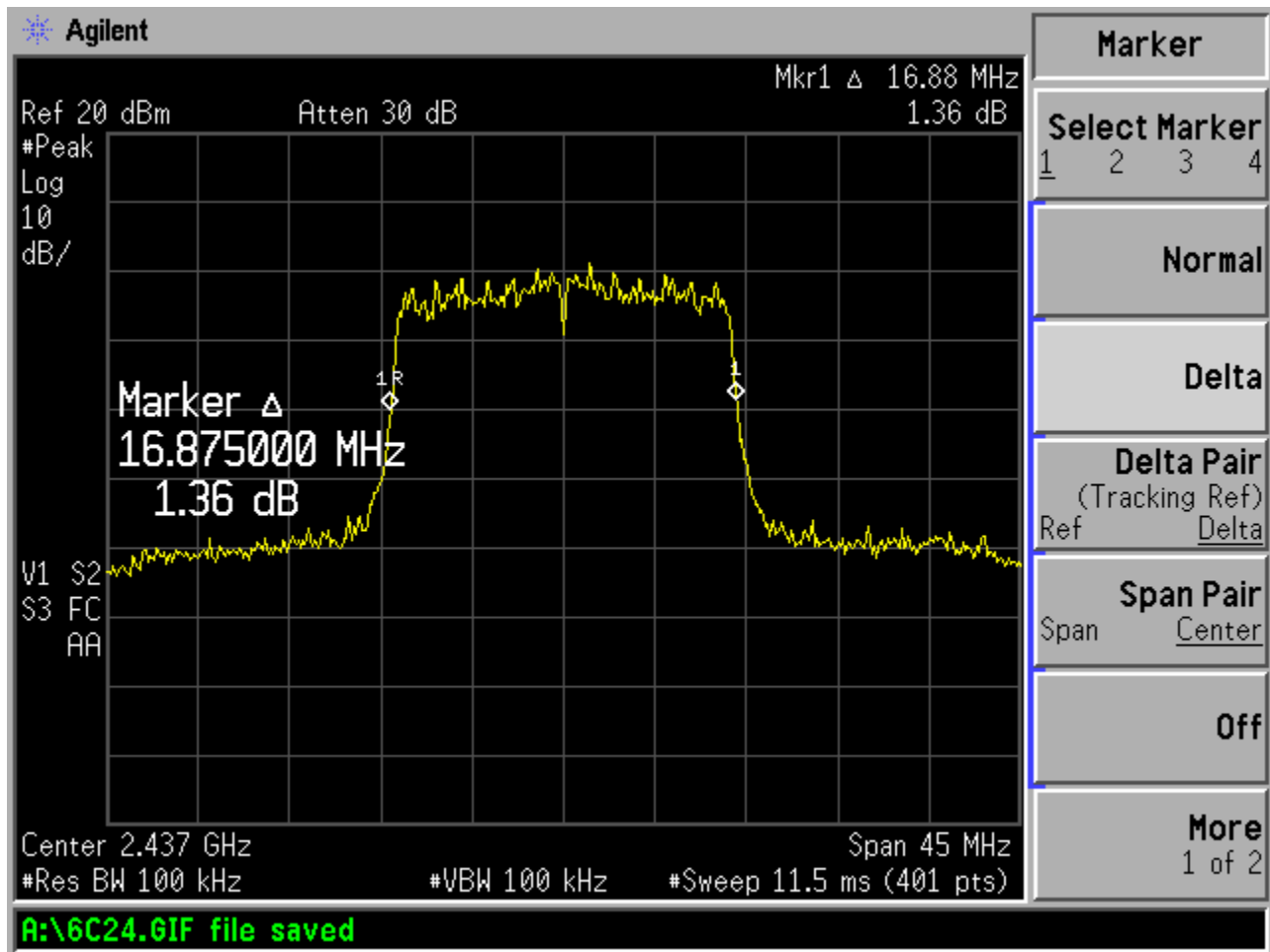
Figure 6c.2-5: Plot of 20 dB bandwidth (Channel 6, 54 Mbps data rate)
