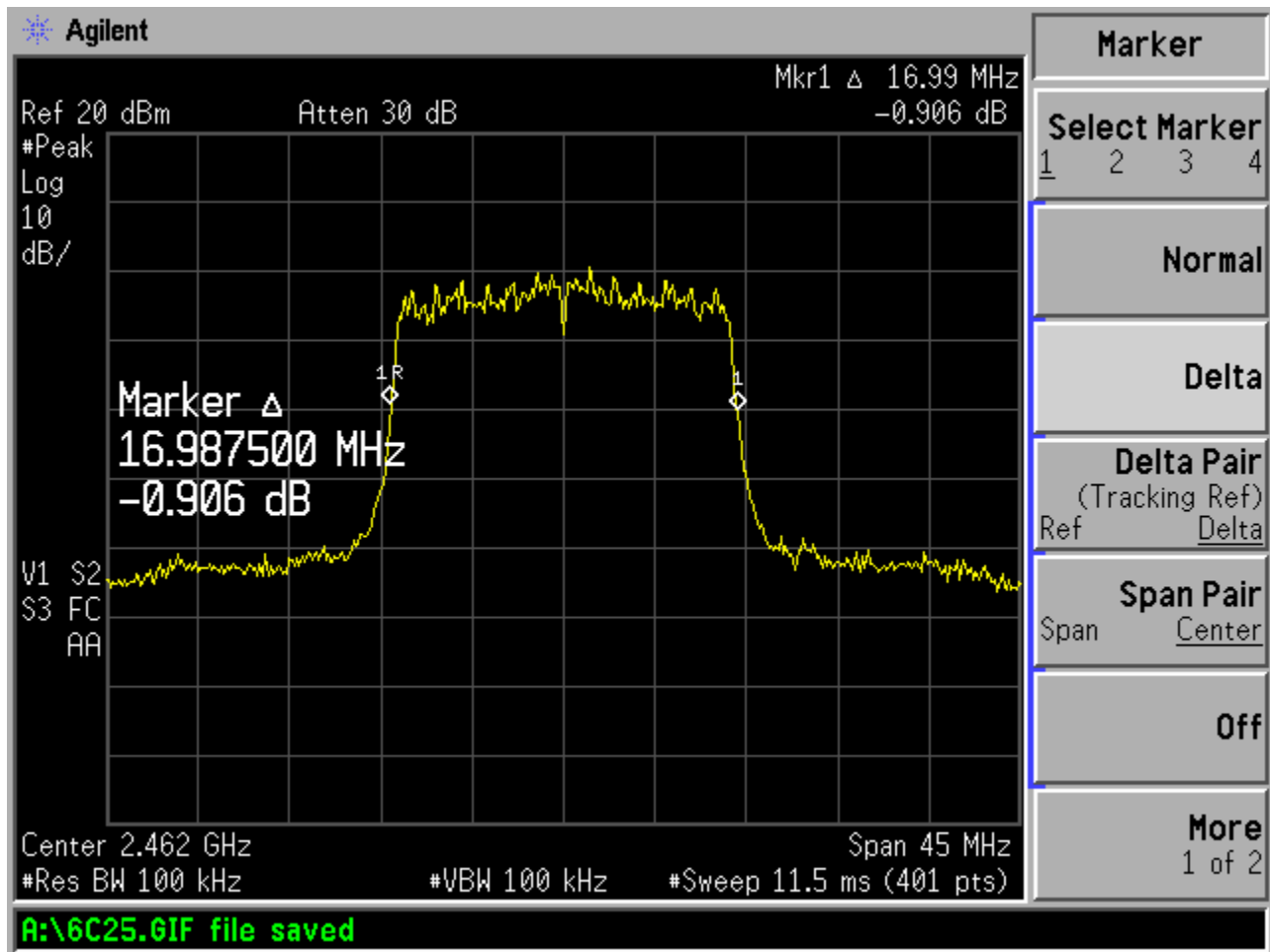
Figure 6c.2-6: Plot of 20 dB bandwidth (Channel 11, 54 Mbps data rate)
