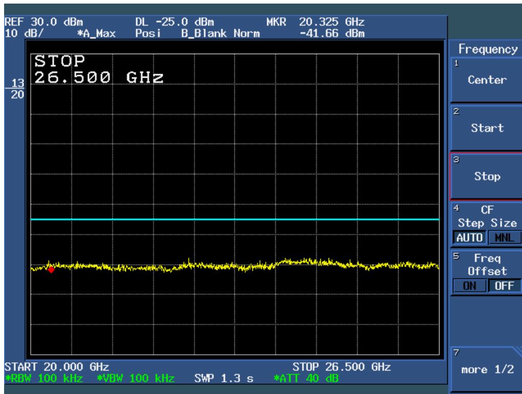
Figure 6c.5-4: Plot of Conducted Spurious Emissions, 20 – 26.5 GHz (11 Mbps data rate, Ch 1).
