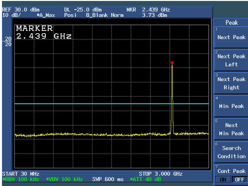
Figure 6c.5-5: Plot of Conducted Spurious Emissions, 30 – 3000 MHz (11 Mbps data rate, Ch 6).
