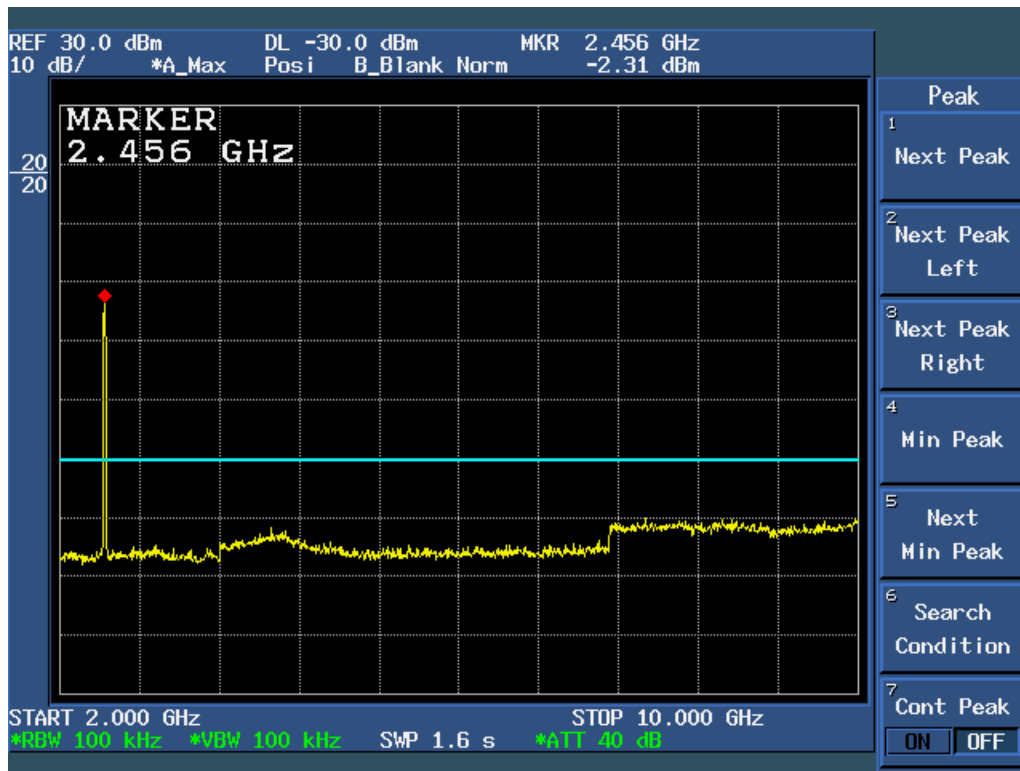
Figure 6c.5-22: Plot of Conducted Spurious Emissions, 2 – 10 GHz (54 Mbps data rate, Ch 11).
