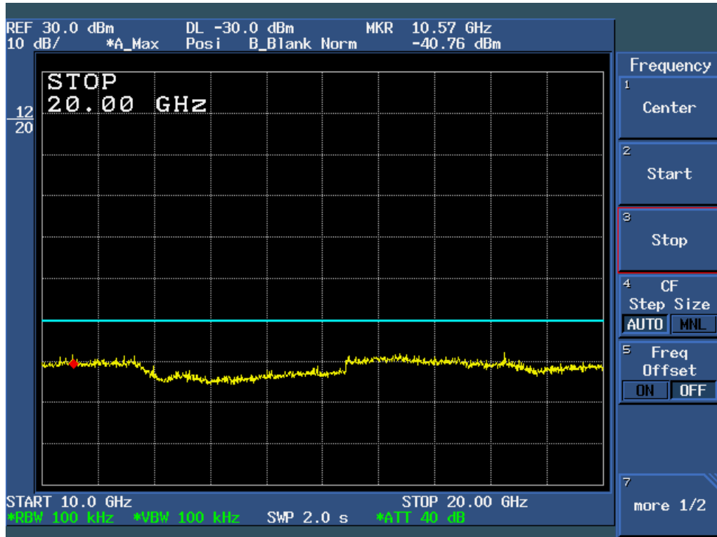
Figure 6c.5-23: Plot of Conducted Spurious Emissions, 10 – 20 GHz (54 Mbps data rate, Ch 11).
