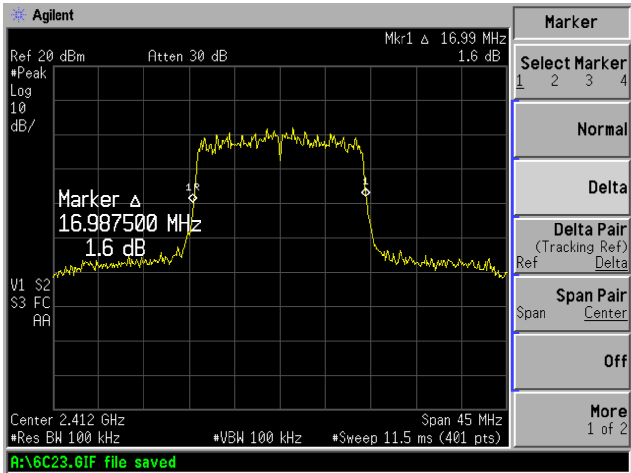
Figure 6c.2-4: Plot of 20 dB bandwidth (Channel 1, 54 Mbps data rate)
