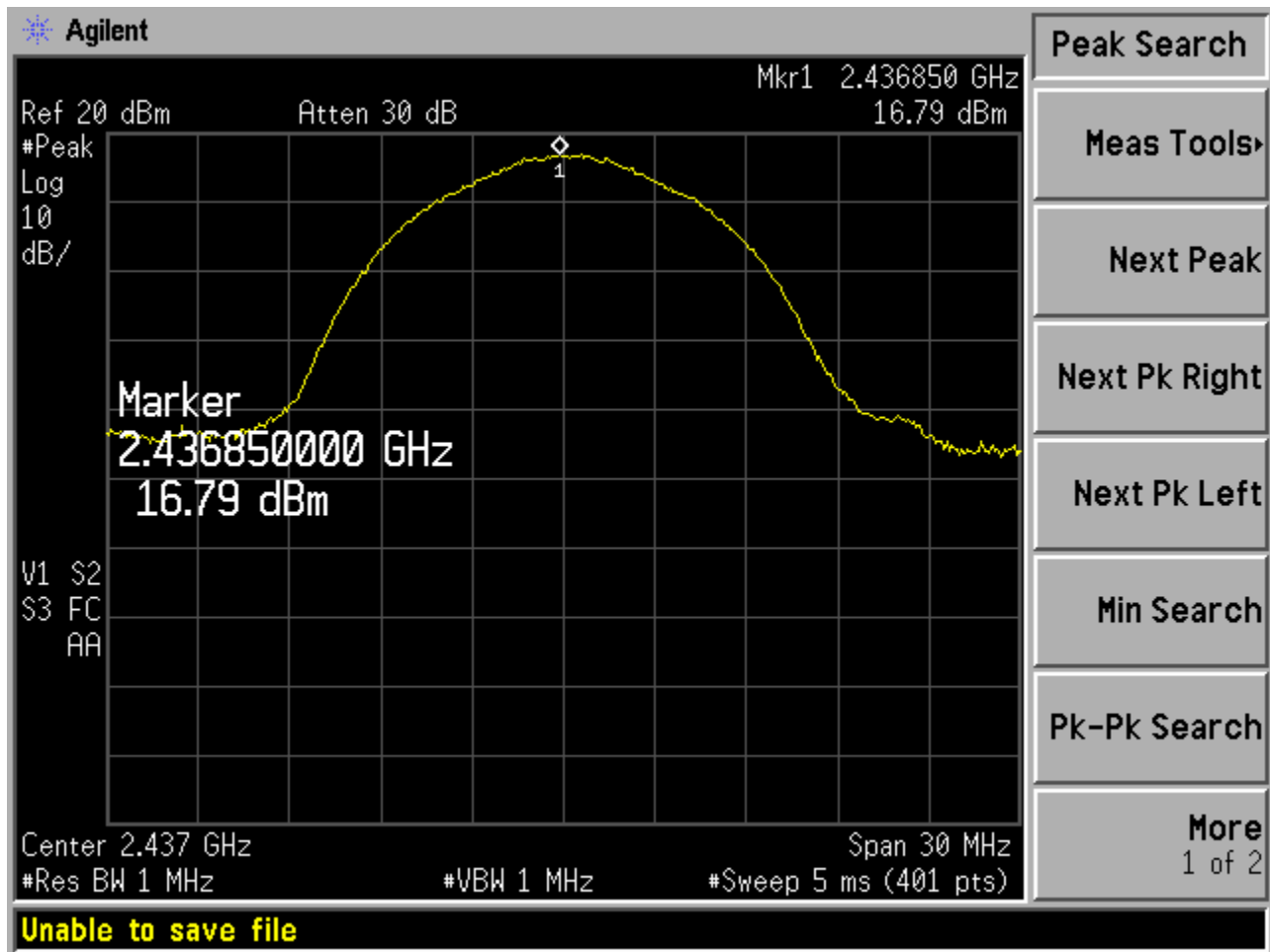
Figure 6c.3-2: Peak Output Power (Channel 6, 11 Mbps data rate)
