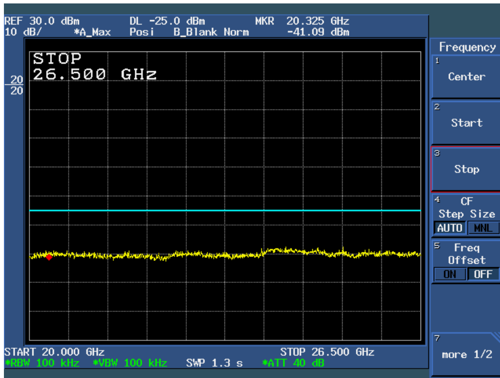
Figure 6c.5-16: Plot of Conducted Spurious Emissions, 20 – 26.5 GHz (54 Mbps data rate, Ch 1).
