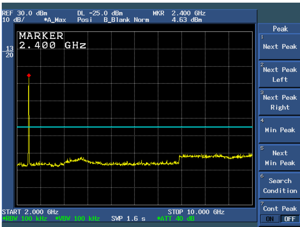
Figure 6c.5-2: Plot of Conducted Spurious Emissions, 2 – 10 GHz (11 Mbps data rate, Ch 1).
