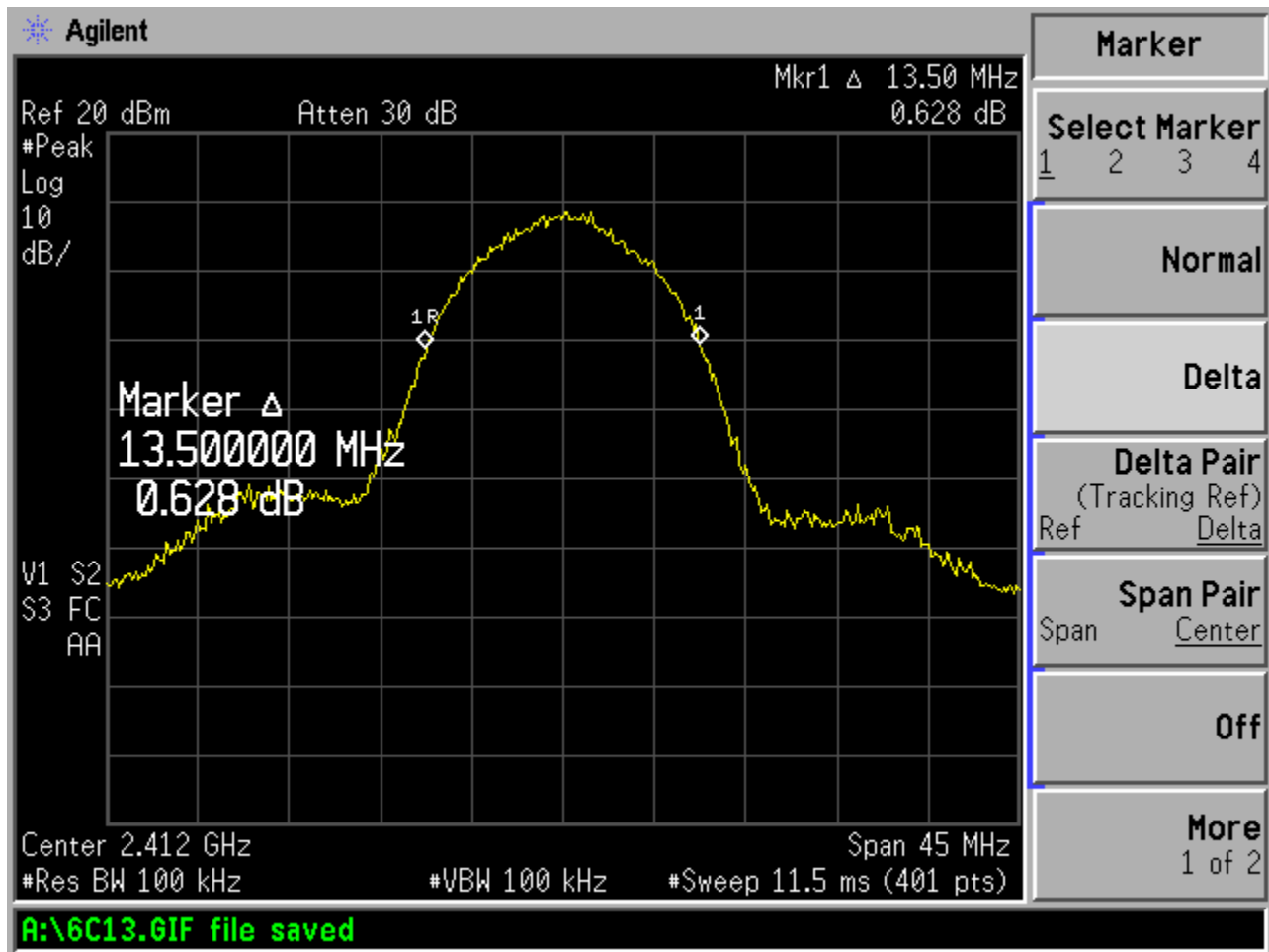
Figure 6c.1-4: Plot of 20 dB bandwidth (Channel 1, 11 Mbps data rate)
