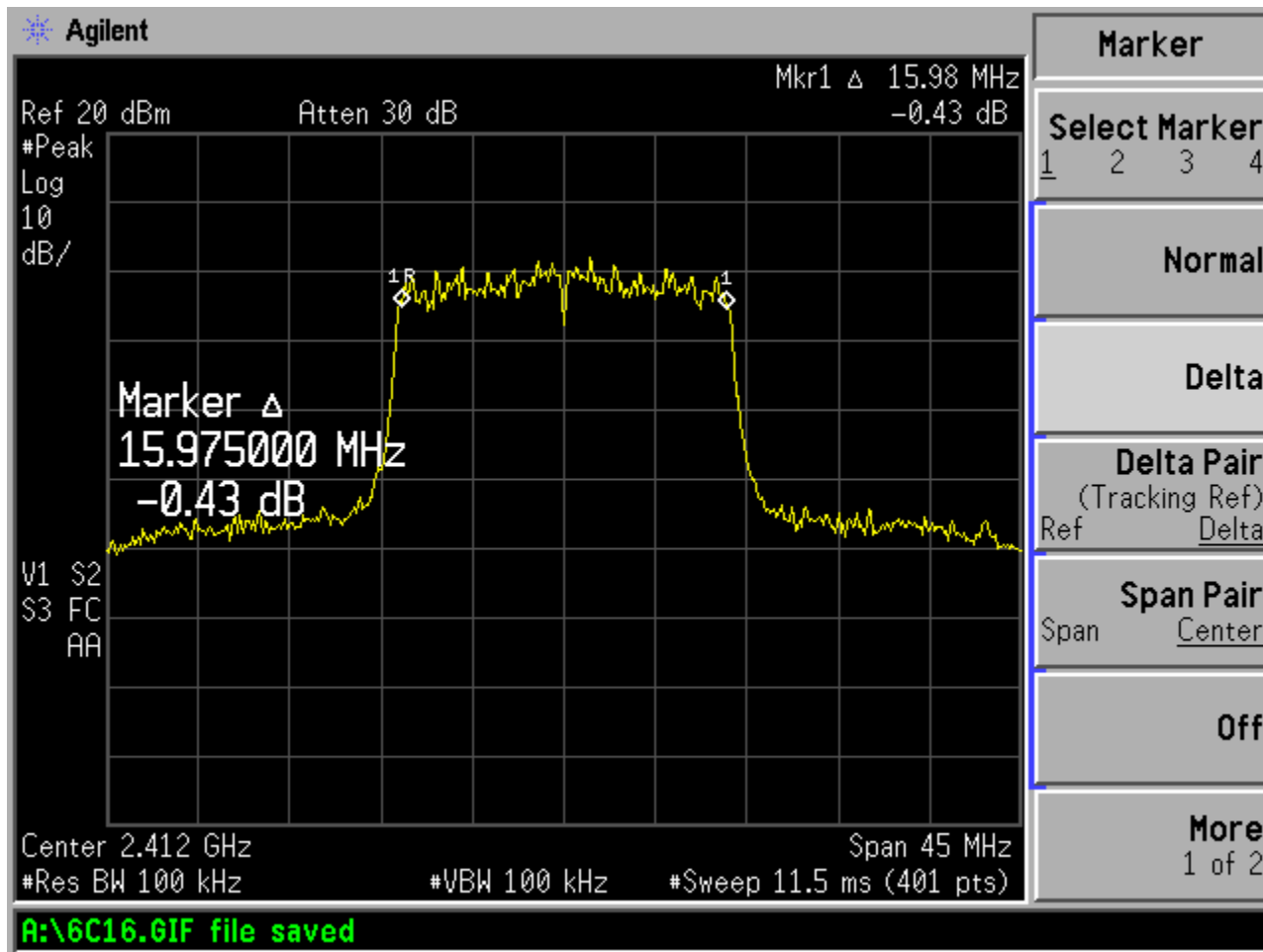
Figure 6c.2-1: Plot of 6 dB bandwidth (Channel 1, 54 Mbps data rate)
