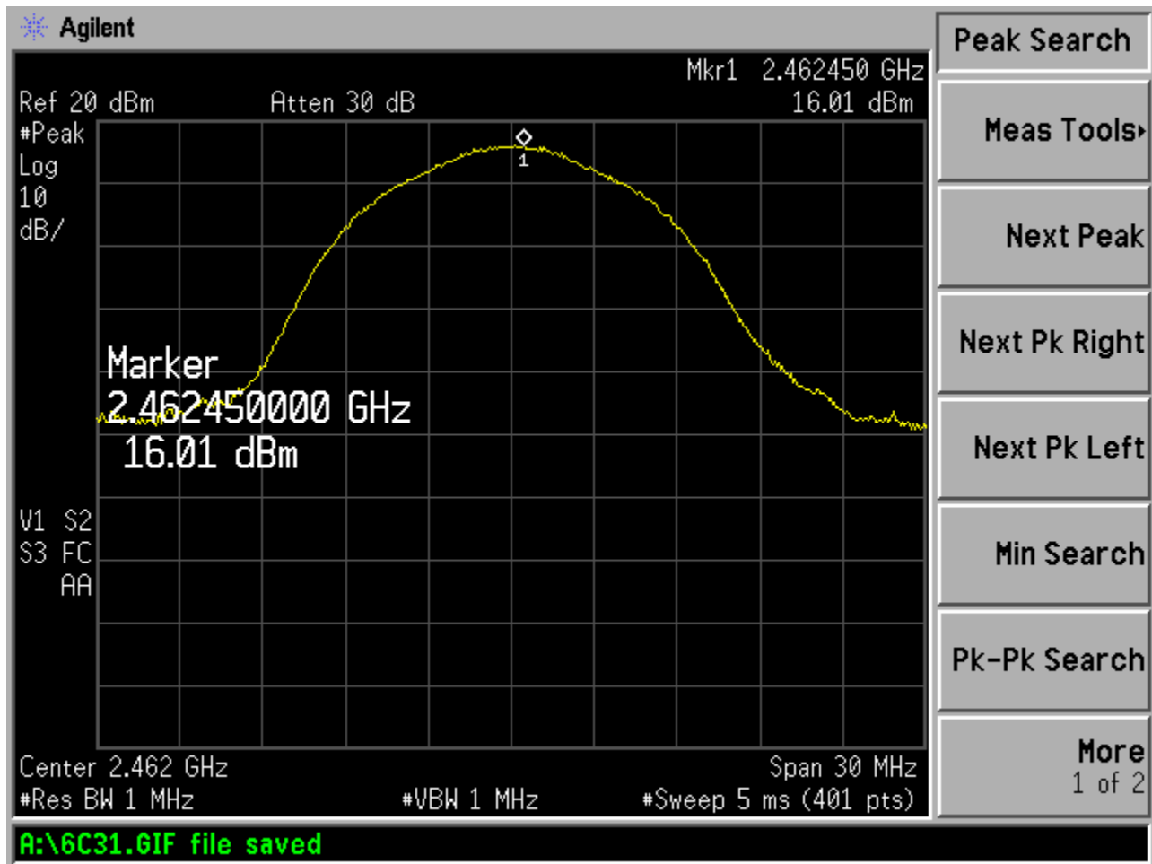
Figure 6c.3-3: Peak Output Power (Channel 11, 11 Mbps data rate)
