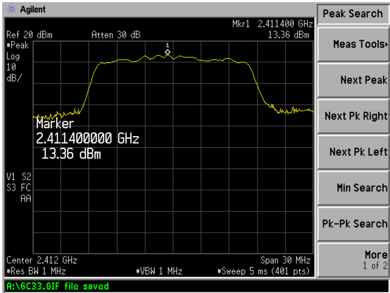
Figure 6c.3-4: Peak Output Power (Channel 1, 54 Mbps data rate)
