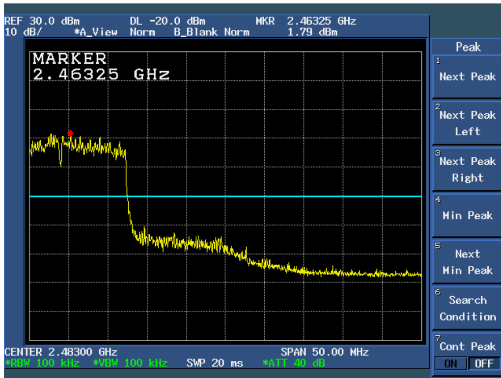
Figure 6c.6-1: Plot of Upper Band Edge Spurious Emission (54 Mbps data rate).
