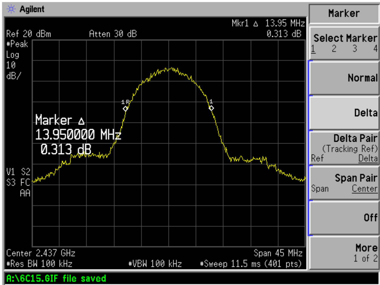
Figure 6c.1-5: Plot of 20 dB bandwidth (Channel 6, 11 Mbps data rate)
