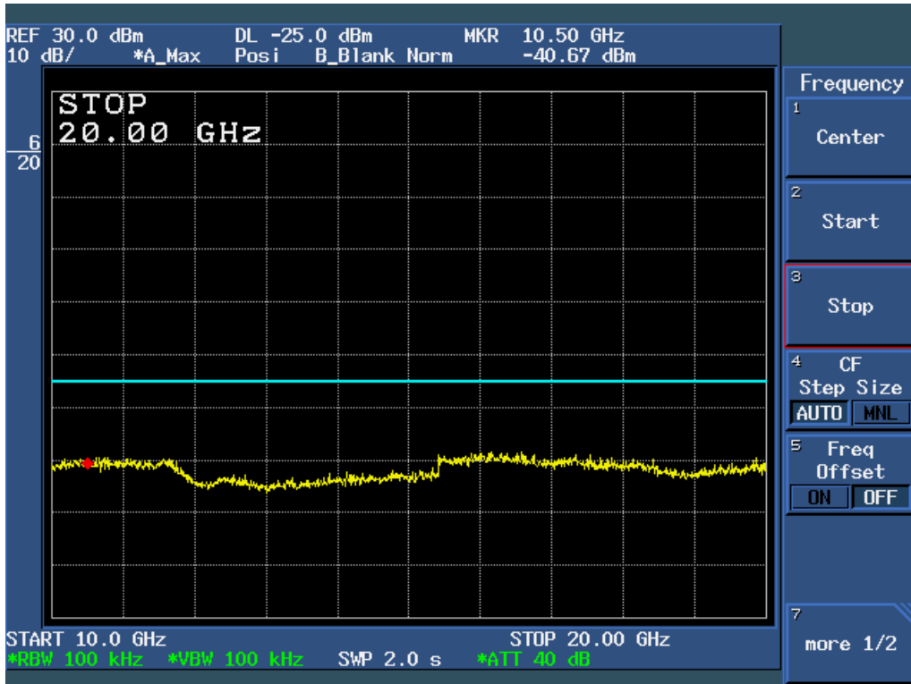
Figure 6c.5-3: Plot of Conducted Spurious Emissions, 10 – 20 GHz (11 Mbps data rate, Ch 1).
