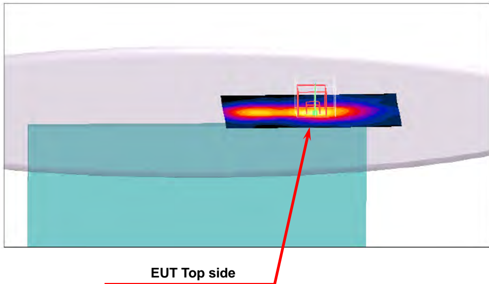
Figure 2. Body SAR Test Setup (Edge Top to phantom)
