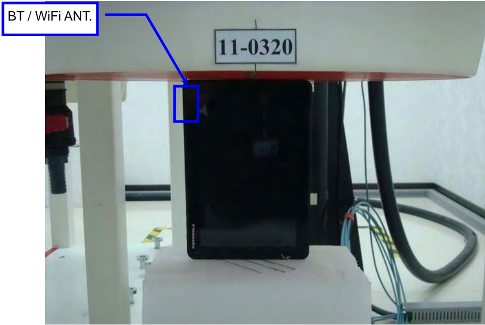
Figure 1. Body SAR Test Setup (Edge Right to phantom)
