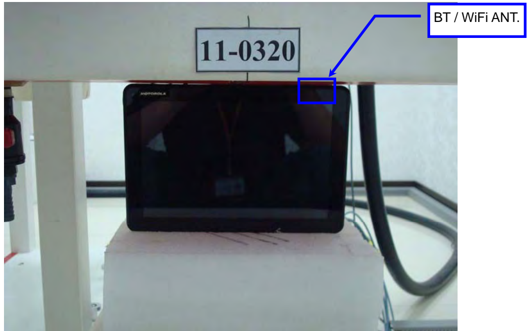
Figure 2. Body SAR Test Setup (Edge Top to phantom)
