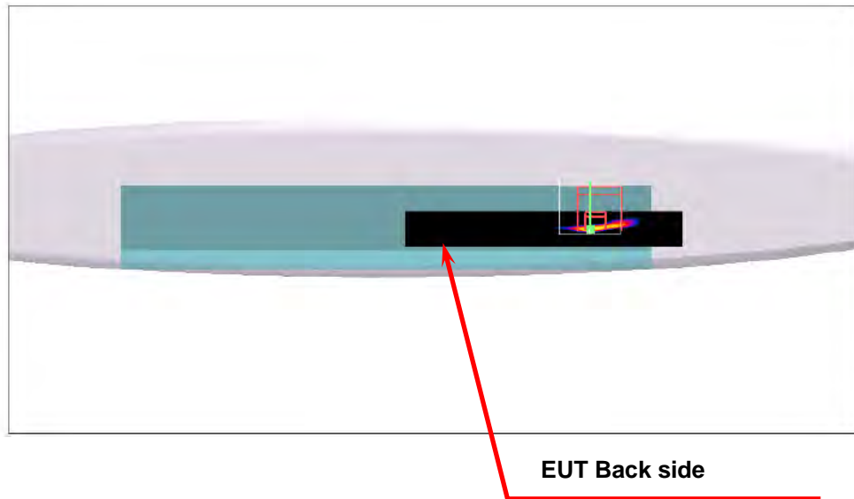
Figure 3. Body SAR Test Setup (Back Surface to phantom)
