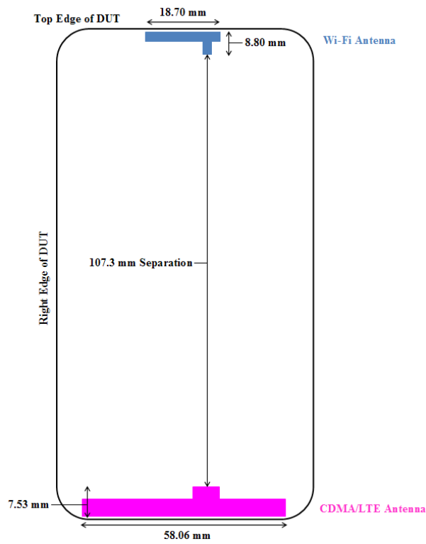
Figure 2: Antenna Separation Distances
