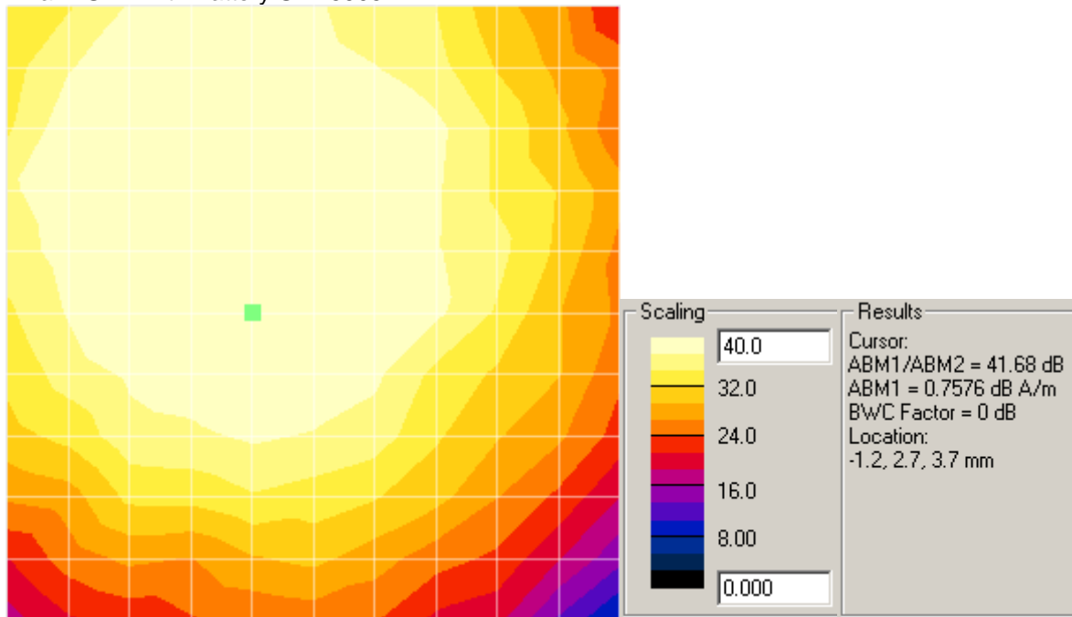
Axial – SNR with Battery SNN5905A
