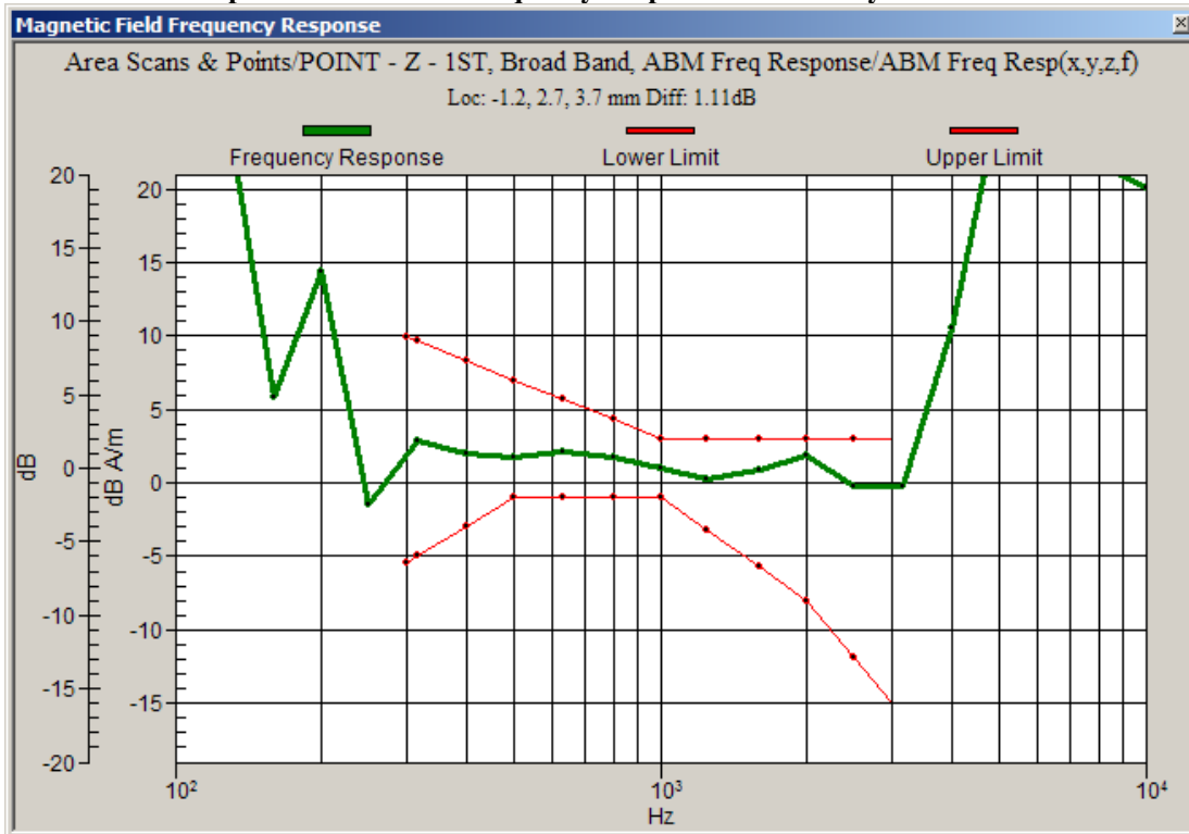
Graph 3: CDMA 1900 Frequency Response with Battery SNN5905A
