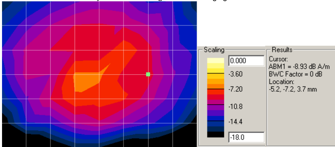
Radial2 – ABM1 with Battery SNN5905A using inductive charging door SJHN0813A
