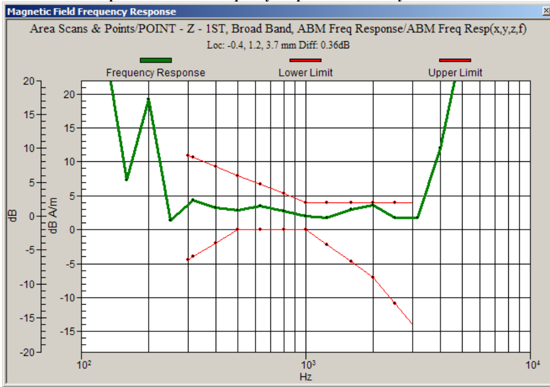
Graph 2: CDMA 800 Frequency Response with Battery SNN5905A
