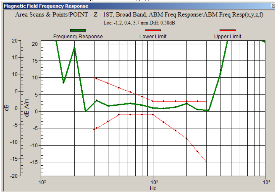
Graph 5: CDMA 1900 Frequency Response with Battery SNN5905A using inductive charging door SJHN0813A
