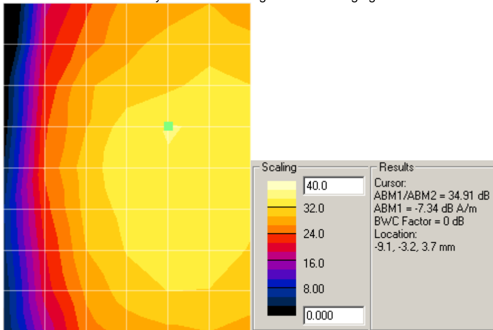
Radial1 – SNR with Battery SNN5905A using inductive charging door SJHN0813A
