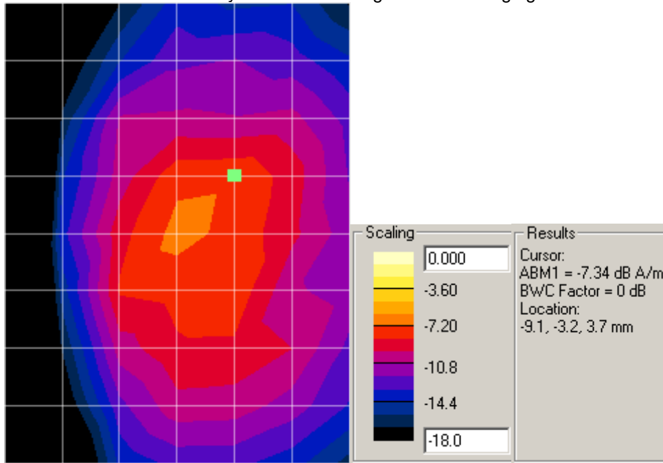
Radial1 – ABM1 with Battery SNN5905A using inductive charging door SJHN0813A
