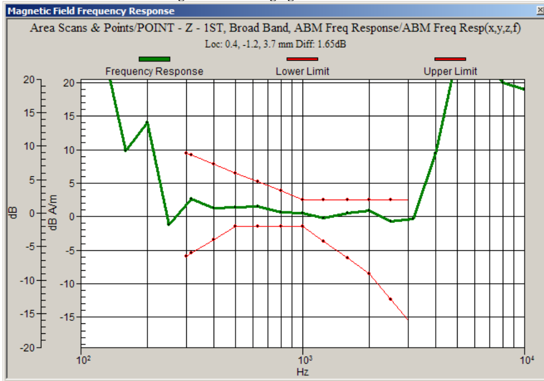
Graph 4: CDMA 800 Frequency Response with Battery SNN5905A using inductive charging door SJHN0813A
