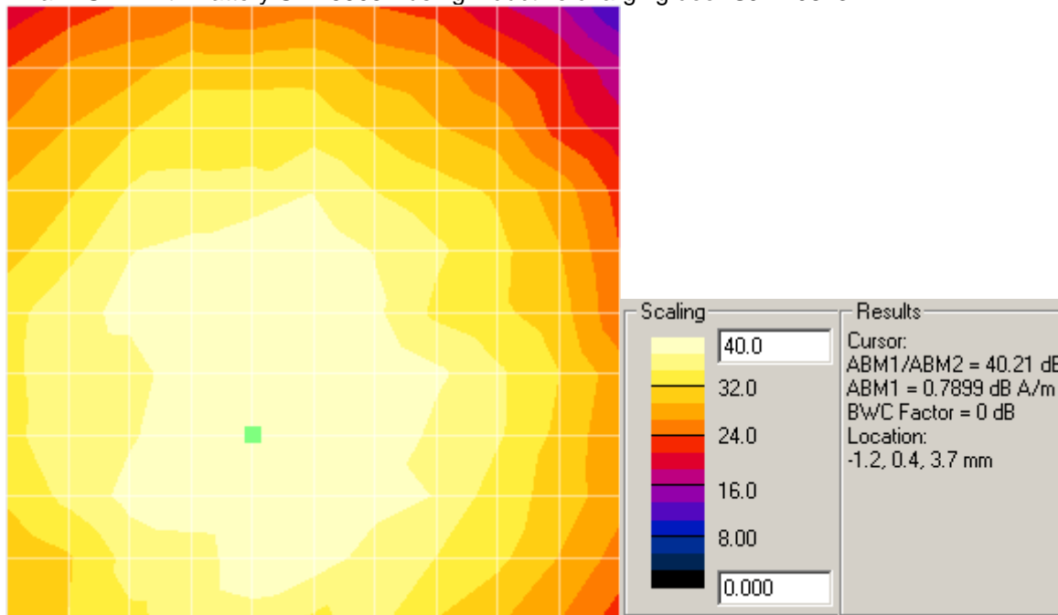
Axial – SNR with Battery SNN5905A using inductive charging door SJHN0813A
