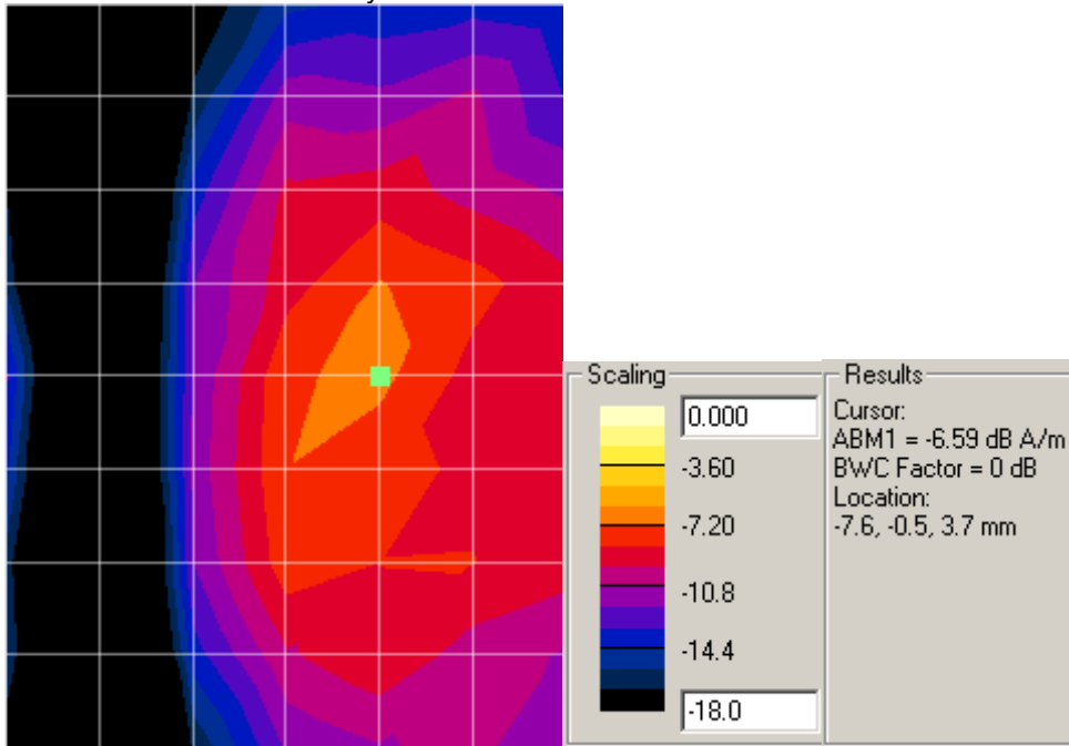
Radial1 – ABM1 with Battery SNN5905A
