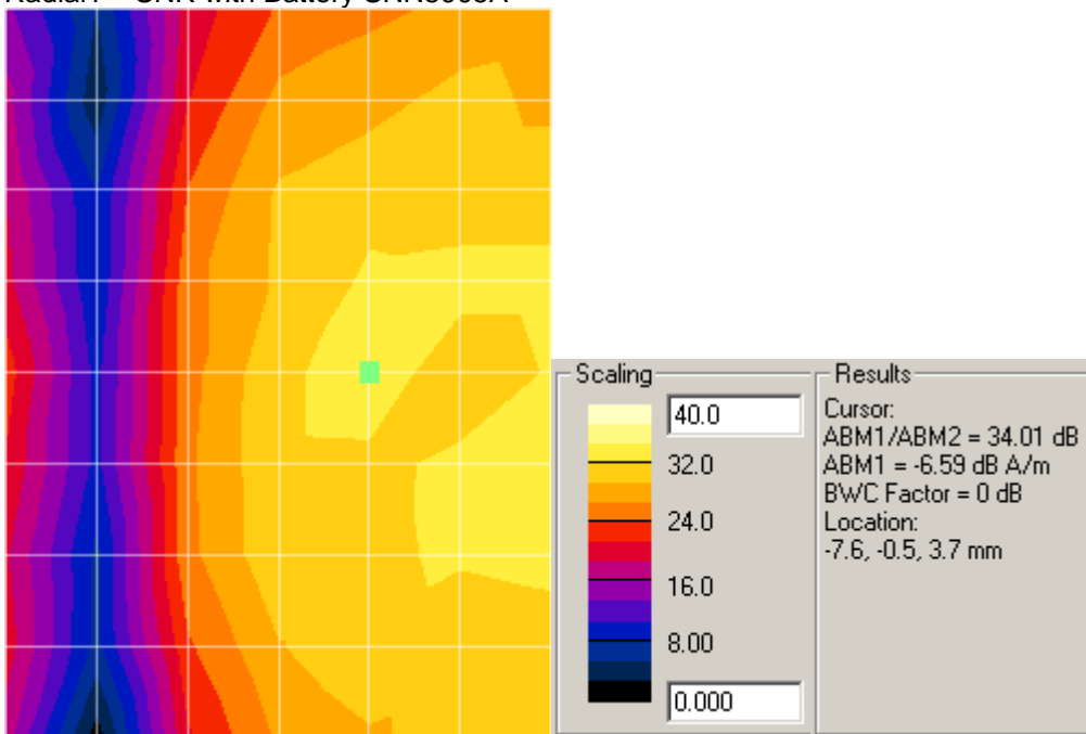
Radial1 – SNR with Battery SNN5905A
