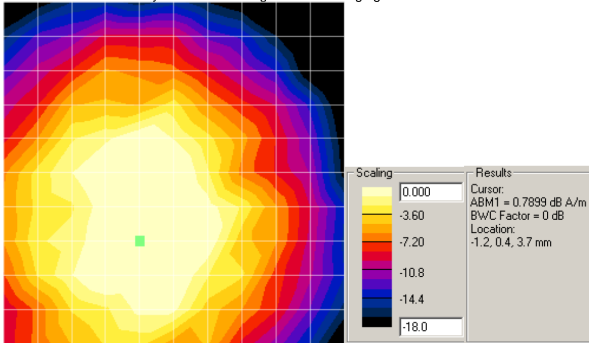
Axial – ABM1 with Battery SNN5905A using inductive charging door SJHN0813A
