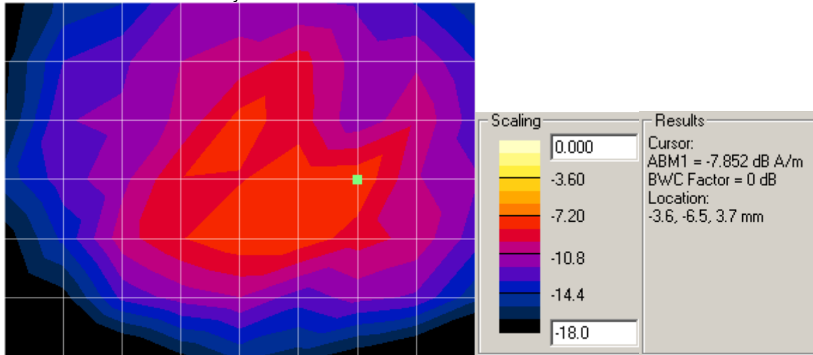
Radial2 – ABM1 with Battery SNN5905A
