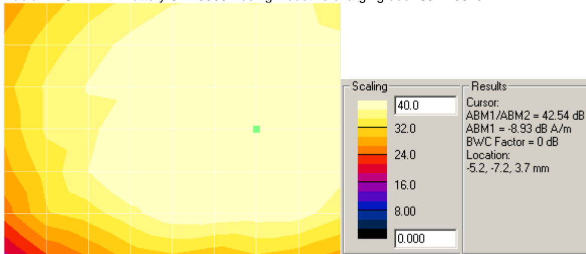
Radial2 – SNR with Battery SNN5905A using inductive charging door SJHN0813A
