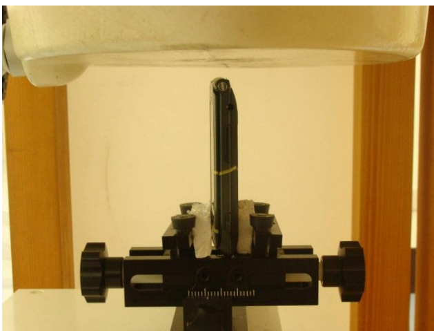
Top Side of the DUT with Phantom 1 cm Gap (DUT without Earphone)
