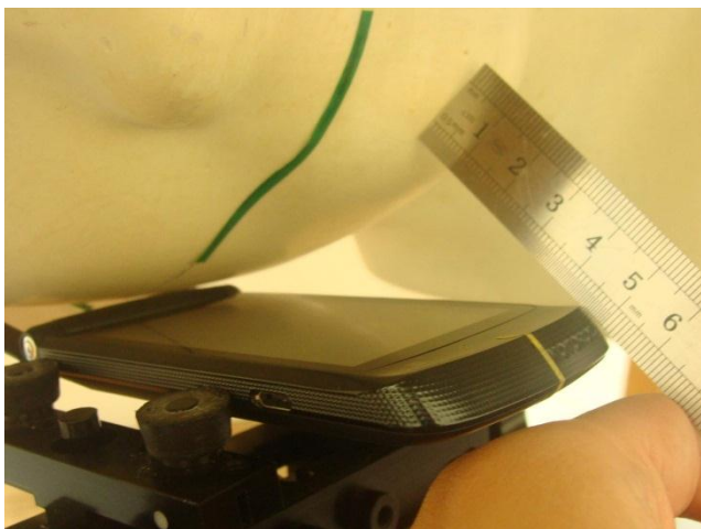
Right Cheek position - Separation distance 4.5cm between mouth and antenna
