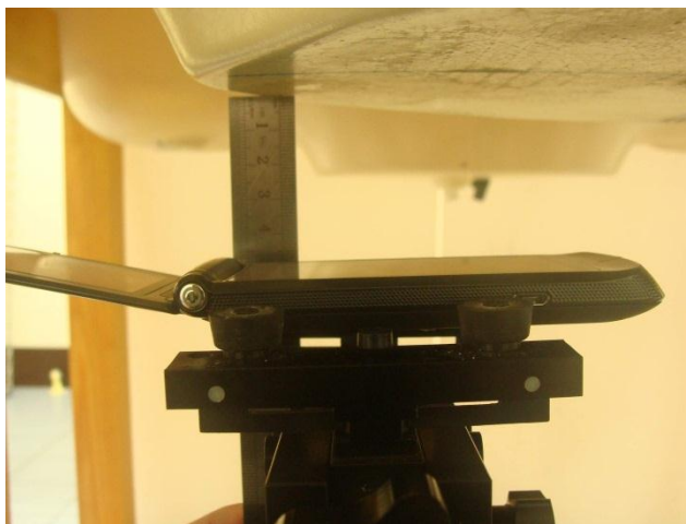
Right Cheek position - Separation distance 4.5cm between mouth and antenna
