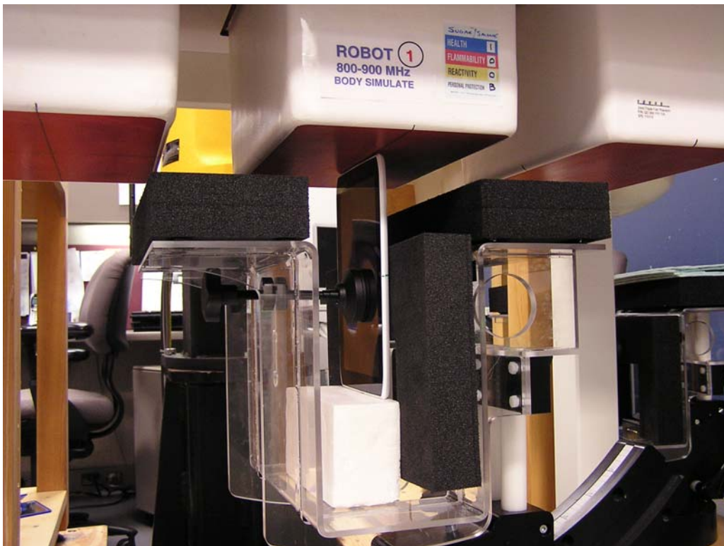
Figure 3: Top Edge of DUT toward Phantom, 0 mm Separation
