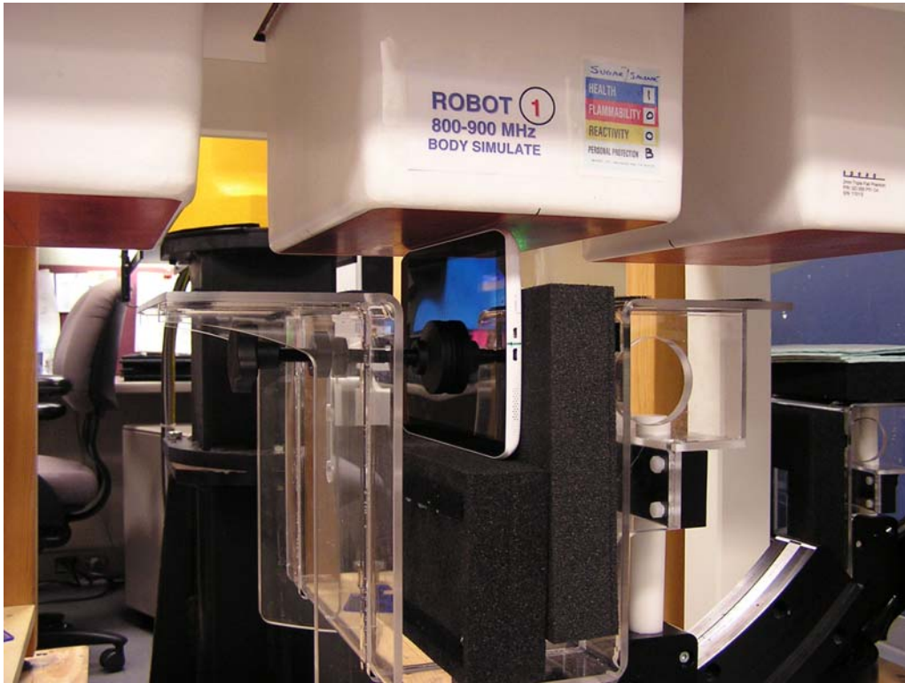
Figure 4: Right Edge of DUT toward Phantom, 0 mm Separation
