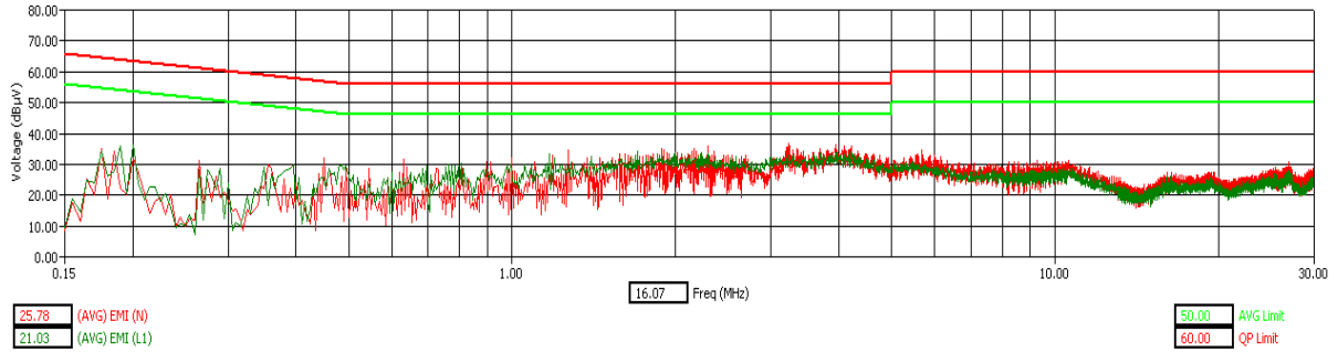
WLAN Channel 1 - Tx Mode - AVG Detector
