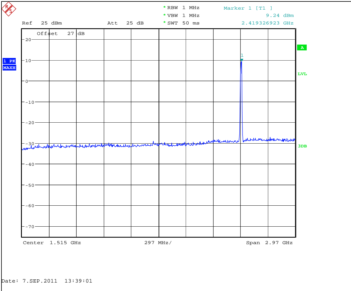
Conducted Spurious Emissions 30-3000MHz (Low Channel)
