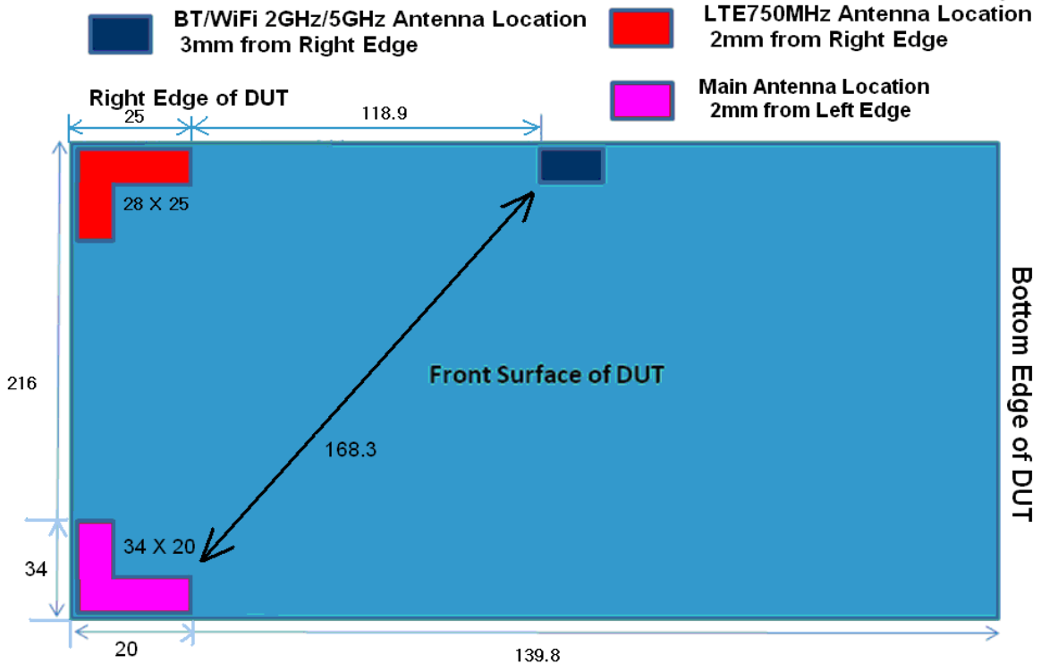
Figure 2: Device Dimensions and Antenna Separation Distances
