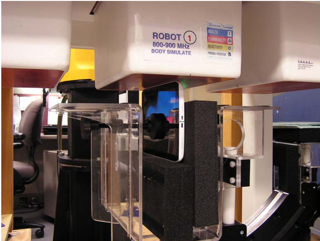
Figure 5: Right Edge of DUT toward Phantom, 0 mm Separation
