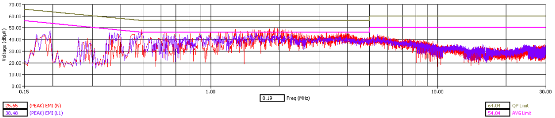
WLAN Channel 48 - Tx Mode - Peak Detector
