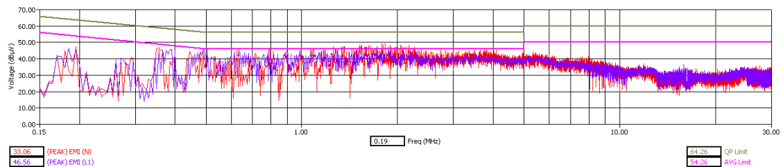
WLAN Channel 44 - Tx Mode - Peak Detector
