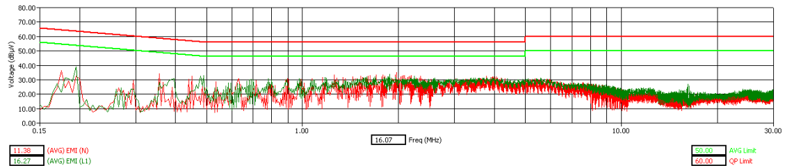
WLAN Channel 36 - Tx Mode - AVG Detector
