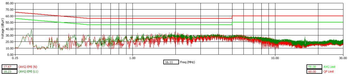
WLAN Channel 48 - Tx Mode - AVG Detector
