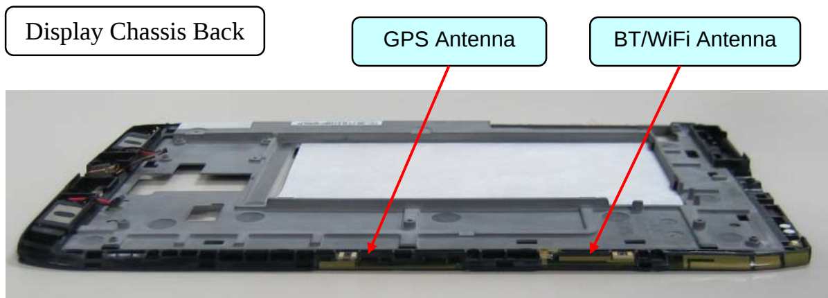
Main, Diversity, GPS, and BT/WiFi Antenna Location
