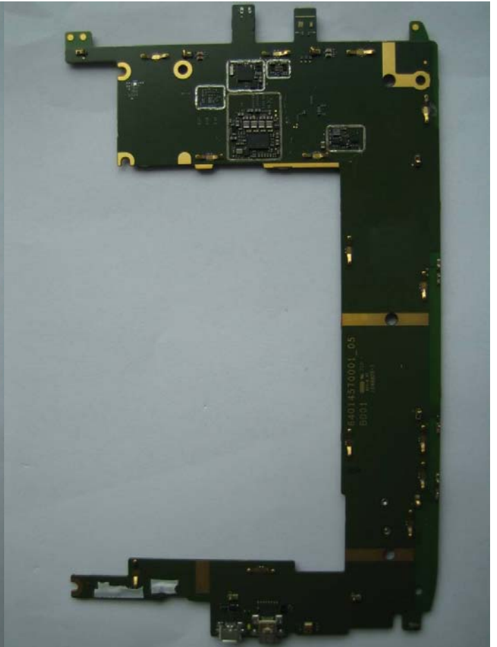
Main Board Bottom without Shields
