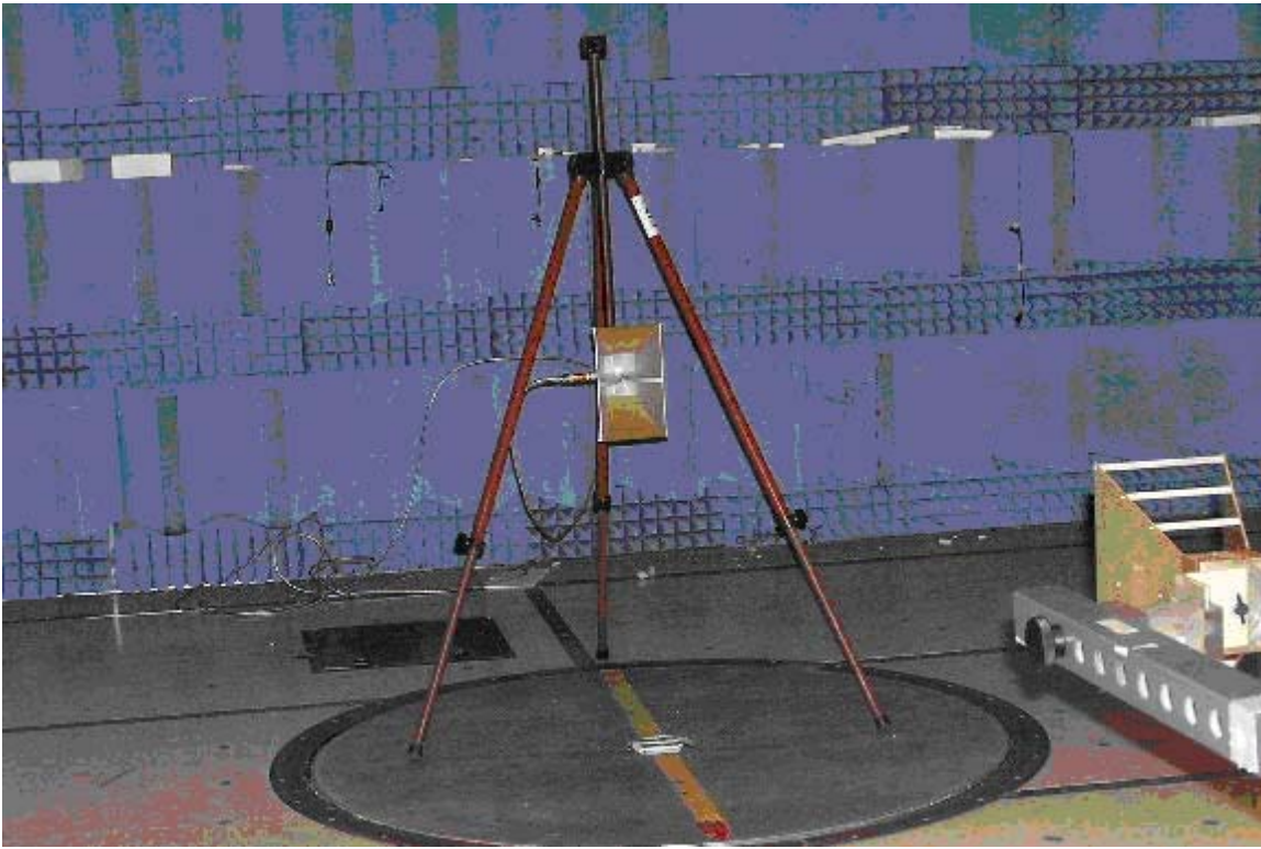
Antenna - Substitution
