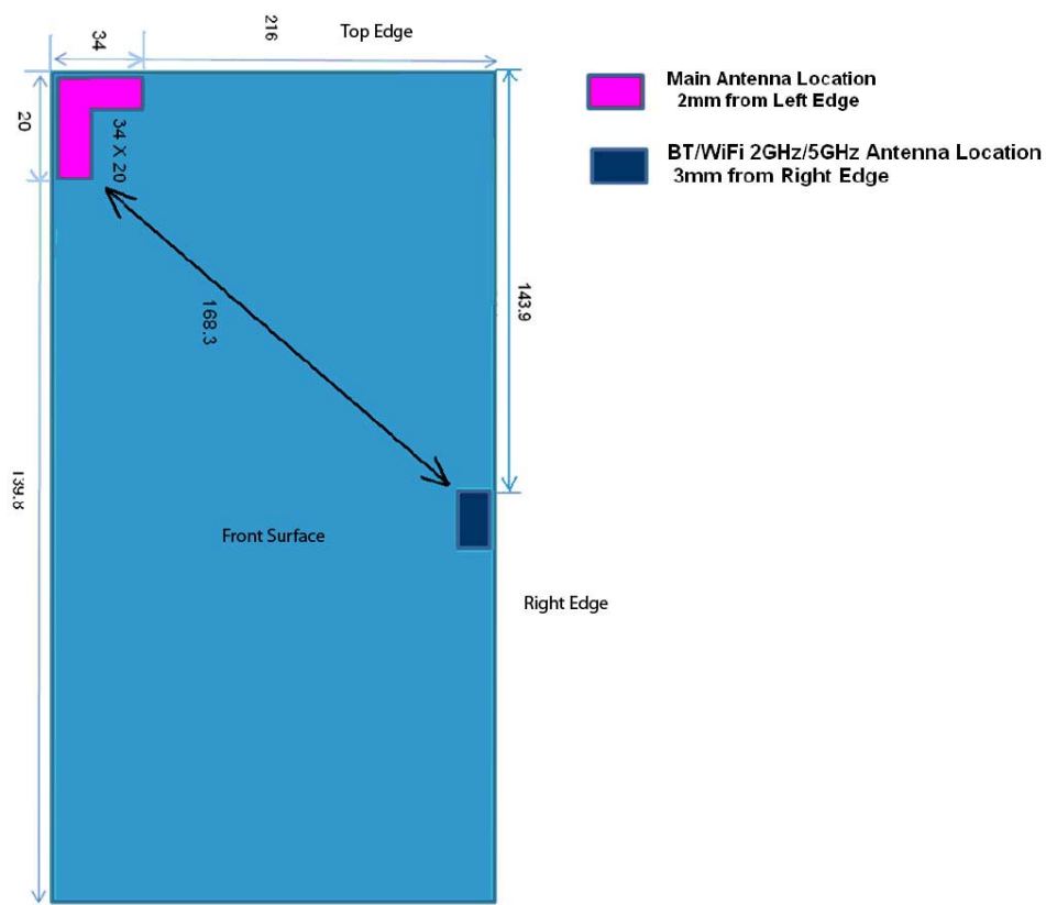
Figure 2: Device Dimensions and Antenna Separation Distances
