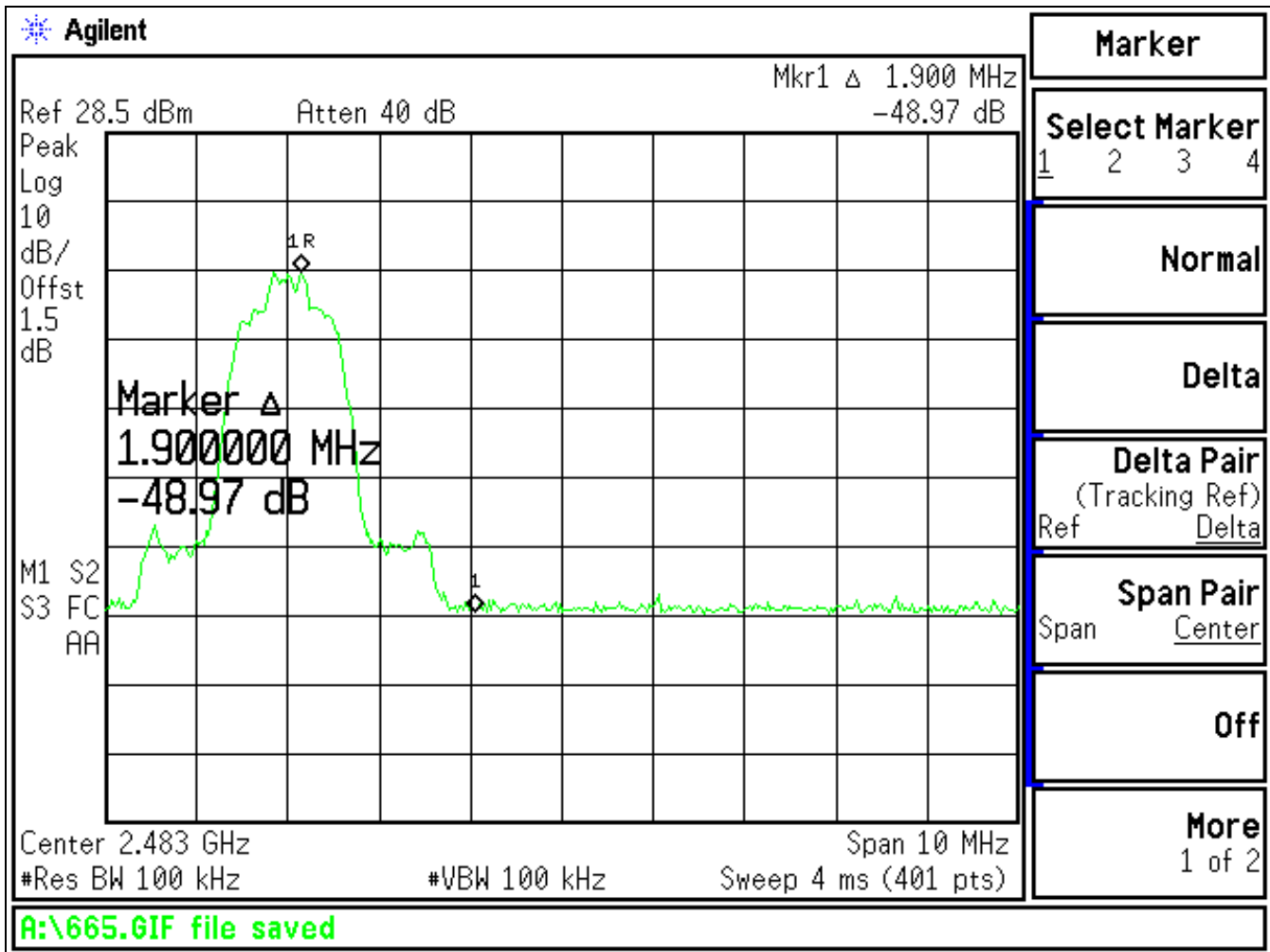
Figure 6d.6-6: Plot of upper band-edge conducted emissions with hopping disabled (Pi/4 DPSK Modulation).
