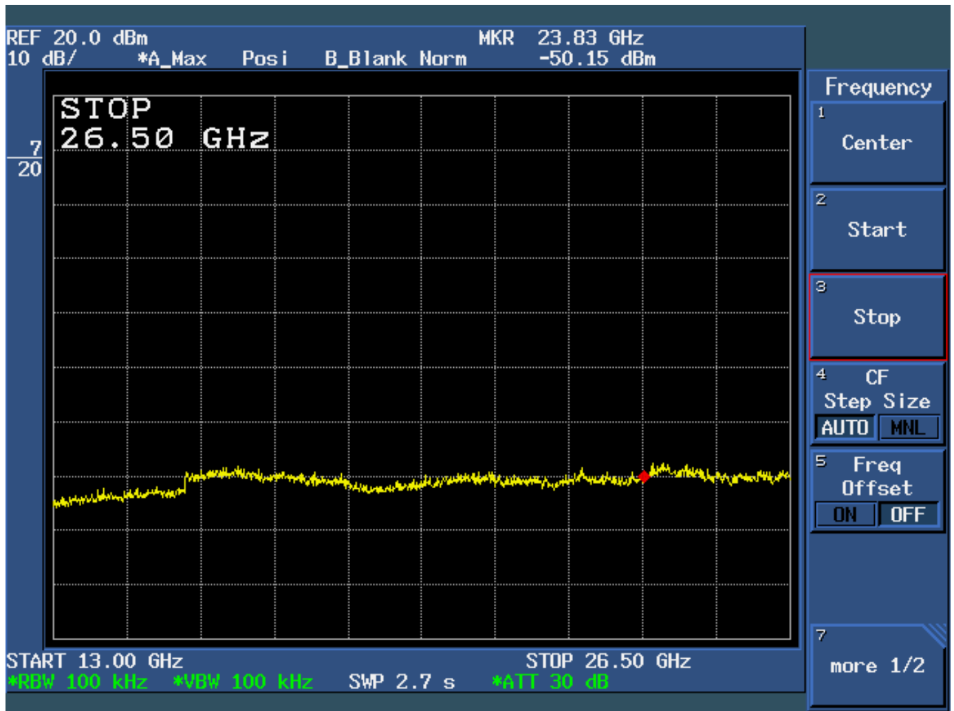
Figure 6d.7-3: Plot of spurious conducted emissions 13 GHz – 26.5 GHz (Low Channel Enabled).
