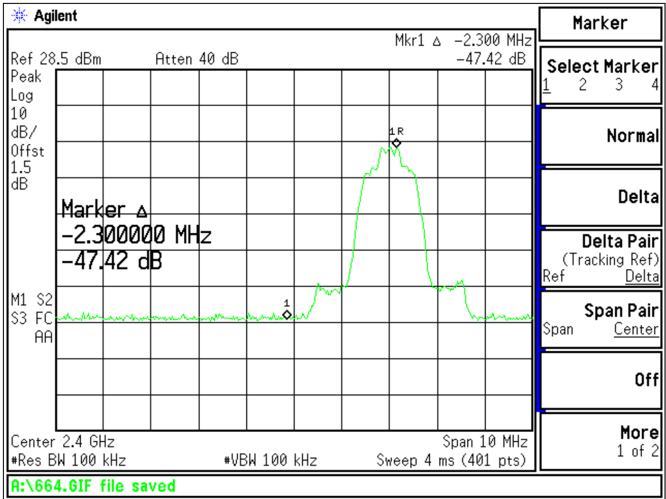
Figure 6d.6-5: Plot of lower band-edge conducted emissions with hopping disabled (Pi/4 DPSK Modulation).
