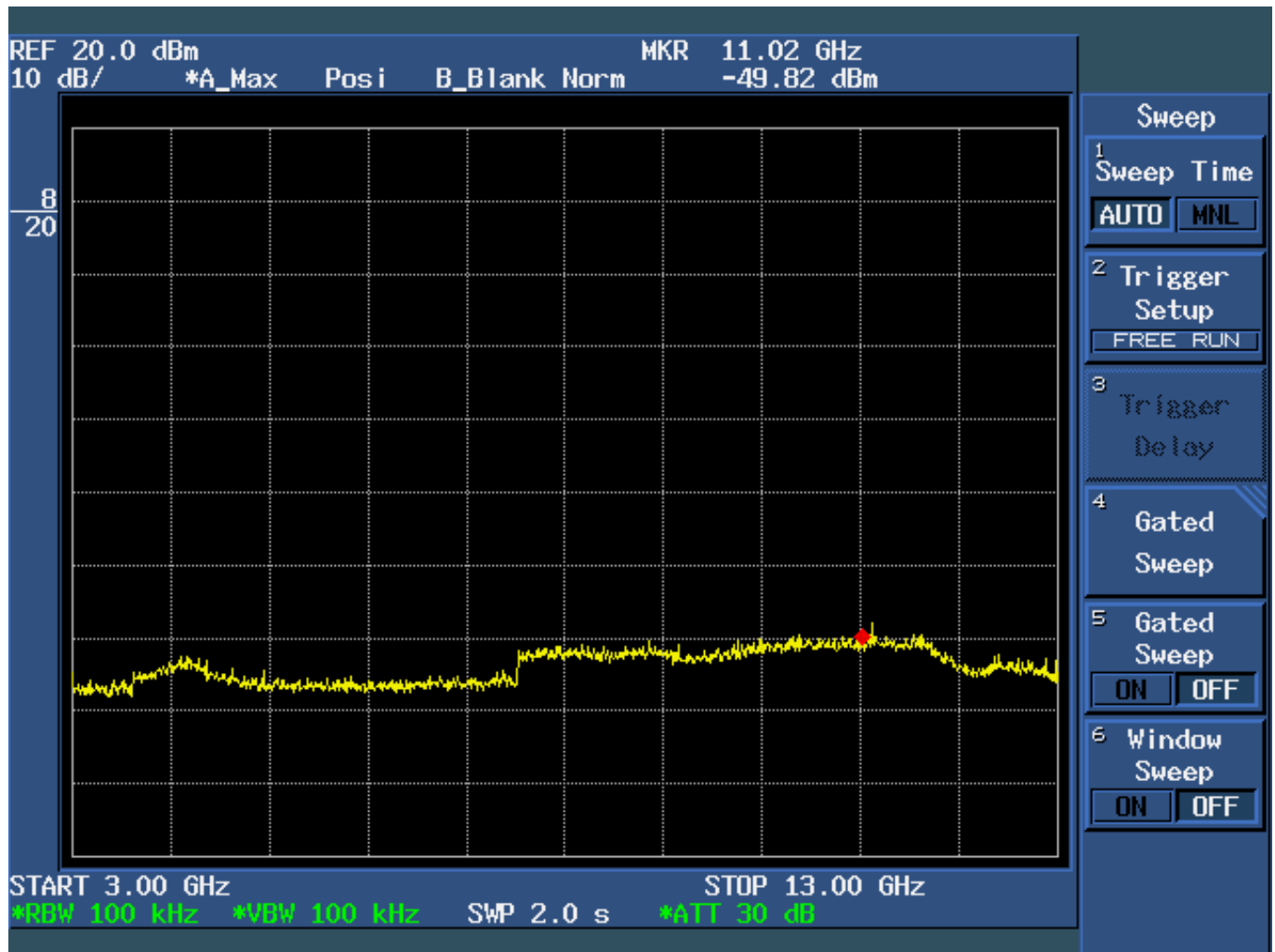
Figure 6d.7-2: Plot of spurious conducted emissions 3 GHz – 13 GHz (Low Channel Enabled).
