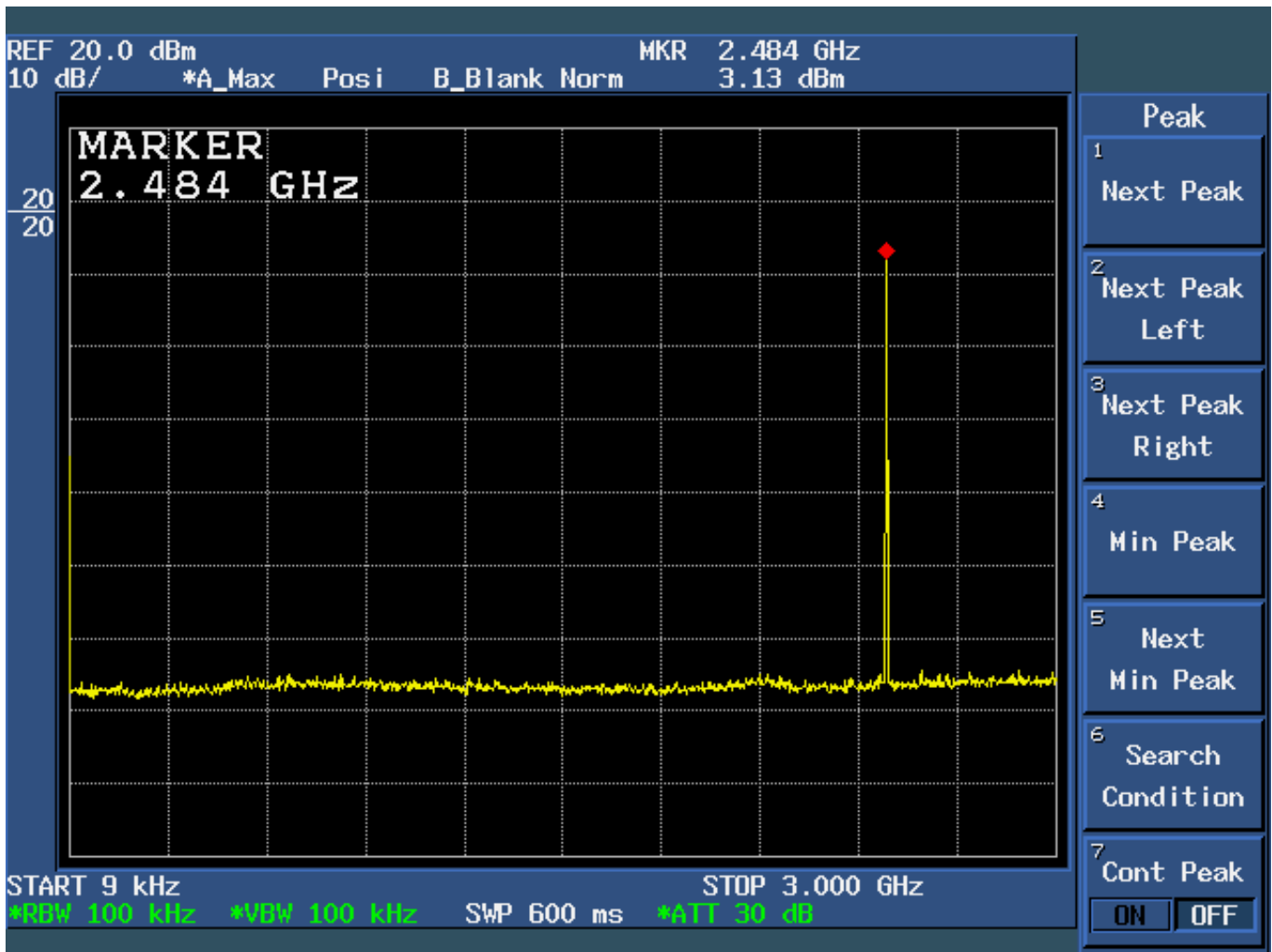
Figure 6d.7-7: Plot of spurious conducted emissions 9 kHz – 3.0 GHz (High Channel Enabled).
