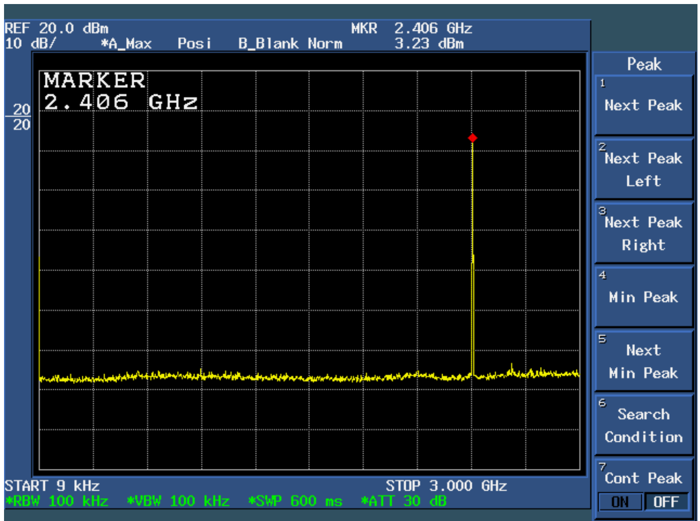
Figure 6d.7-1: Plot of spurious conducted emissions 9 kHz – 3.0 GHz (Low Channel Enabled).
