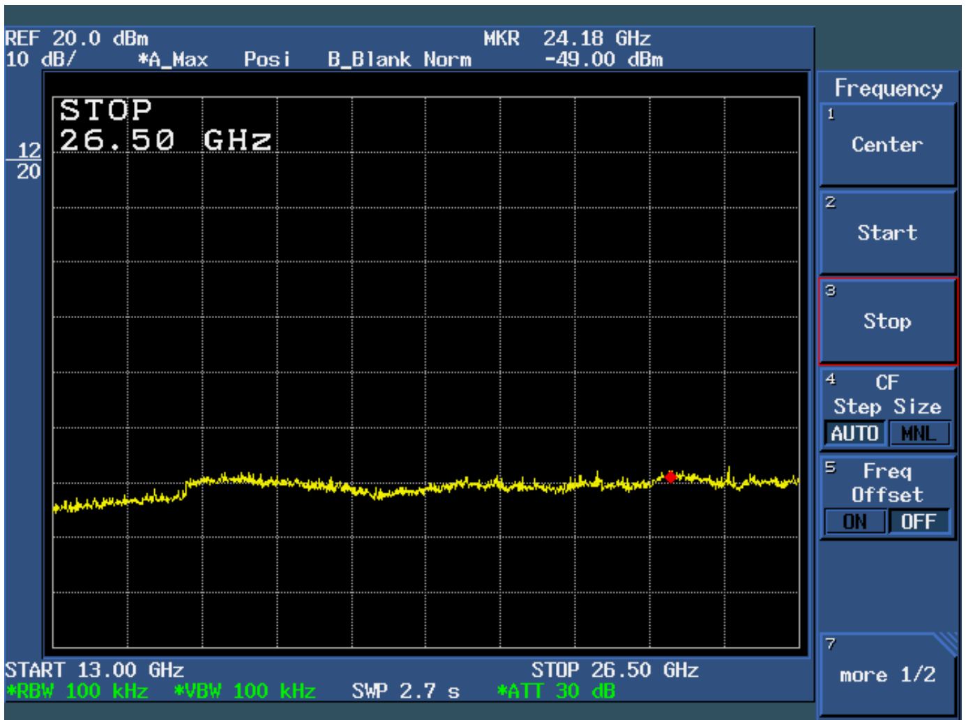
Figure 6d.7-9: Plot of spurious conducted emissions 13 GHz – 26.5 GHz (High Channel Enabled).
