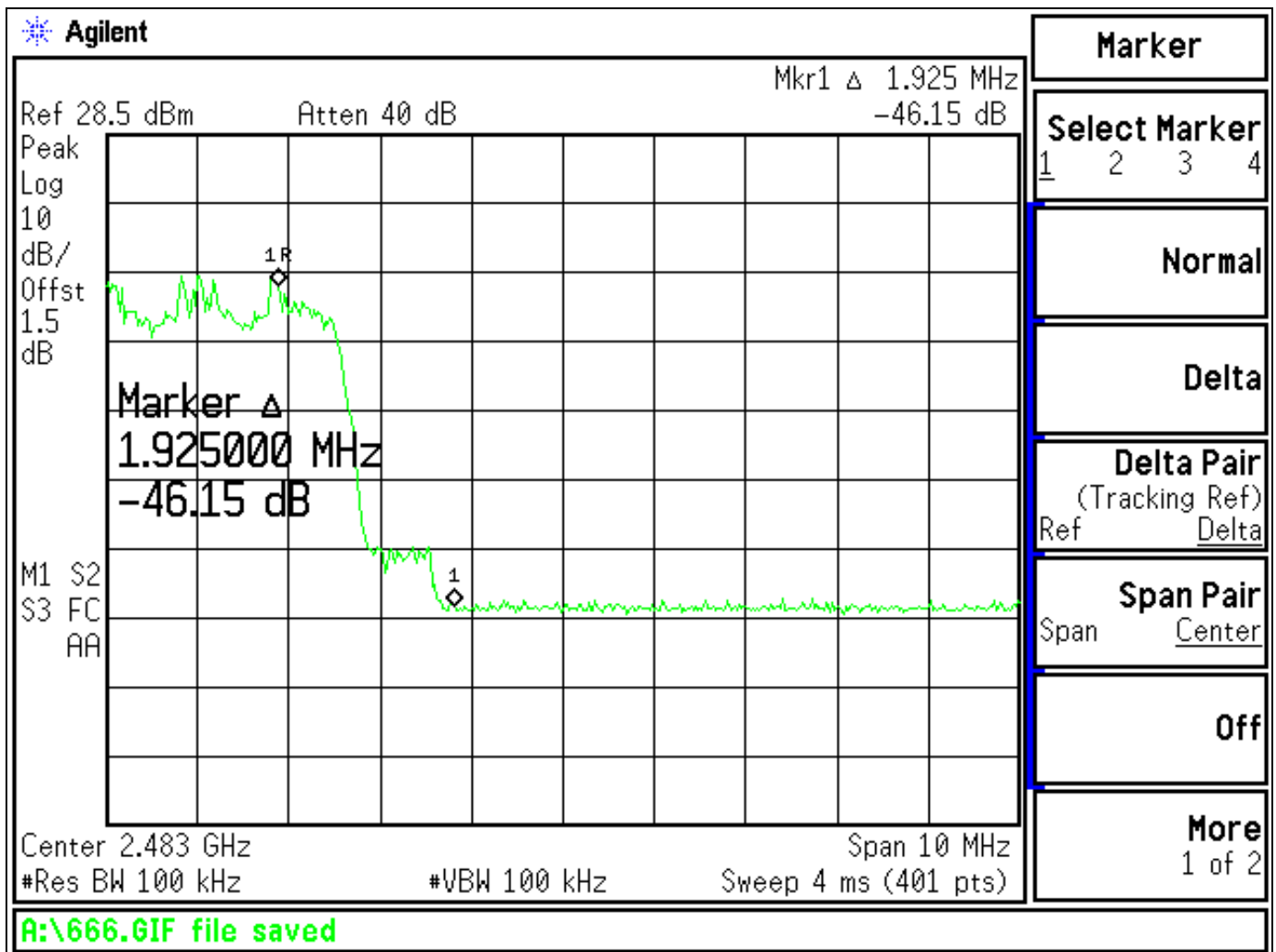
Figure 6d.6-8: Plot of upper band-edge conducted emissions with hopping enabled (Pi/4 DPSK Modulation).
