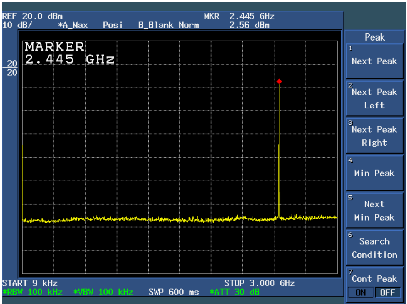
Figure 6d.7-4: Plot of spurious conducted emissions 9 kHz – 3.0 GHz (Mid Channel Enabled).
