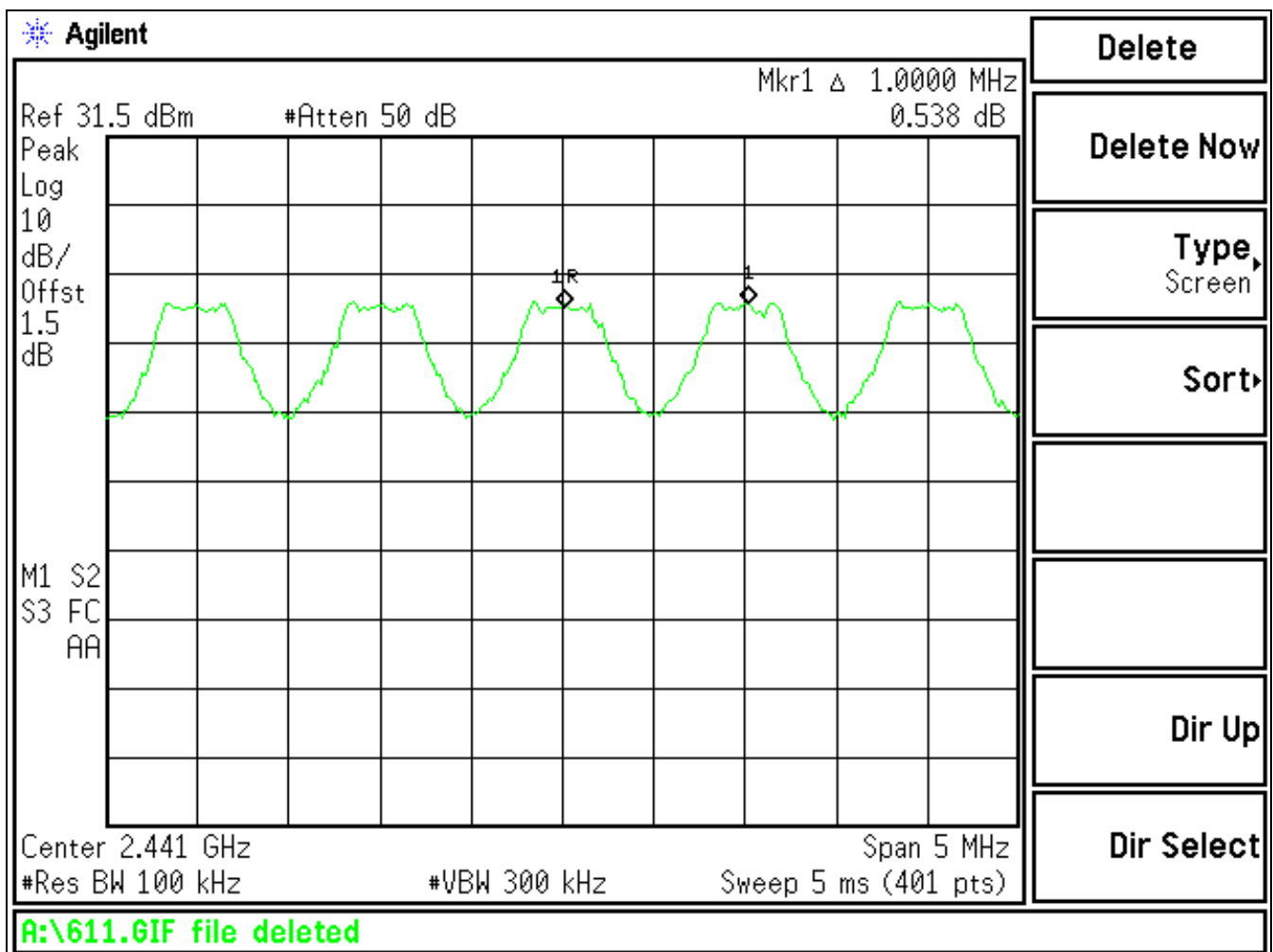
Figure 6d.1-1: Plot of Bluetooth carrier frequency separation
