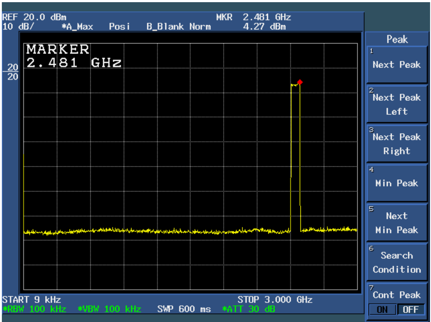
Figure 6d.7-10: Plot of spurious conducted emissions 9 kHz – 3.0 GHz (Hopping Function Enabled).
