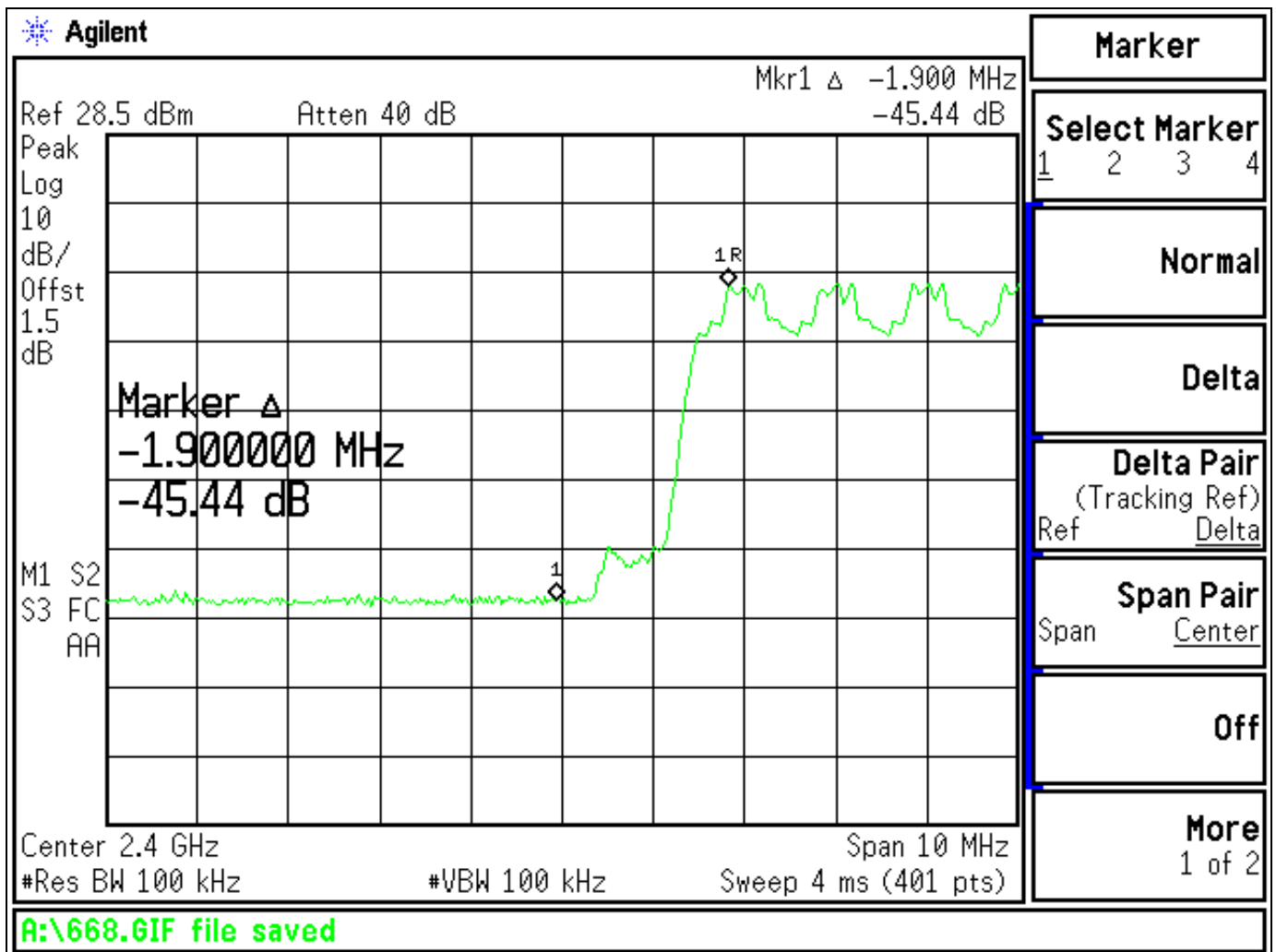
Figure 6d.6-7: Plot of lower band-edge conducted emissions with hopping enabled (Pi/4 DPSK Modulation).
