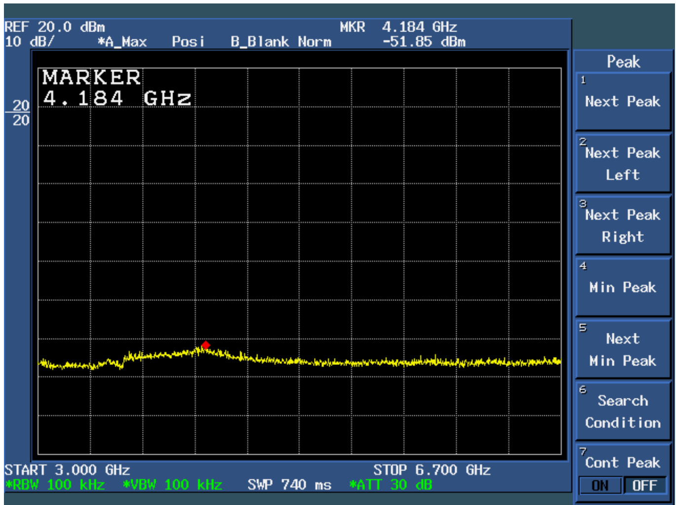
Figure 6d.7-11: Plot of spurious conducted emissions 3 GHz – 6.7 GHz (Hopping Function Channel Enabled).
