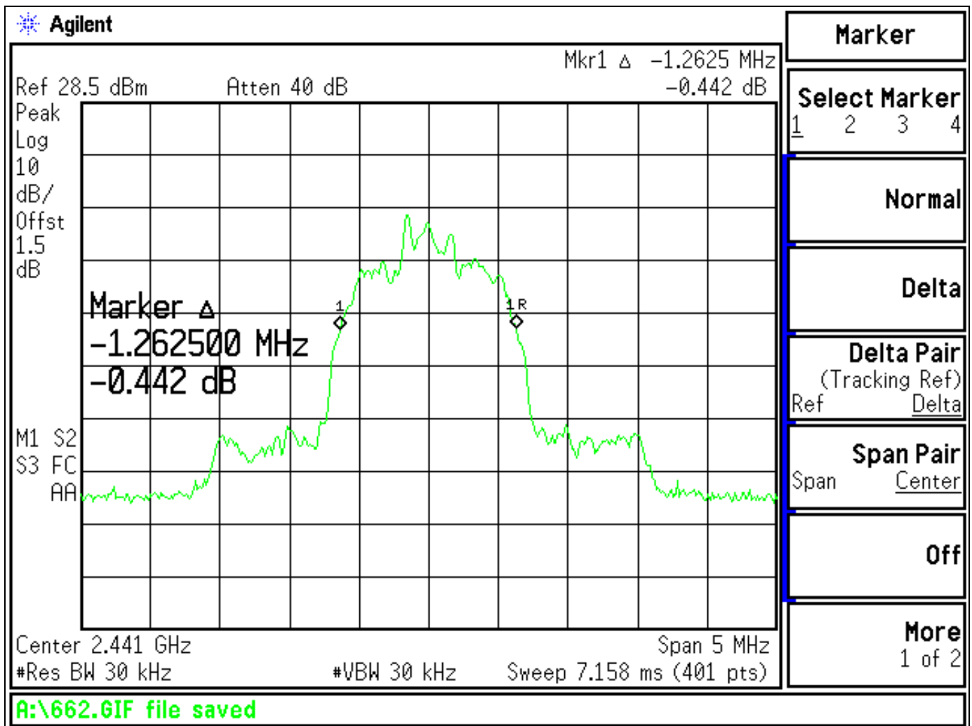
Figure 6d.2-2: Plot of 20 dB bandwidth (Pi/4 DPSK Modulation)
