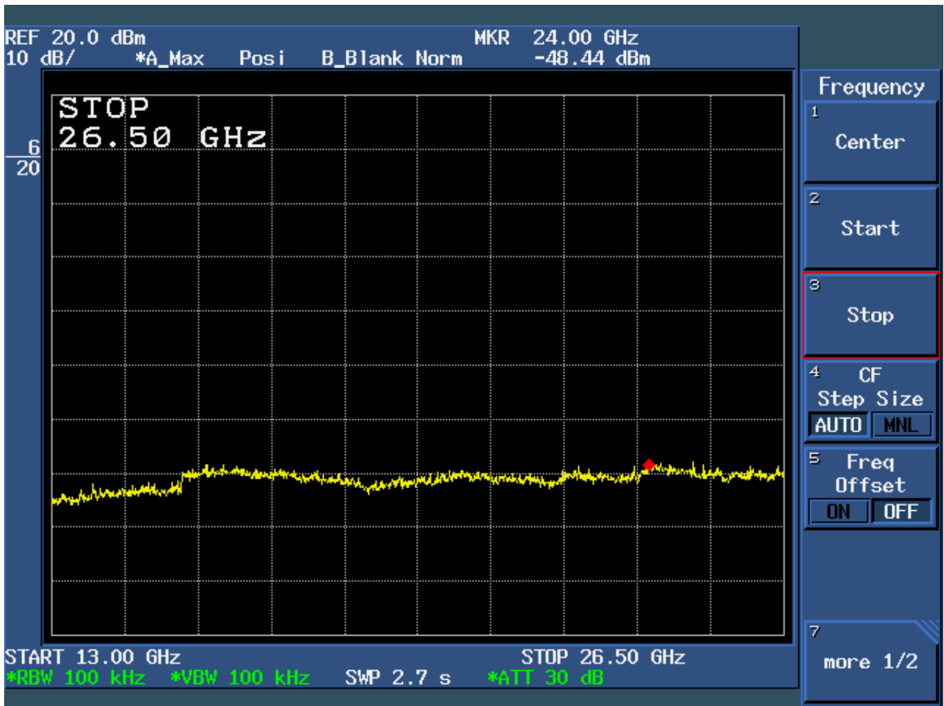
Figure 6d.7-6: Plot of spurious conducted emissions 13 GHz – 26.5 GHz (Mid Channel Enabled).
