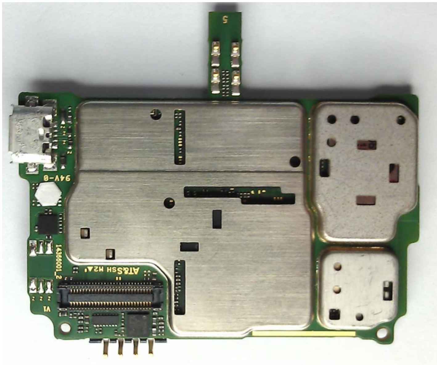
Photograph 9-1: Front side view of radio product PC Board, Shields in Place.
