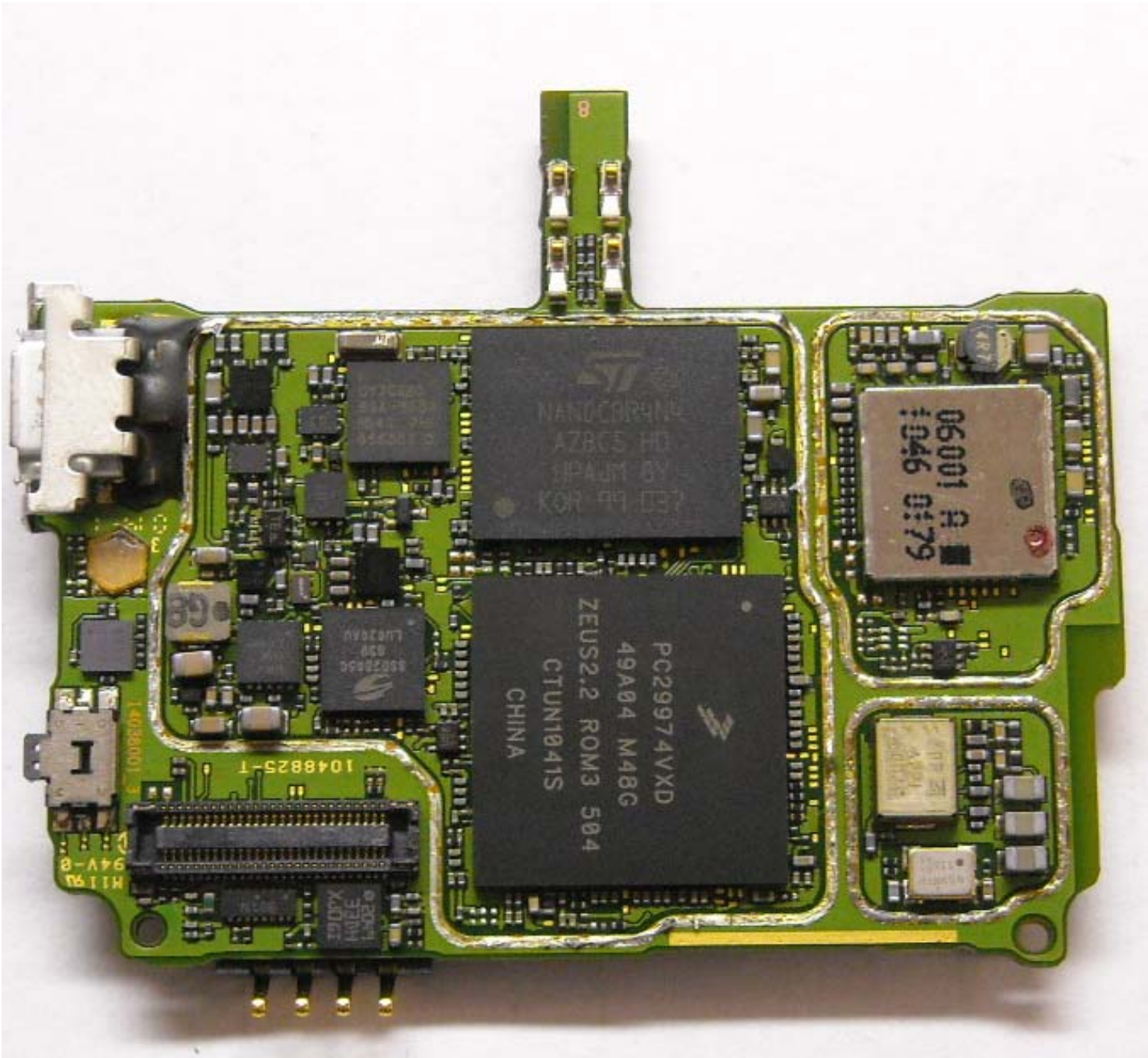
Photograph 9-2: Front side view of radio product PC Board, Shields Removed.
