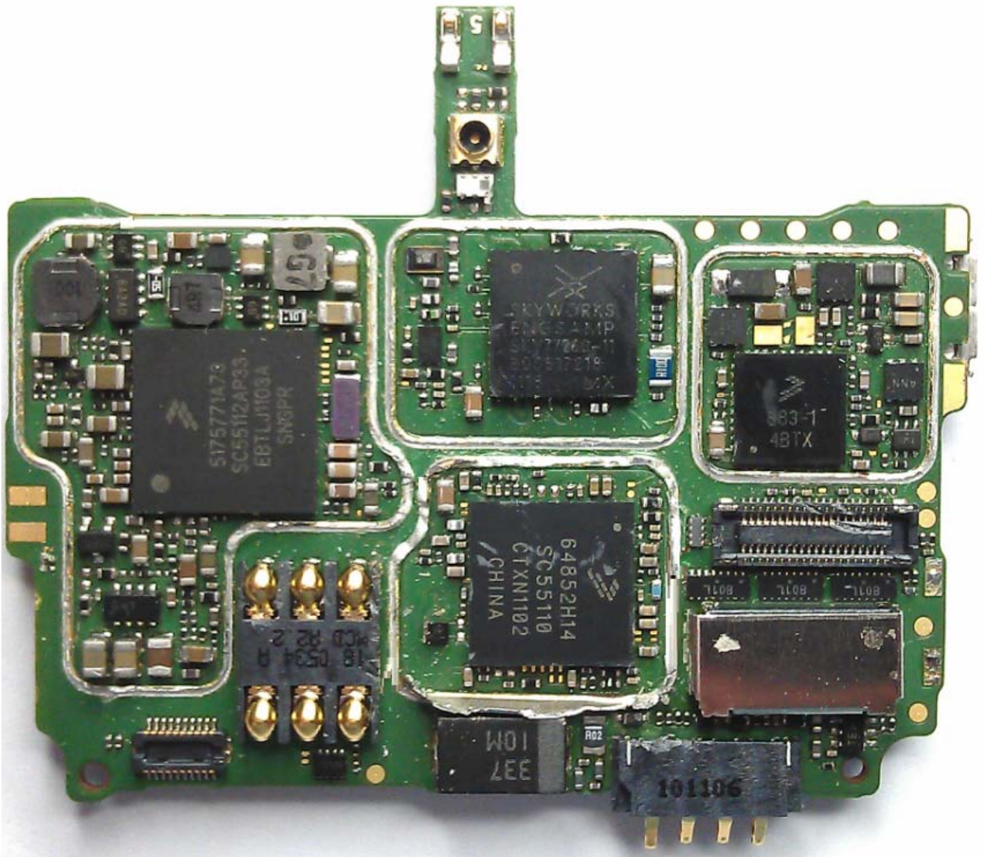
Photograph 9-4: Rear side view of radio product PB Board, Shields Removed.
