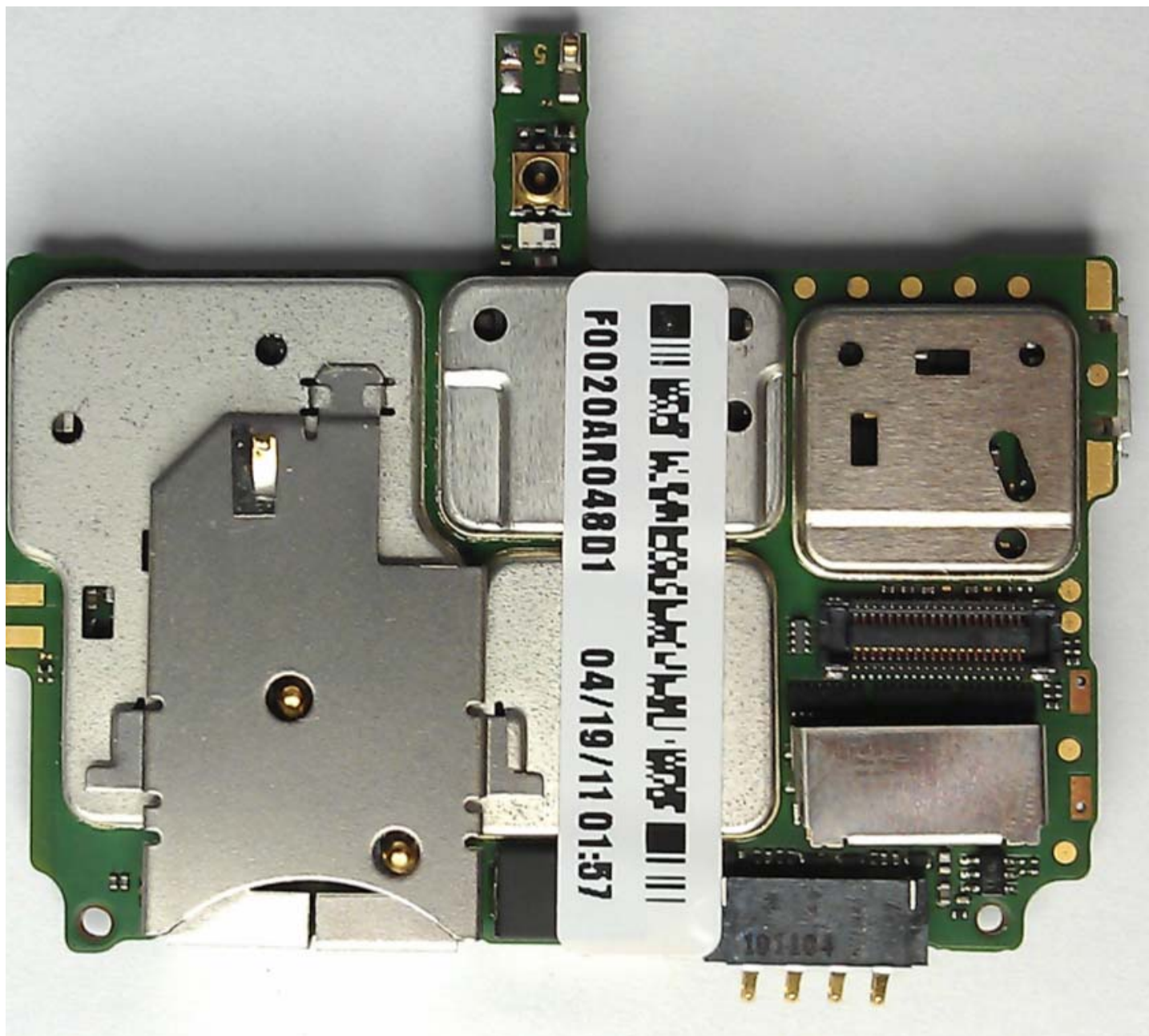
Photograph 9-3: Rear side view of radio product PB Board, Shields in Place.
