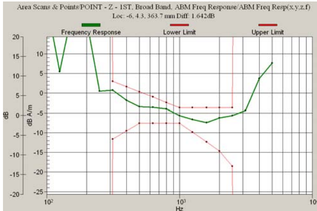
Figure 9-1-1: 800 MHz Measured Frequency Response (2:6).
