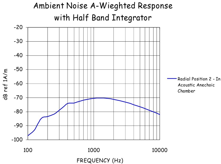
Figure 8-3 – Radial Position 2 Ambient Magnetic frequency distribution
