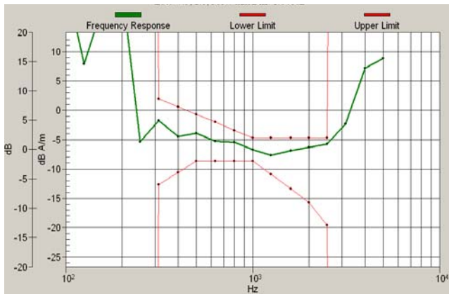
Figure 9-1-3: 900 MHz Measured Frequency Response (2:6).
