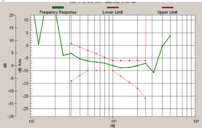
Figure 9-1-4: 900 MHz Measured Frequency Response (1:6).
