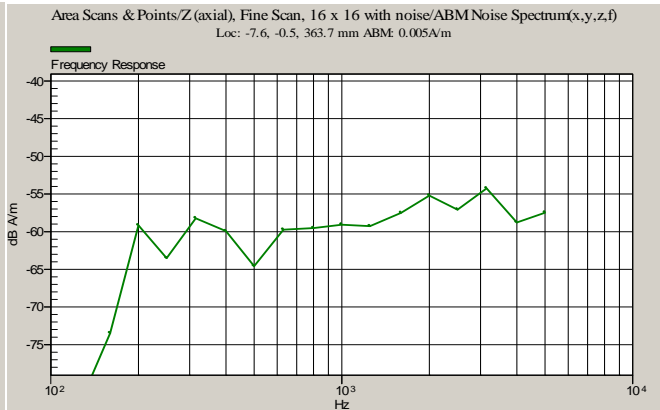
Figure 9-2-2: 800 MHz ABM2 Undesired Signal (1:6).
