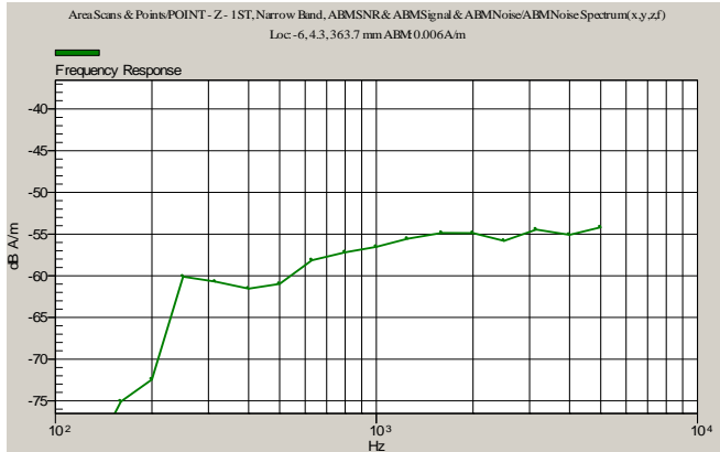
Figure 9-2-1: 800 MHz ABM2 Undesired Signal (2:6).
