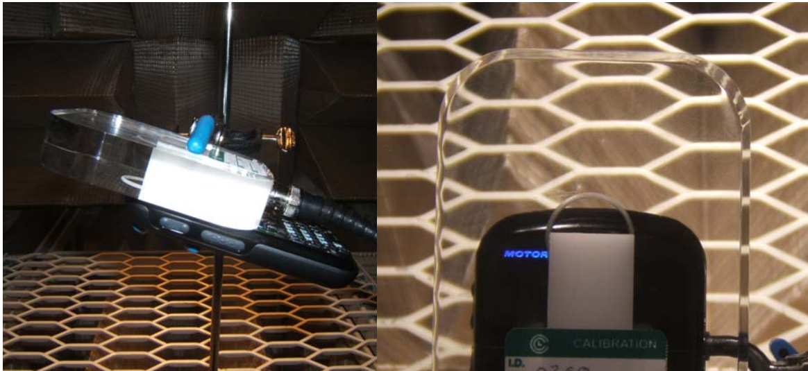
Figure 7-1 – Test holder
