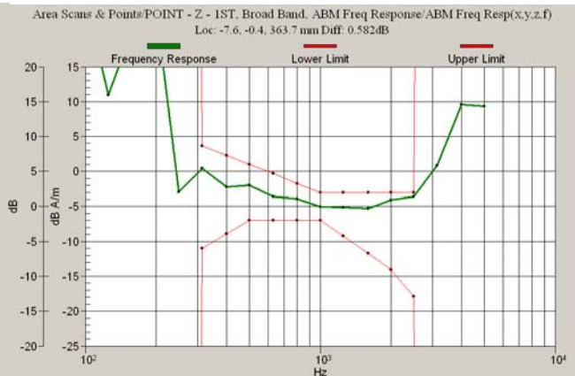
Figure 9-1-2: 800 MHz Measured Frequency Response (1:6).
