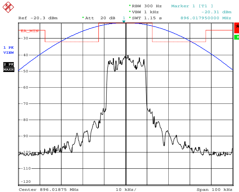
Figure 6a.2.2-11. iDEN 900 MHz Band, Quad-64QAM, Maximum Power, EA Emission Mask
