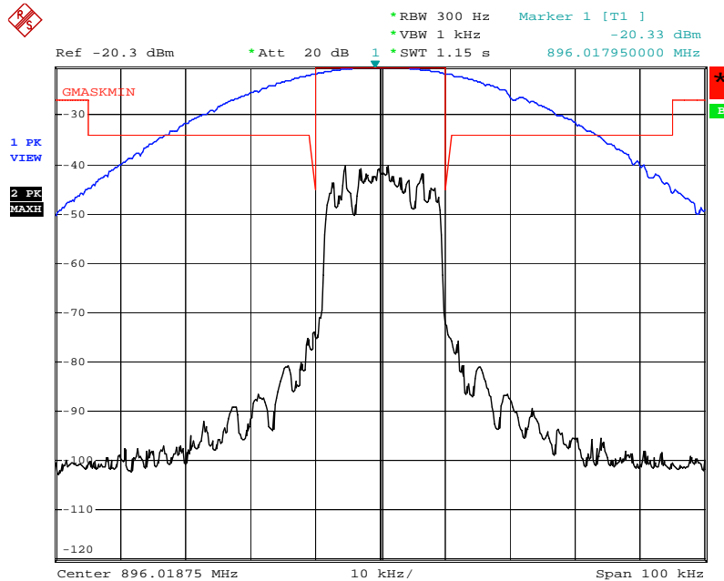
Figure 6a.2.2-5. iDEN 900 MHz Band, Quad-16QAM, Maximum Power, Emission Mask G
