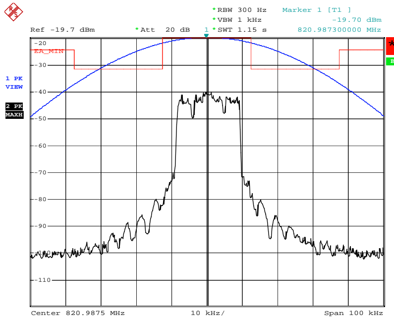
Figure 6a.2.1-7. iDEN 800 MHz Band, Quad-16QAM, Maximum Power, EA Emission Mask
