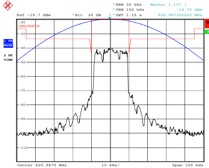
Figure 6a.2.1-1. iDEN 800 MHz Band, Quad-QPSK, Maximum Power, Emission Mask G
