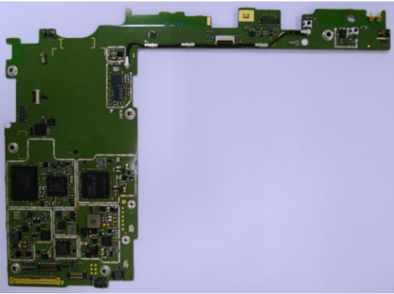
Main Board Bottom Without Shields
