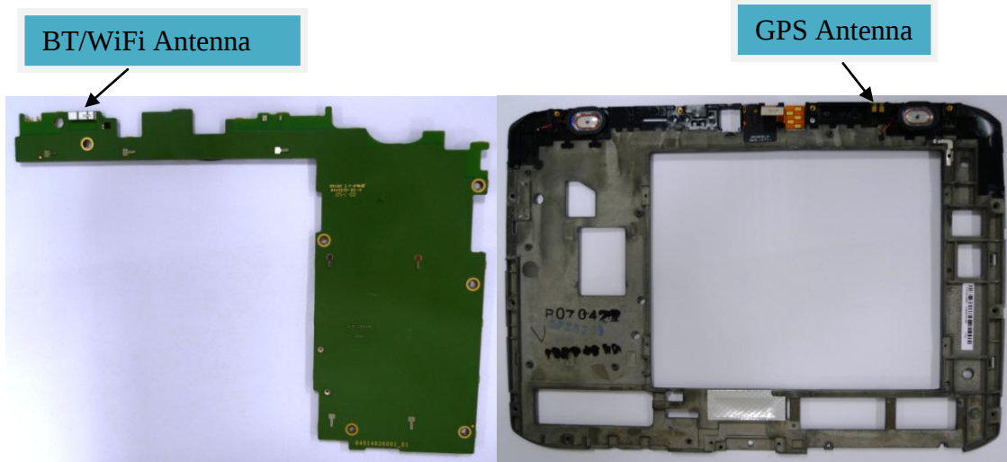
GPS and BT/WiFi Antenna Location
