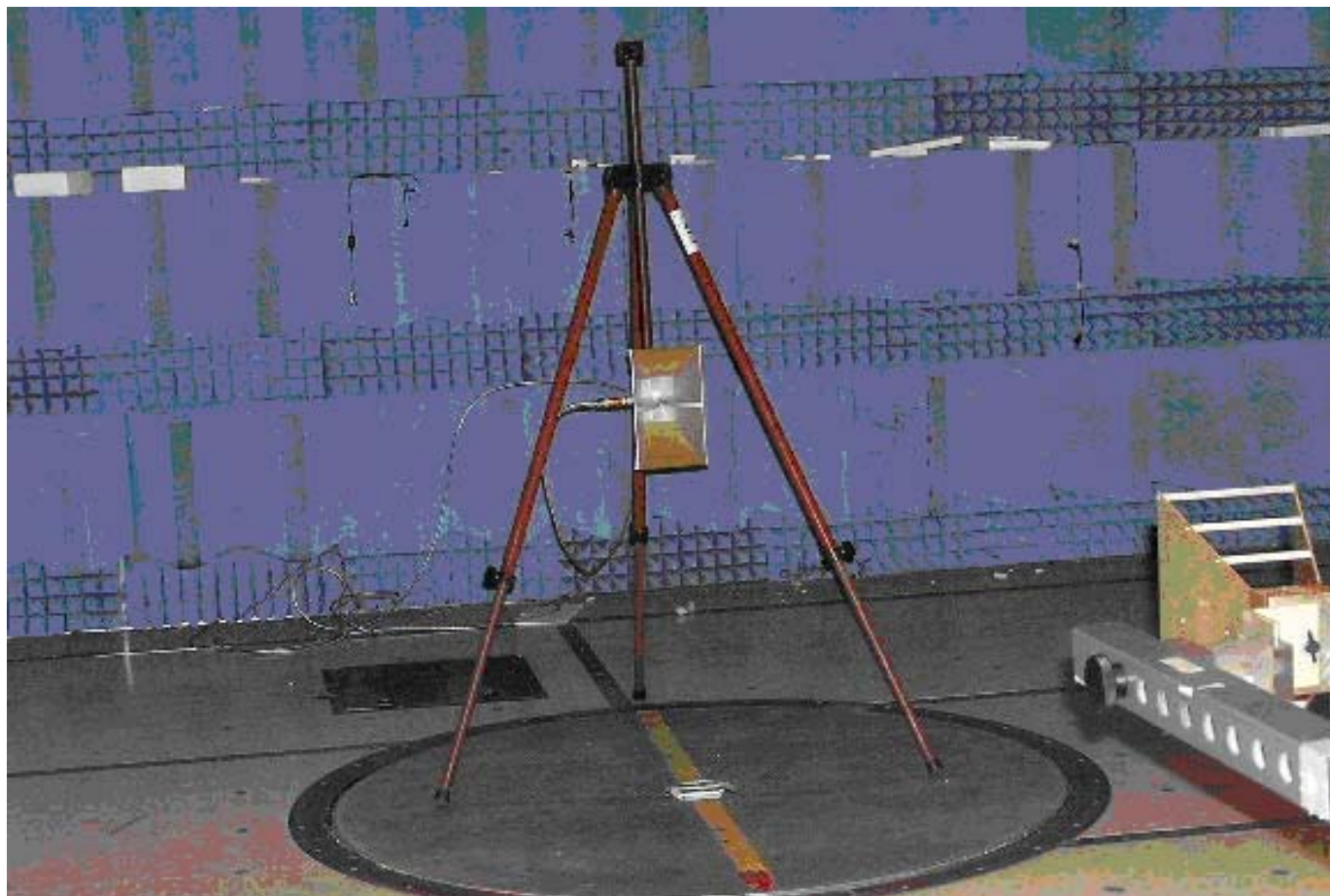
Figure 7c1-3: Antenna - Substitution.
