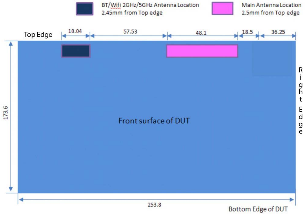
Figure 3: Device Dimensions and Antenna Separation Distances
