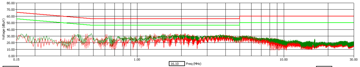
WLAN Channel 6 - Tx Mode - AVG Detector
