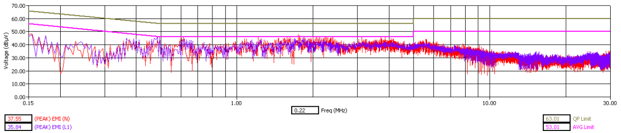
WLAN Channel 6 - Tx Mode - Peak Detector
