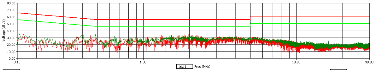
WLAN Channel 11 - Tx Mode - AVG Detector
