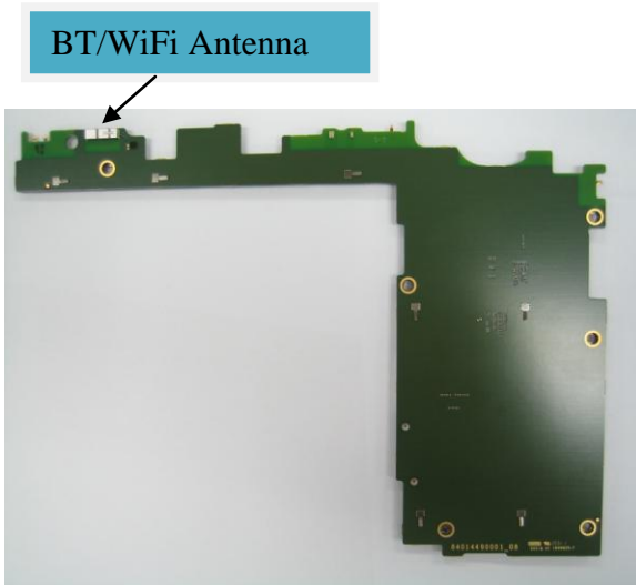
Main, Diversity, GPS and BT/WiFi Antenna Location
