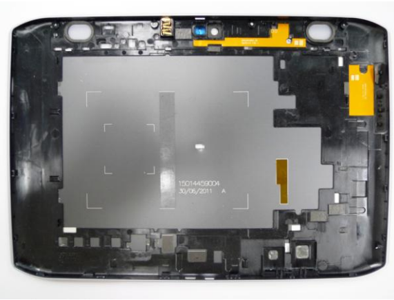
Rear Housing
