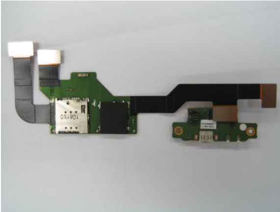
SIM Flex and IO PCB Bottom
