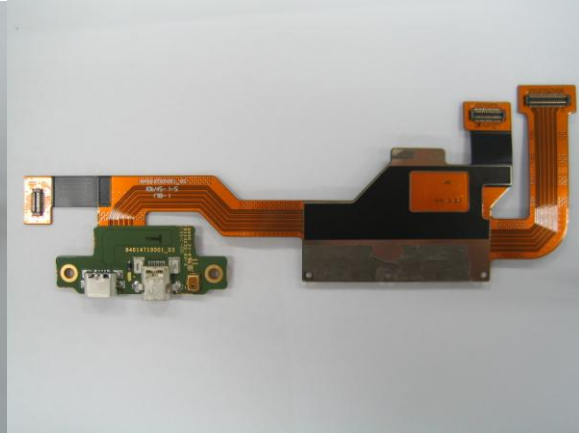
SIM Flex and IO PCB Top
