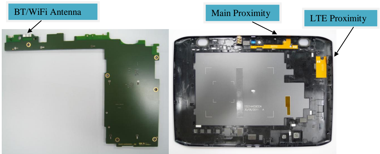
Main, Diversity, GPS and BT/WiFi Antenna and Proximity Sensor Location
