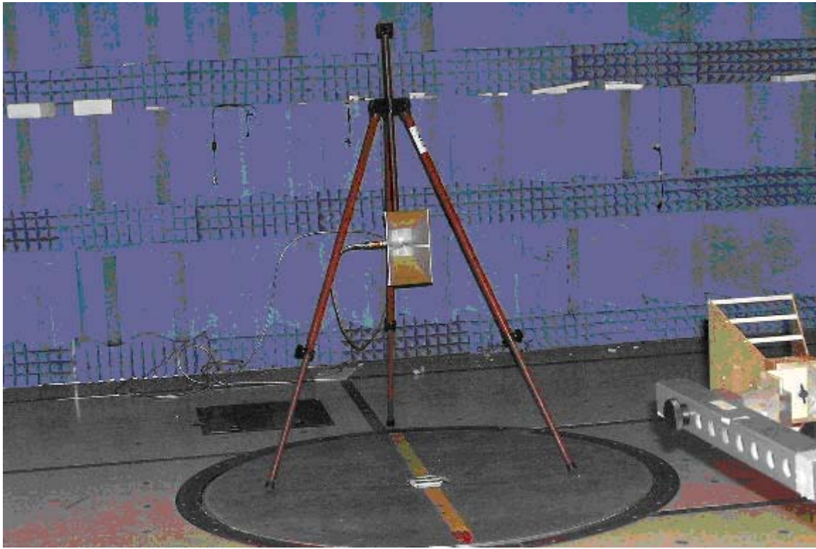
Antenna - Substitution
