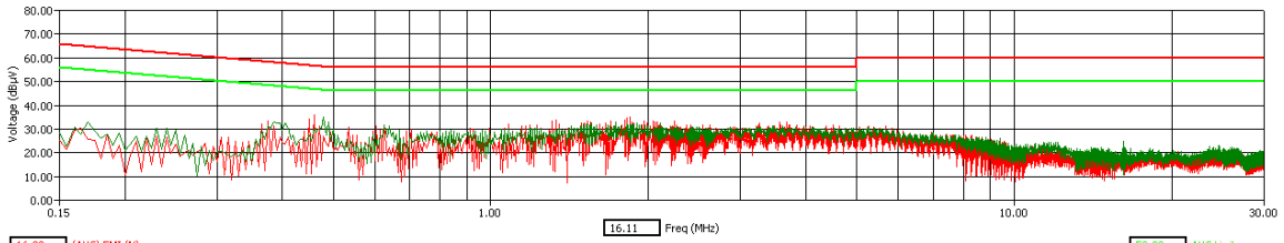
WLAN Channel 161 - Tx Mode - AVG Detector
