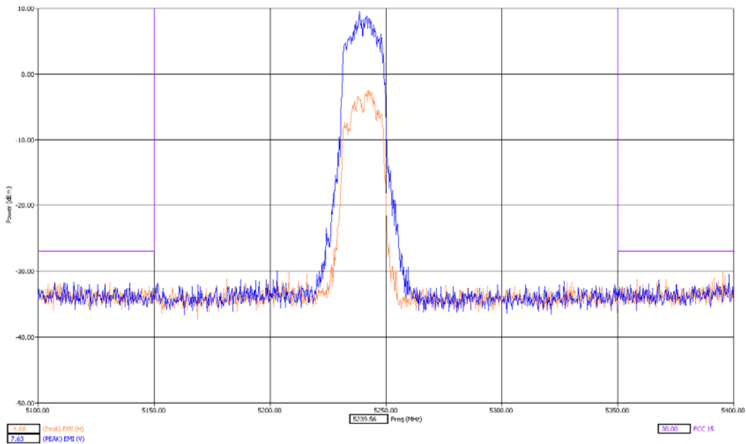
High Band Edge Z Orientation Peak Detector
