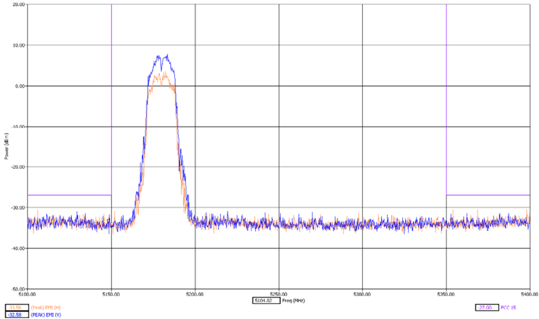
Low Band Edge Z Orientation Peak Detector
