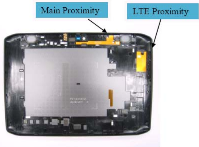
Main, LTE, Diversity, GPS, BT/WiFi Antenna and Cap proximity sensor Location
