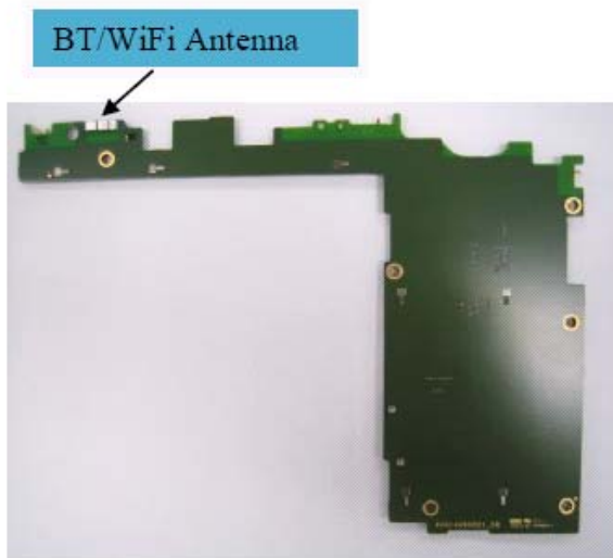
Main, LTE, Diversity, GPS, BT/WiFi Antenna and Cap proximity sensor Location
