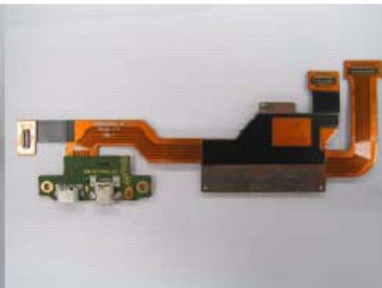
SIM Flex and IO PCB Top
