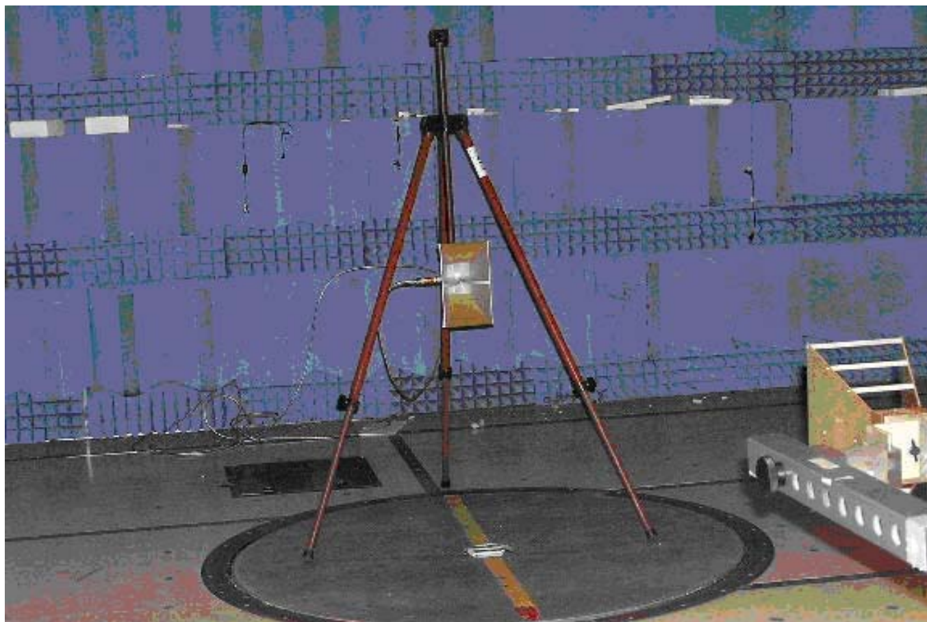
Figure 3: Antenna Substitution.
