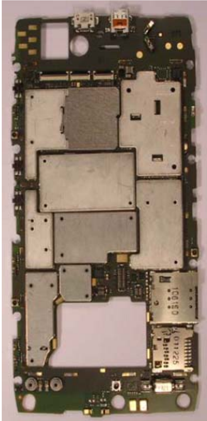
Photograph 9-1: Front side view of the device's PC Board, Shields in place.
