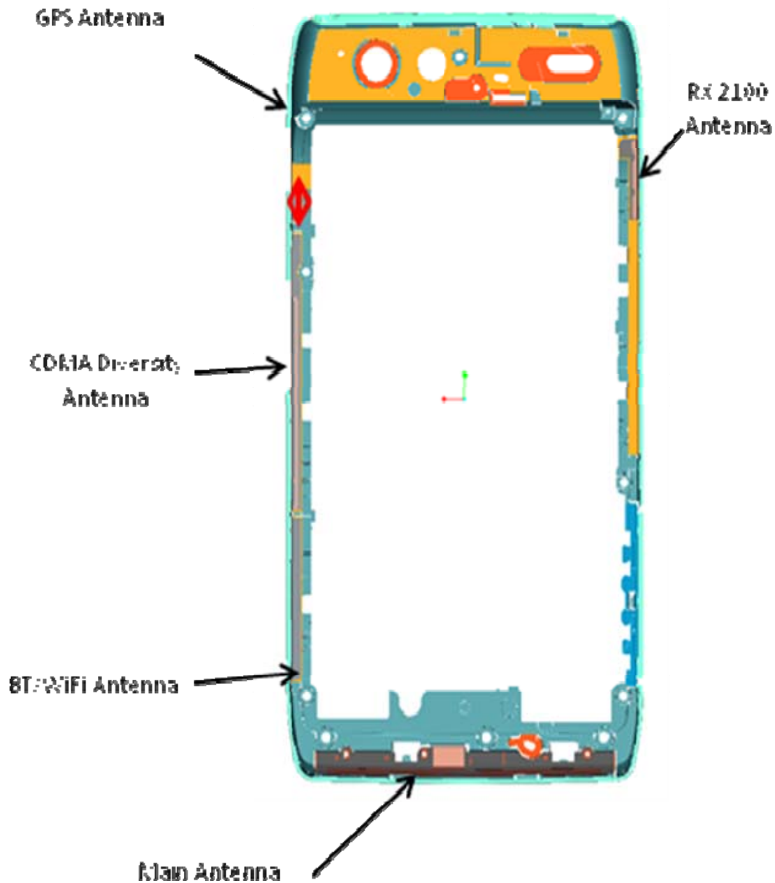
Photograph 9-5: Schematic, showing physical locations of all Antennas.
