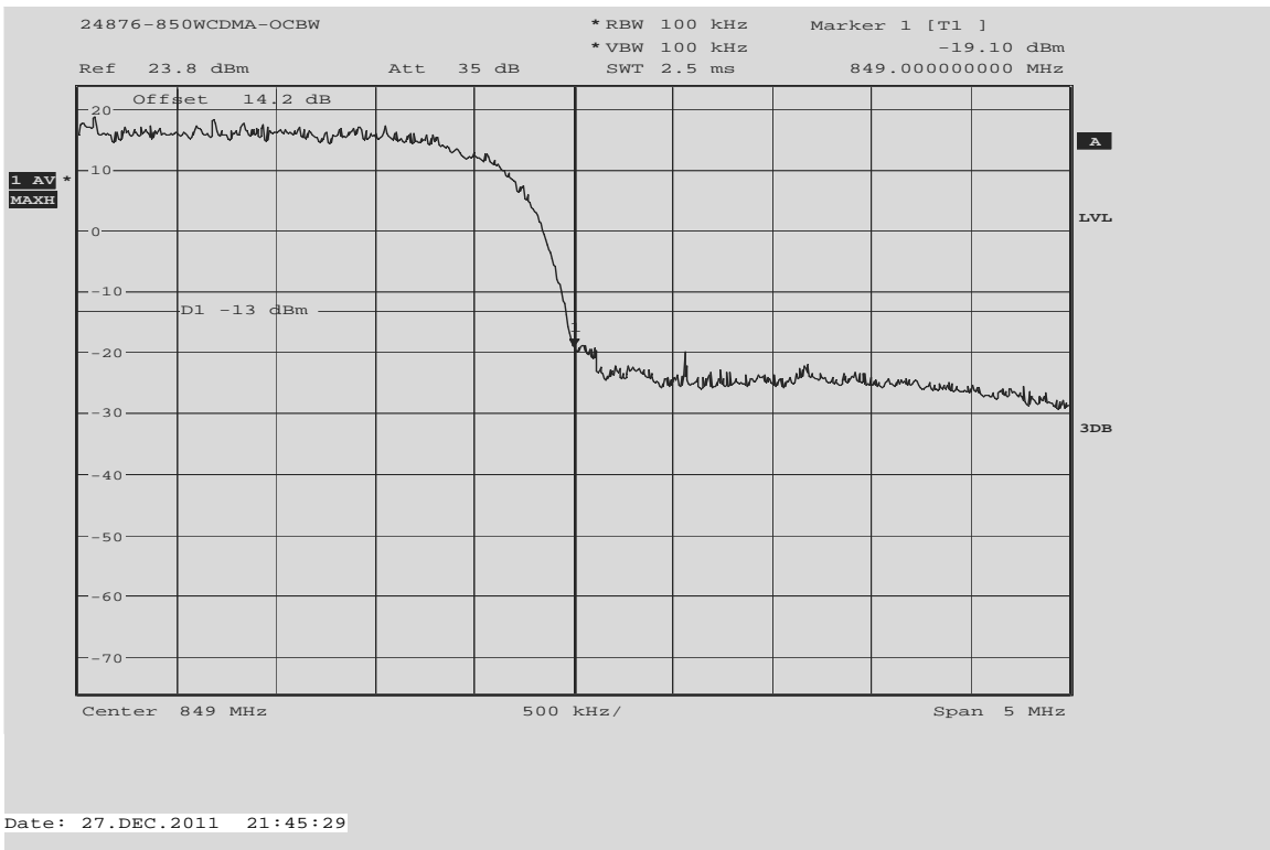
WCDMA 850 – Upper Band Edge – Channel 4233 (848.6 MHz)
