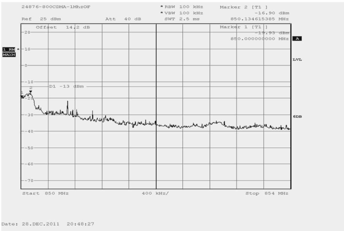
800 CDMA Conducted Spurious Emissions (Upper adjacent 1 MHz band)
