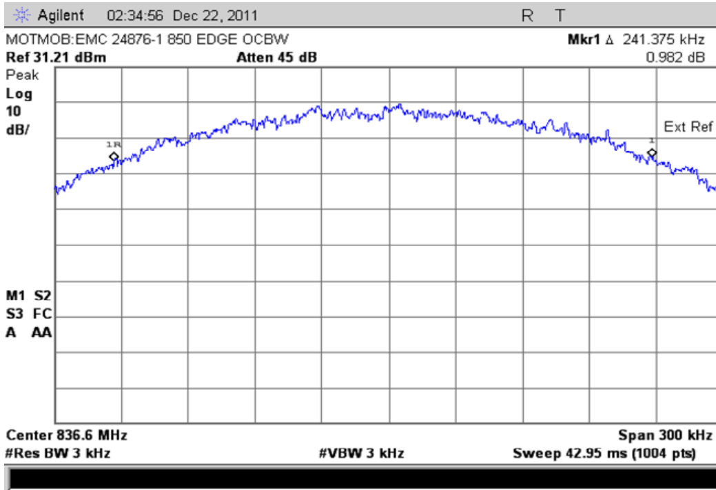
EDGE 850 – Channel 190 (836.60 MHz) – Occupied Bandwidth
