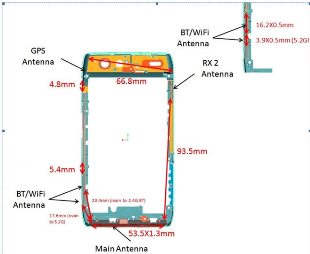
Figure 2: Antenna Separation Distances
