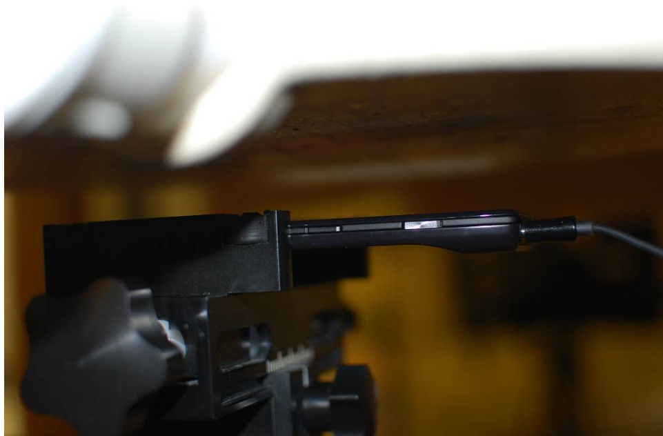
SAR Test Setup Photo 6- Body-Worn Front at 2.5 cm
