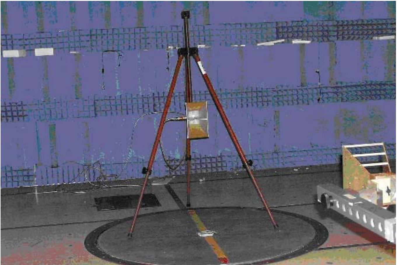
Figure 3: Antenna Substitution.
