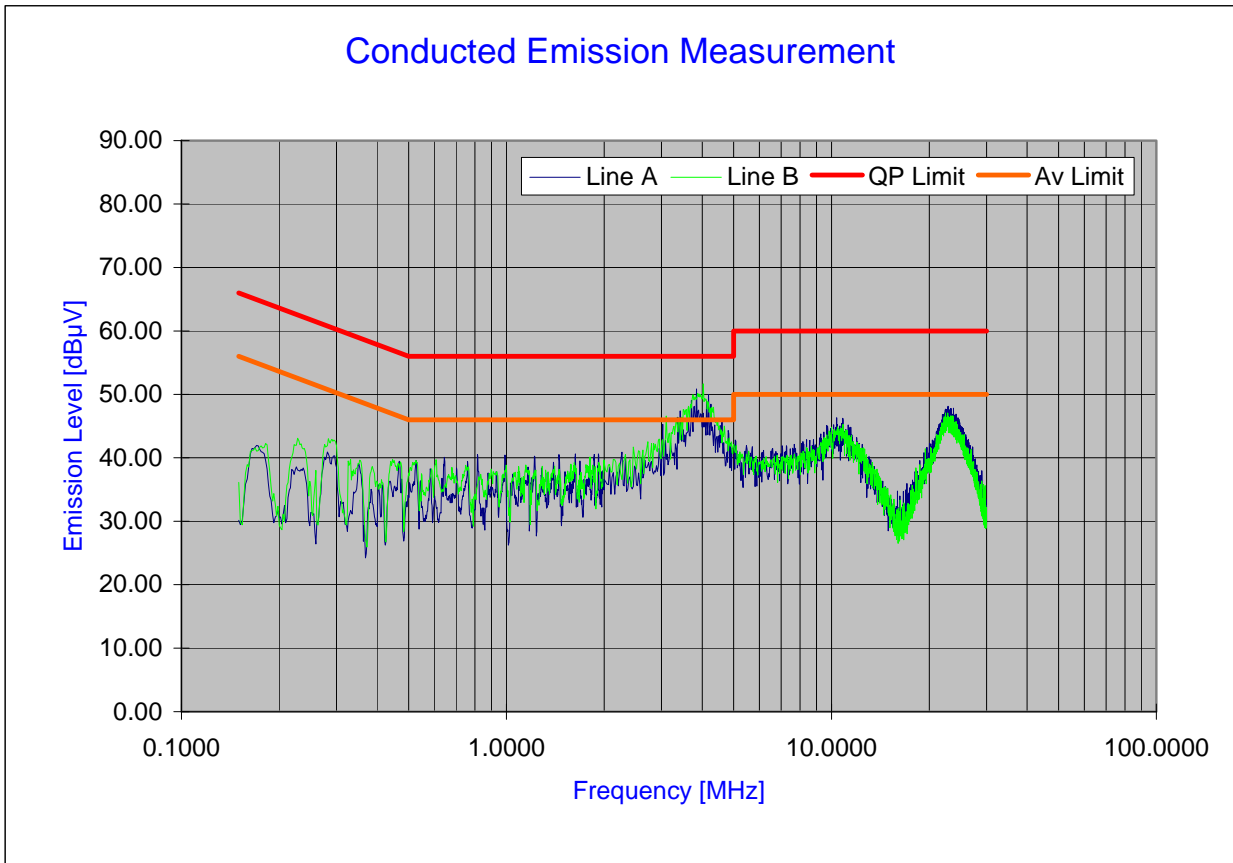
Plot 6-58. Line Conducted Plot with 802.11n (2.4GHz)
