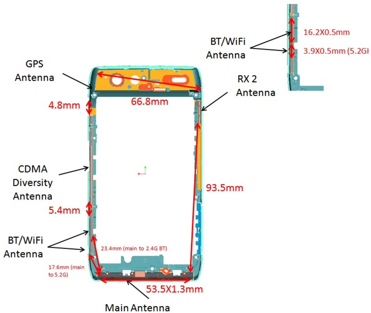
Figure 2: Antenna Separation Distances
