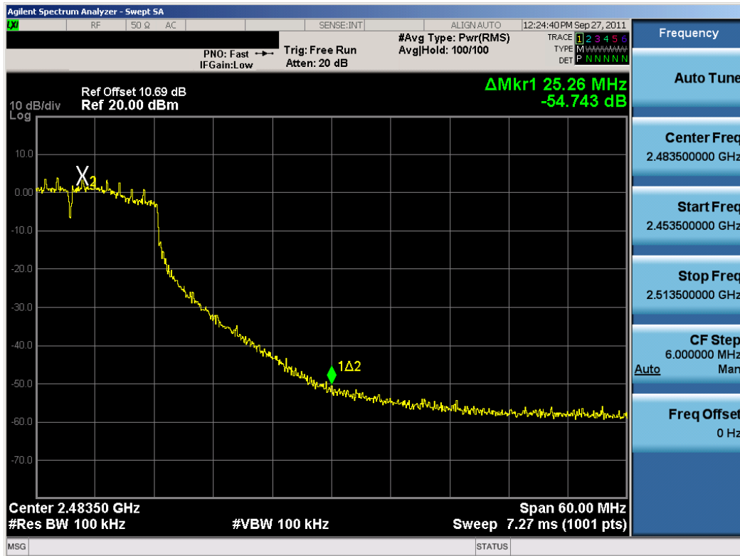
Plot 6-39. Band Edge Plot (802.11n (2.4GHz) – Ch. 10)
