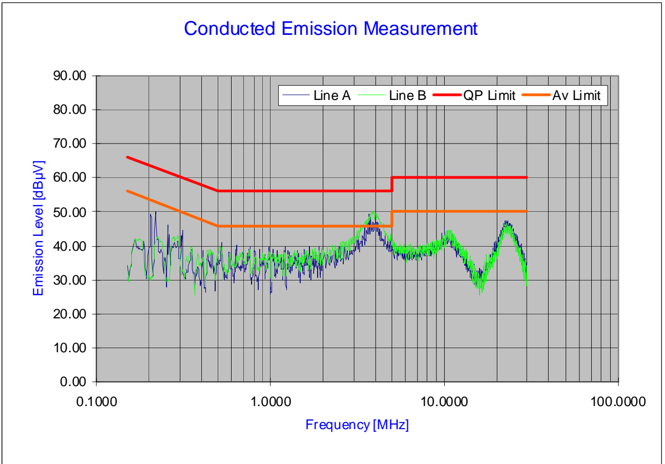
Plot 6-61. Line Conducted Plot with 802.11g
