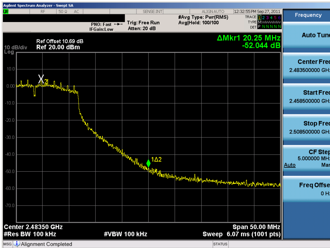
Plot 6-37. Band Edge Plot (802.11g – Ch. 11)
