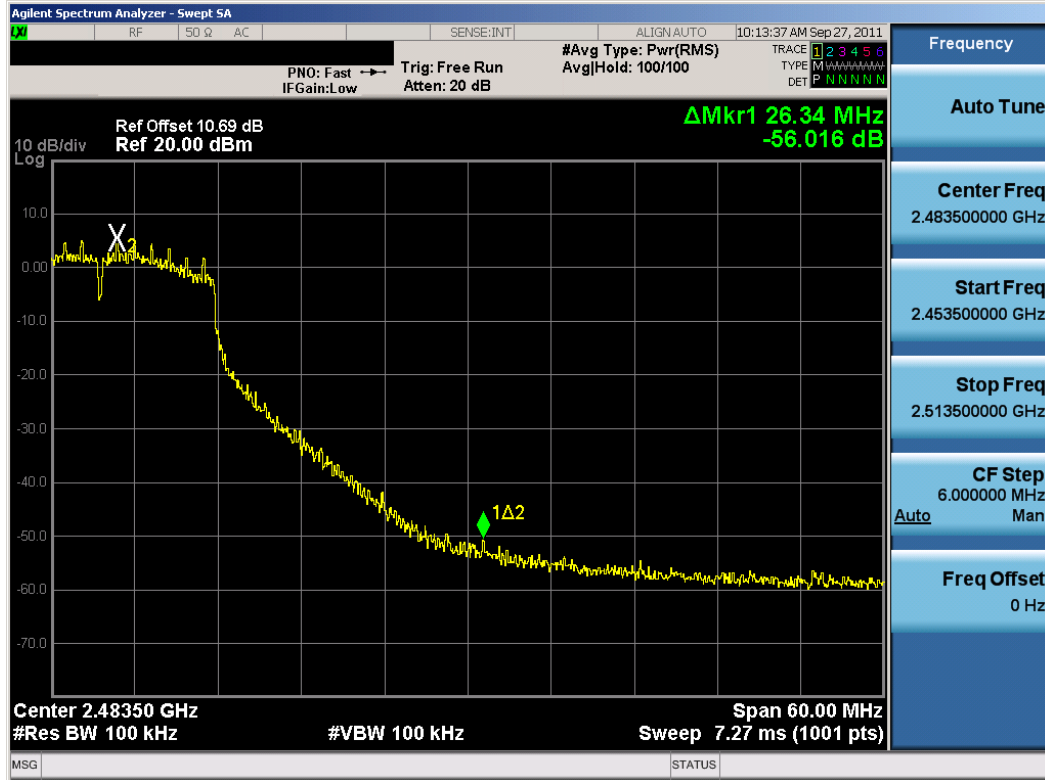
Plot 6-36. Band Edge Plot (802.11g– Ch. 10)
