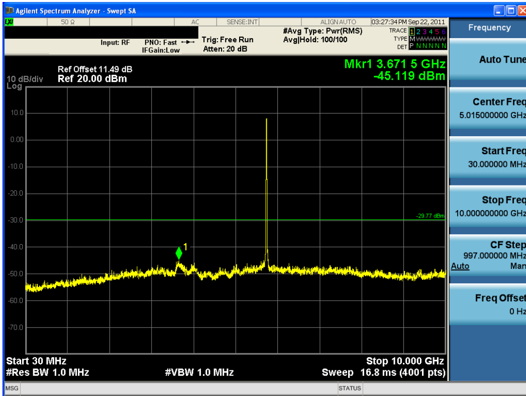
Plot 6-51. Conducted Spurious Plot (802.11a – Ch. 149)
