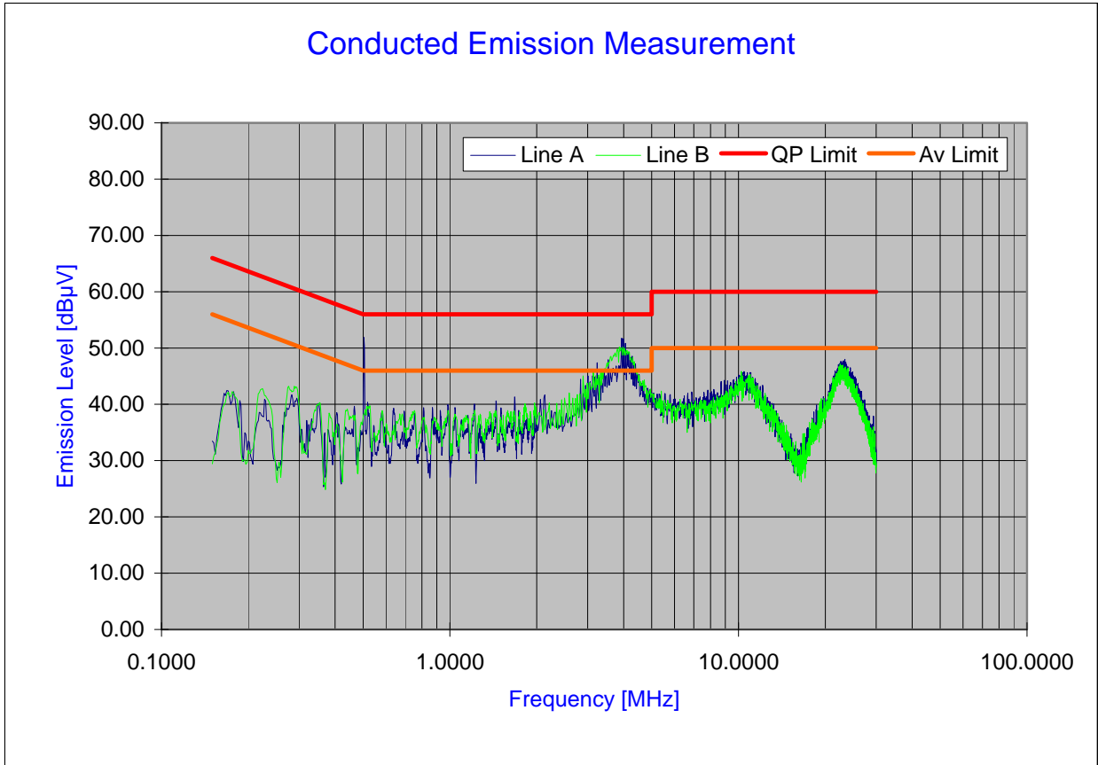
Plot 6-60. Line Conducted Plot with 802.11b
