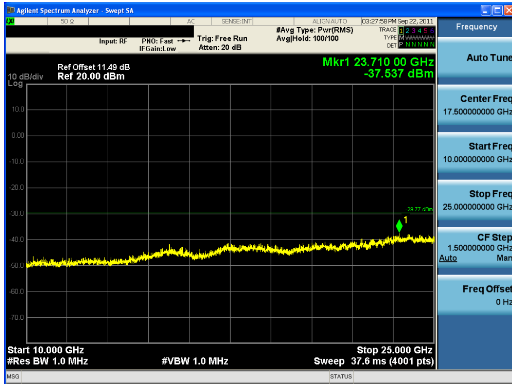
Plot 6-52. Conducted Spurious Plot (802.11a – Ch. 149)
