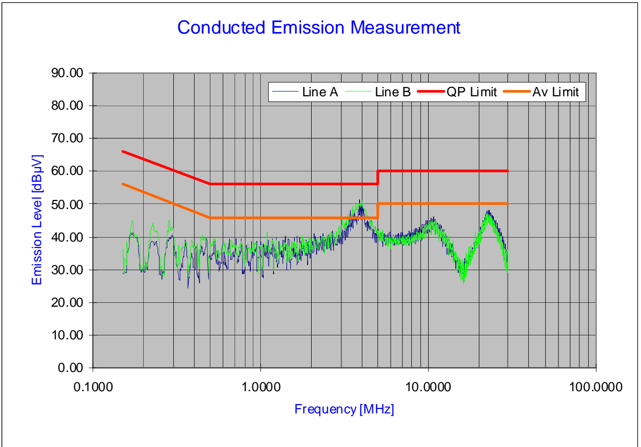
Plot 6-63. Line Conducted Plot with 802.11a
