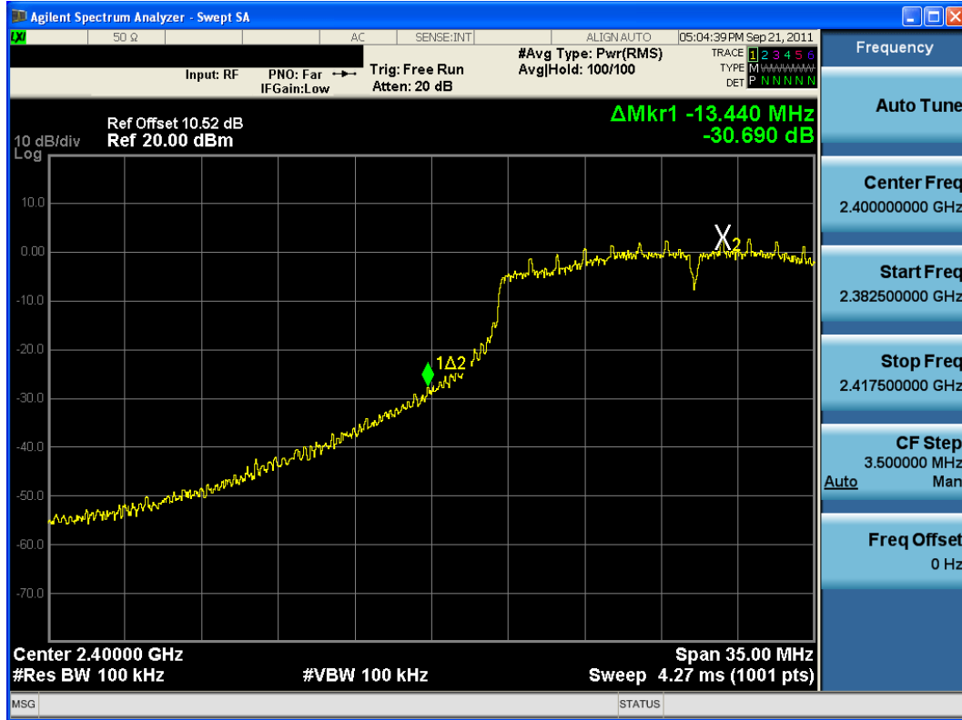
Plot 6-38. Band Edge Plot (802.11n (2.4GHz) – Ch. 1)
