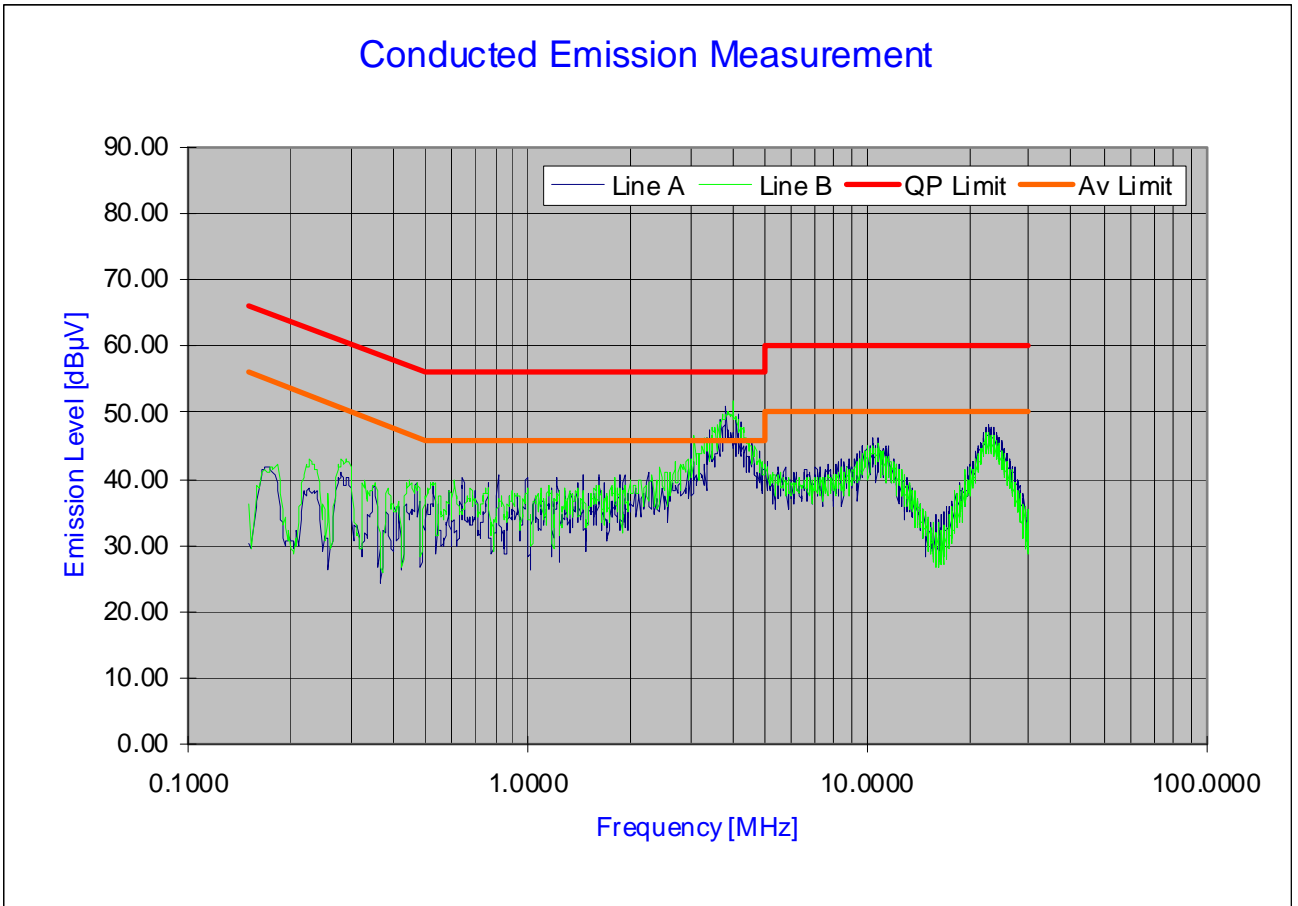
Plot 6-62. Line Conducted Plot with 802.11n (2.4GHz)
