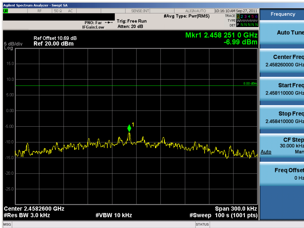
Plot 6-21. Power Spectral Density Plot (802.11g – Ch. 10)
