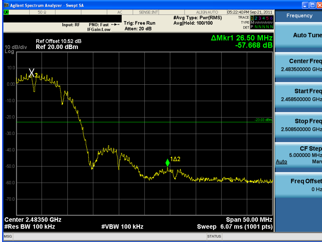
Plot 6-34. Band Edge Plot (802.11b – Ch. 11)
