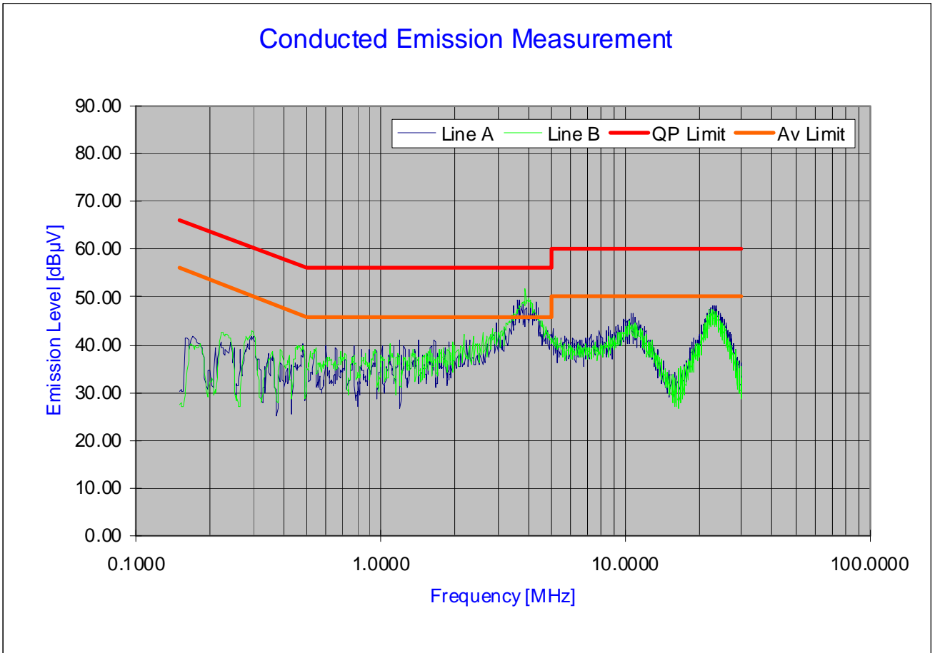
Plot 6-64. Line Conducted Plot with 802.11n (5.8GHz)
